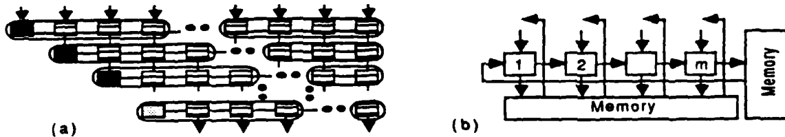
Figure 5: Partitioned linear array for the Faddeev algorithm
