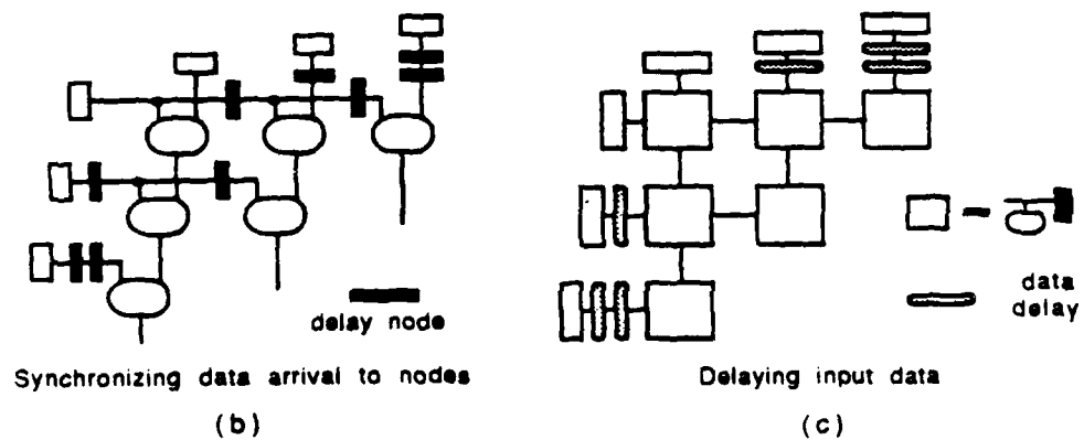
Figure 3: Removing data broadcasting
