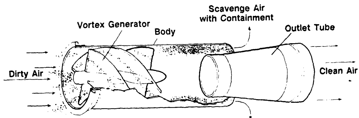
Figure B-17. Vortex Generator Tube
