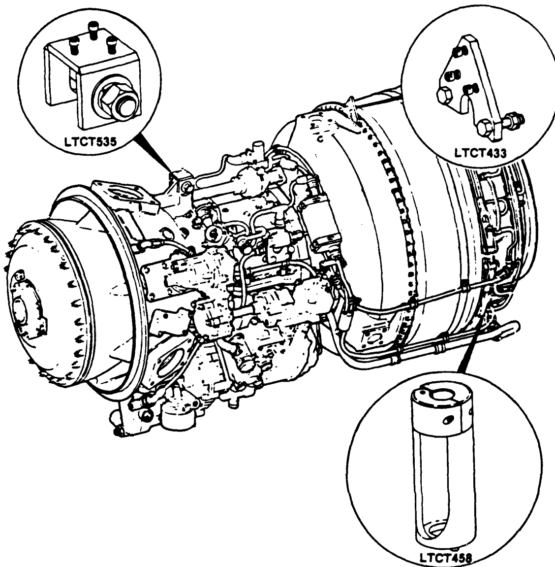
Figure C-3. Engine Accelerometer Locations
