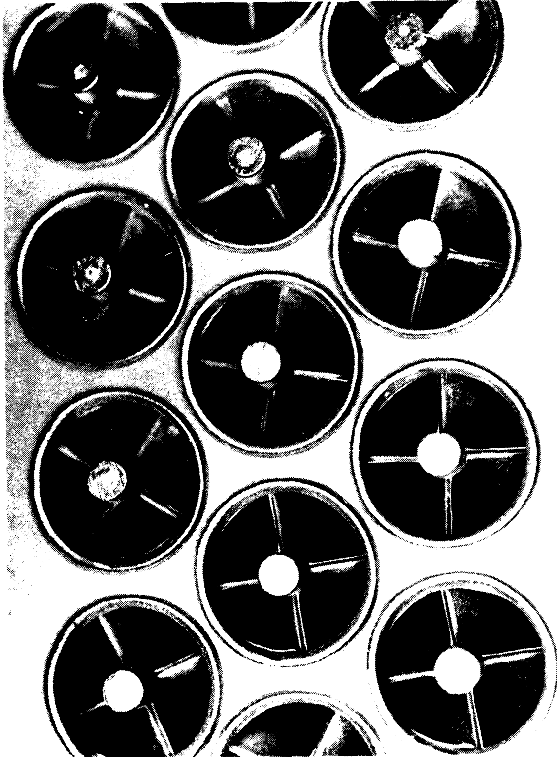
Figure B-18. Vortex Generator Tubes Installed in IEAFS. View from Outside of IEAFS Showing Upstream Ends of Tubes
