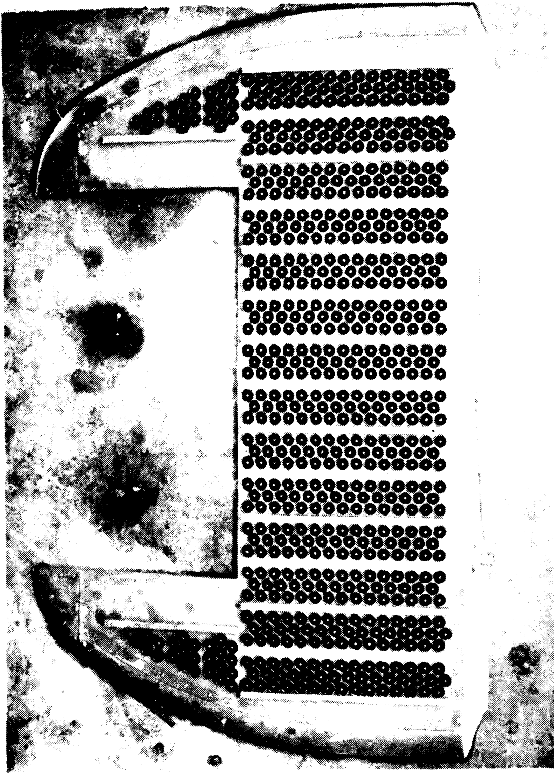
Figure B-15. IEAFS Upper Half with Screen Removed-Vertical View Looking Down
