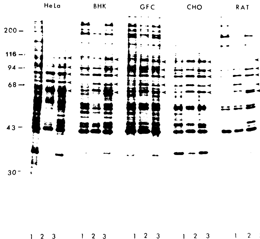
Fig. 1. Patterns of stress protein synthesis in five different mammalian cell lines. HeLa, baby hamster kidney (BHK) cells, gerbil fibroma (GFC) cells, Chinese hamster ovary (CHO) cells, and rat-1 (RAT) cells were pulse-labeled with [ ^{35} S]-methionine after a 5 hour incubation at 37°C (lanes 1), at 37°C in the presence of 5mM Azc, an amino acid analog of proline (lanes 2) or at 42°C (lanes 3). The cells were solubilized and the labeled proteins analyzed on a 10% polyacrylamide gel. Shown is an autoradiograph of the gel. Molecular mass markers are indicated at the left and the stress proteins indicated at the right (in descending order: 110, 100, 90, 80, 73/72 kDa proteins).
