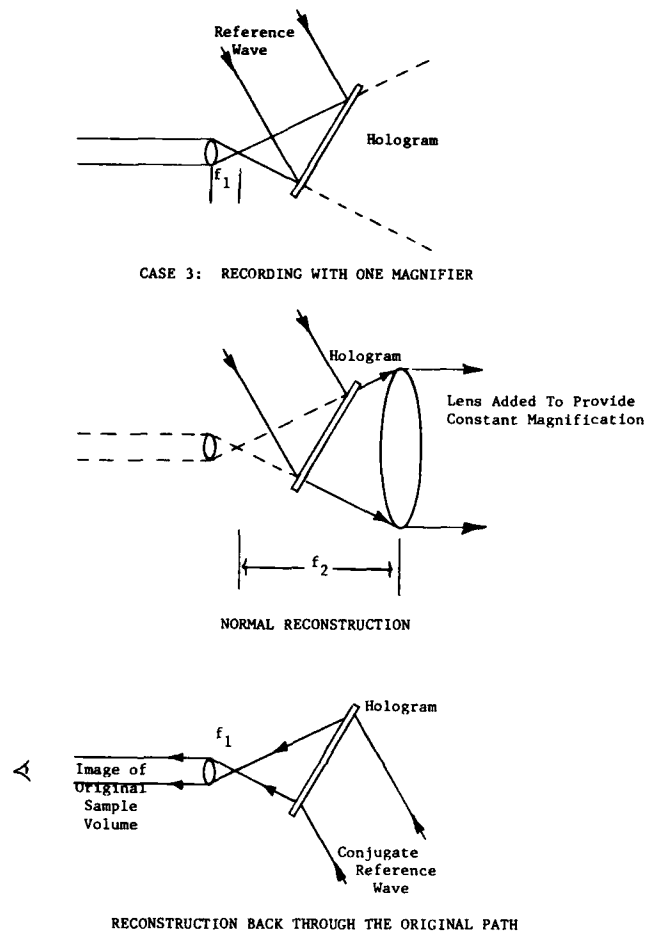
Figure 3.14 Holography with Premagnification.
