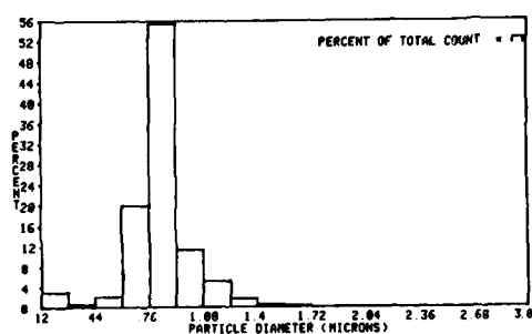
Figure 4.33m DOP without dilution flow in the vaporization/condensation seeder.
