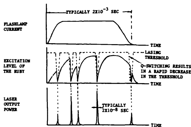
Figure 1.27 Multiple Q-switching a ruby laser
