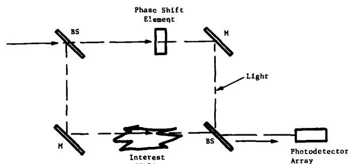
Figure 2.23a Subfringe interferometer
