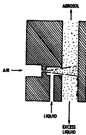
Figure 4.33c Collision nebulizer
