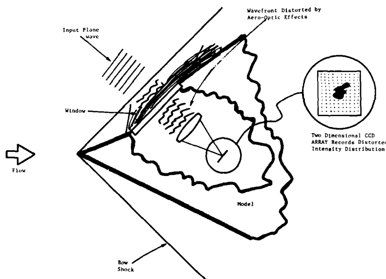
Figure 2.5 Conceptual experiment for measuring aero-optic effects. The incoming wave from is distorted by the flow field, limiting the attainable resolution of an imaging system in the vehicle.
