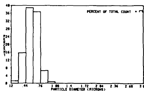
Figure 33n DOP with dilution nitrogen in the vaporization/condensation feeder.
