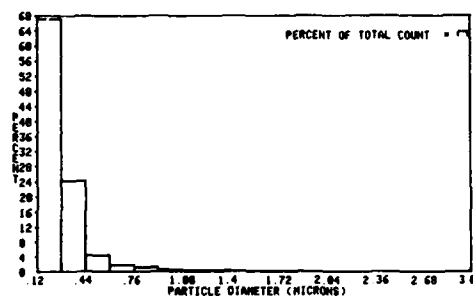
Figure 4.33l DOP in the Collision nebulizer.
