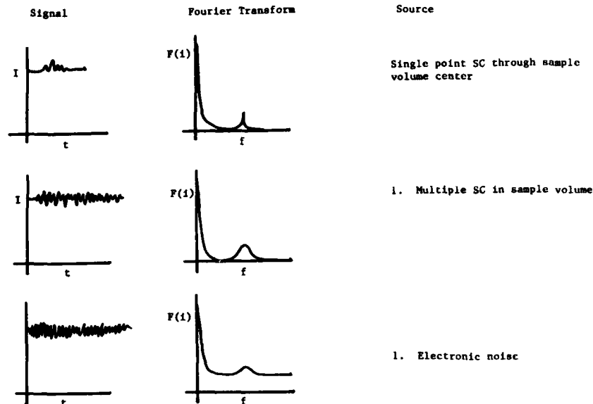
Figure 4.11 LDV signal types - reference scatter systems
