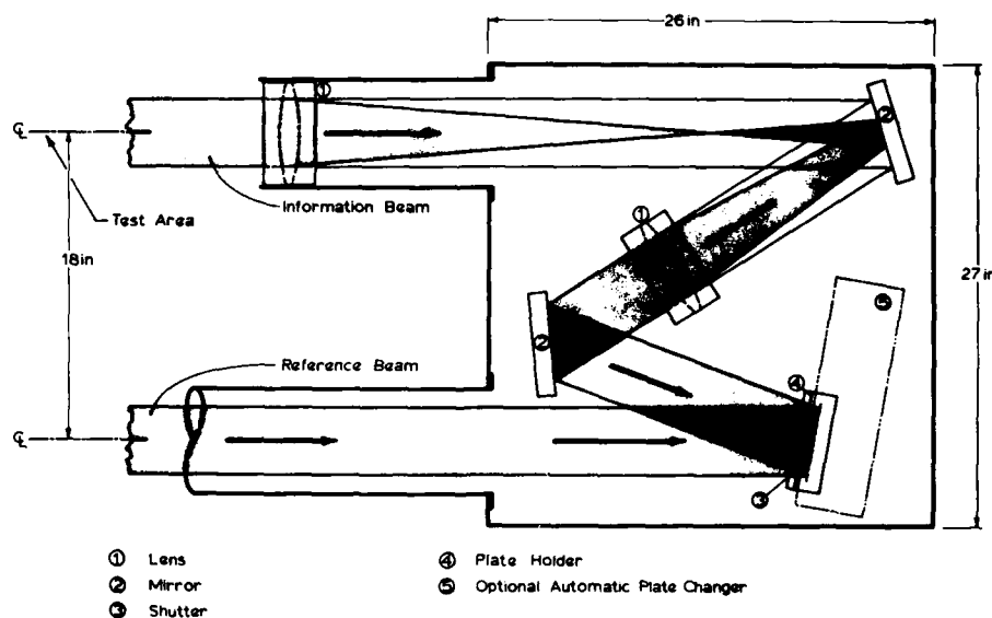
Figure 3.10b Receiver
