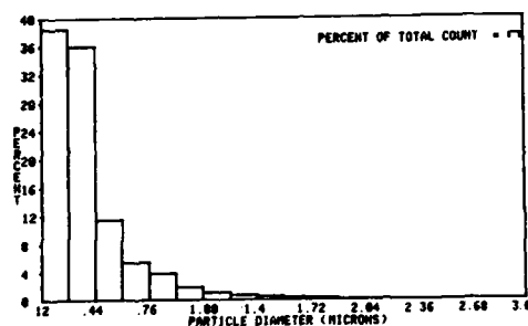
Figure 4.33k DOP in the Laskin nozzle.
