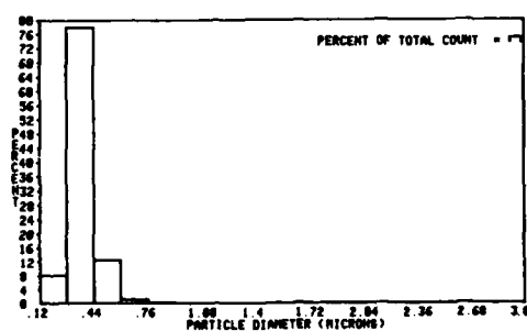
Figure 33o Ethanol and DOP in the ratio 99/1 in the vaporization seeder.
