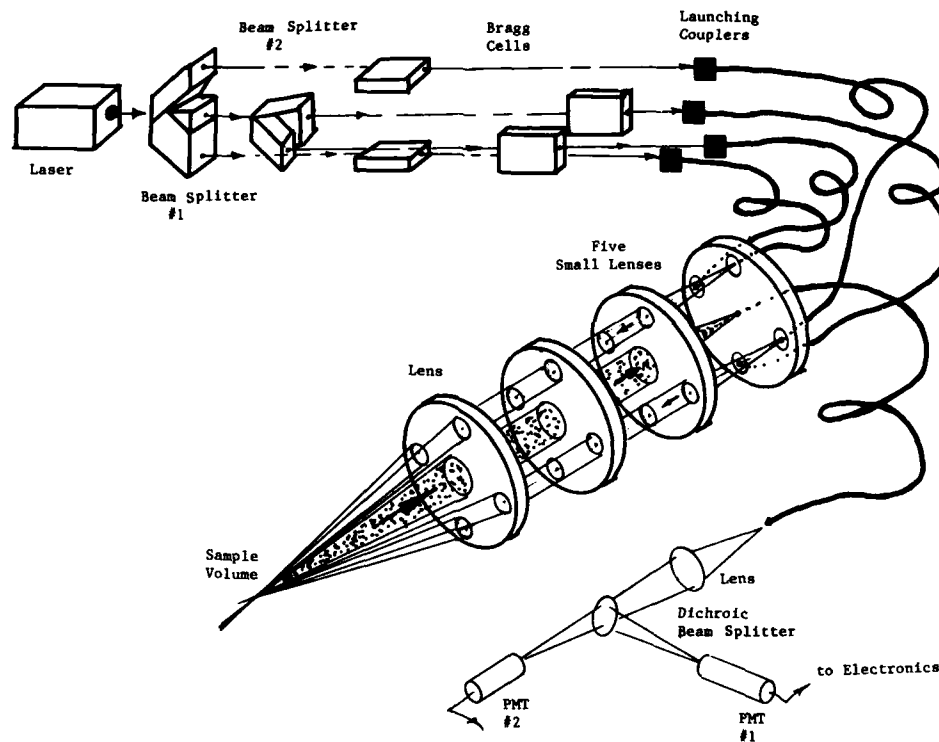
Figure 4.29b Two-component system.
