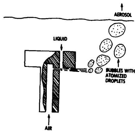
Figure 4.33d Laskin Nozzle
