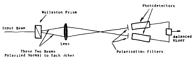
Figure 4.16 Beam splitting with a Wollaston Prism
