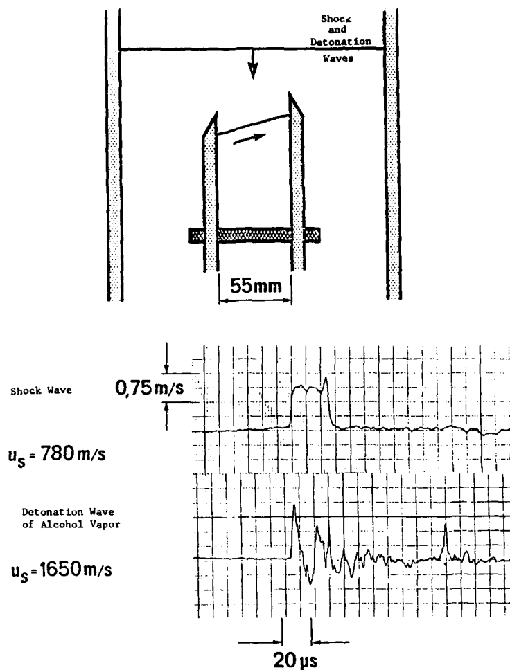
Figure 4.26a Refractive index variation caused by a shock and detonation wave in an explosive alcohol/air mixture.
