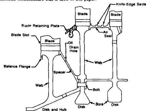
Figure 2. Composite Sketch Of Typical Rotor Components Of A Gas Turbine Engine
