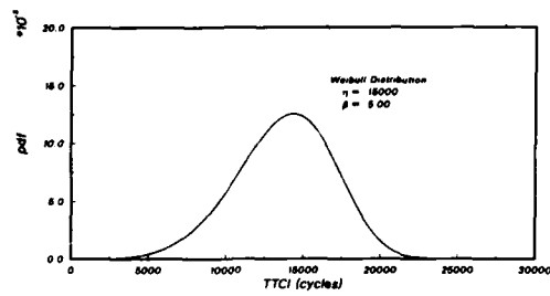
Fig. 17. The LCF cycles to crack initiation distribution for the 5th stage compressor discs. (Ref. 6.)
