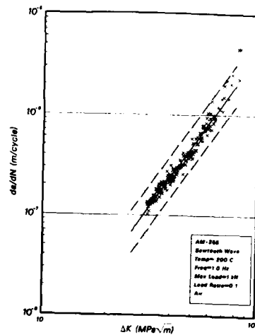
Fig. 8. Fatigue crack growth rate data from six compact tension specimens showing the upper and lower confidence bounds at \pm 3 conditional standard deviations.
