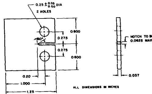
Fig. 3. Geometry of the compact tension specimen used to generate fatigue crack growth rate (FCGR) data at 200°C.
