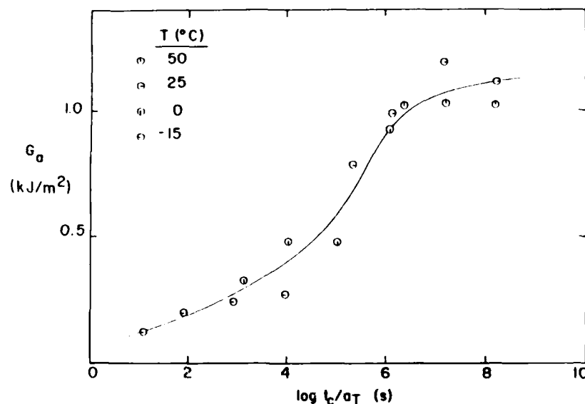
FIG. 11.—Master curve of adhesive fracture energy at 0°C and rate of 5 cm/min, as a function of temperature reduced contact time, t_1 . Reference temperature = 0°C.
