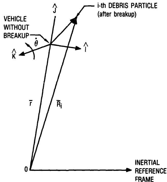
Figure 52. Coordinate Frame
