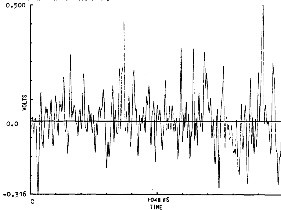
Fig 8 Comparison of raw data at hub and tip - 1st rotor exit
