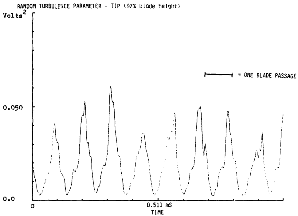
Fig 10 Periodic and random turbulence parameters at the tip - 1st rotor exit
