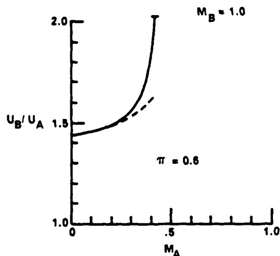
Figure 6. Actuator-disk solution for \pi = 0.6 .
