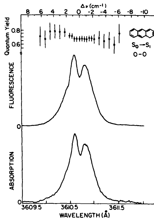
FIG. 8. Absorption spectrum, fluorescence excitation spectrum, and absolute fluorescence quantum yields from the S_0 \rightarrow S_1 electronic origin of anthracene. P = 110 Torr, T = 140^\circ\text{C} , X = 6 mm, spectral resolution 0.6 \text{ cm}^{-1} .
