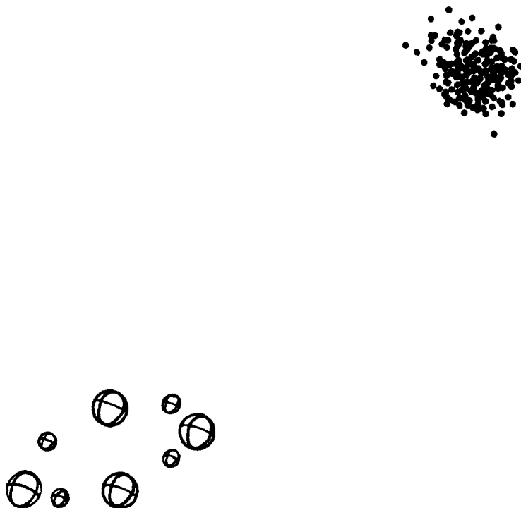
Fig. 18. - Ionic configuration and «electron necklace» distribution for an excess electron interacting with \text{Na}_4\text{Cl}_4^+ cluster and resulting in dissociation detachment (ref. [69]).
