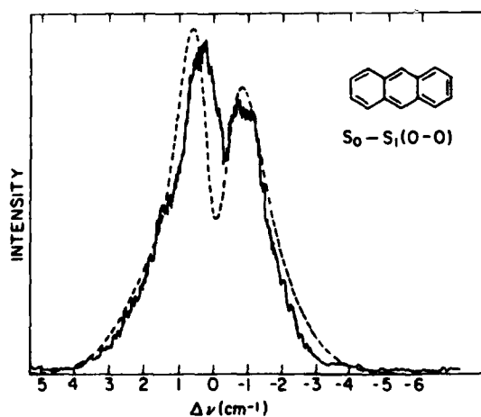
FIG. 7. A comparison between the experimental spectrum of the electronic origin of anthracene in a planar supersonic jet P = 110 Torr, T = 130^\circ\text{C} , X = 10 mm, spectral resolution 0.5 \text{ cm}^{-1} (solid curve) with the numerical simulation of the rotational contour at T_{\text{rot}} = 20 K.
