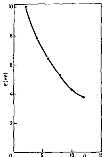
Fig. 27. - Estimates of the energy required for the symmetric fission of (\text{H}_2\text{O})_n clusters: (\text{H}_2\text{O})_n^* \rightarrow \text{H}^+(\text{H}_2\text{O})_p + (\text{OH}^-)(\text{H}_2\text{O})_p ; 2p + 1 = n . Data from ref. [89].
