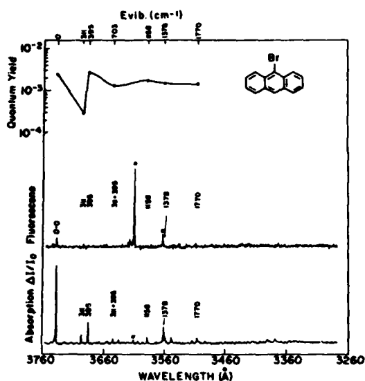
FIG. 18. Absorption spectrum, fluorescence excitation spectrum, and absolute fluorescence quantum yields of 9-bromoanthracene over the spectral region 3760–3260 Å. P = 100 Torr, T = 145^\circ\text{C} , and X = 6 mm. Notation as in Fig. 11. The spectral features in the LMIF spectrum marked by a star (*) correspond to an impurity of anthracene.
