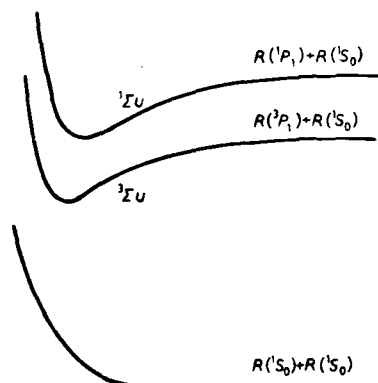
Fig. 20. - Potential curve for the formation of R_n^* electronically excited diatomic rare-gas molecule.
