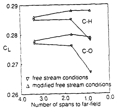
Fig 7 Variation of lift with position of far-field boundary
