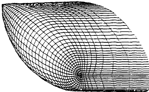
Fig 5 Surface grid at the wing tip (leading edge)
