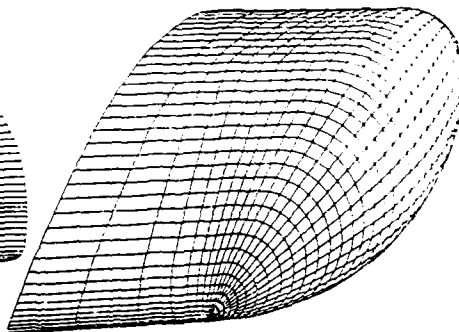
Fig 6 Surface grid at the wing tip (trailing edge)
