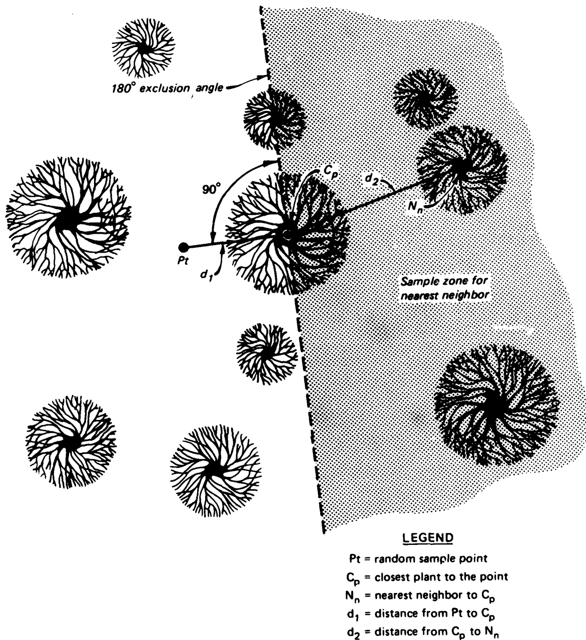
Figure 4. Application of the T-square nearest-neighbor method (adapted from Hays et al. 1981)
