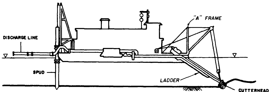
Figure 3. Hydraulic pipeline cutterhead dredge
