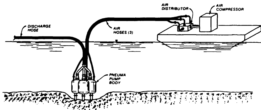
Figure 8. PNEUMA pump
