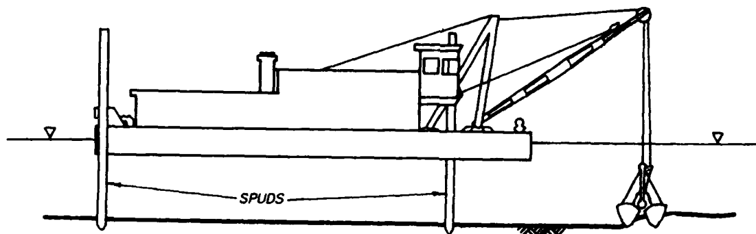
Figure 2. Bucket dredge
