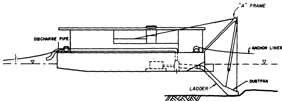
Figure 6. Dustpan dredge
