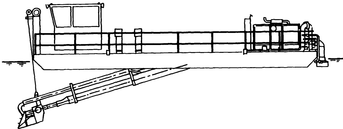
Figure 16. Muck Duck dredge - jet pump
