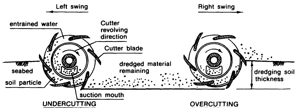
Figure 5. Cutting operation (front view)
