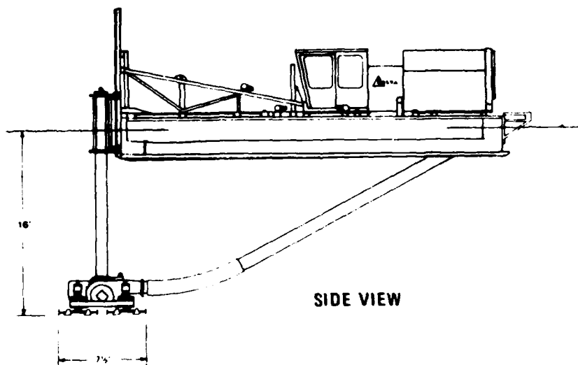
Figure 14. Delta dredge (from Barnard 1978)
