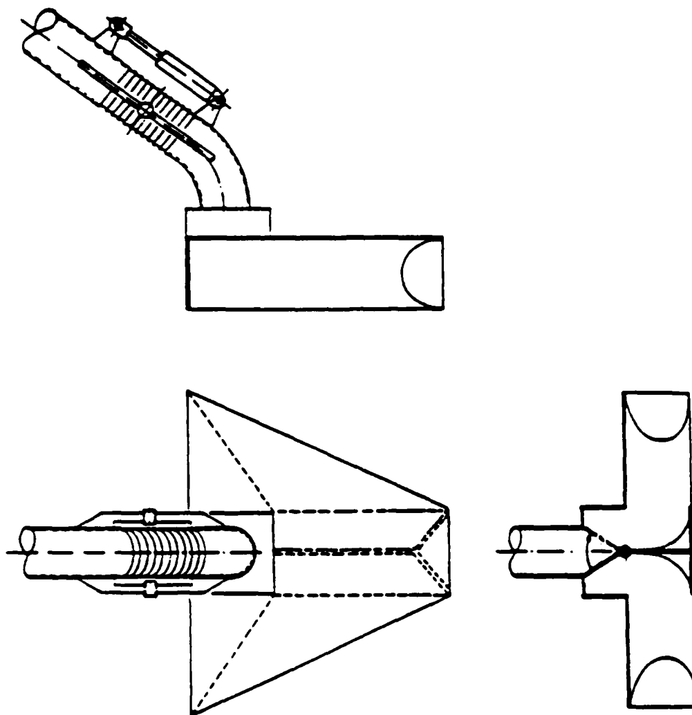
Figure 11. Matchbox head
