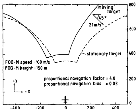
Figure 7. Footprint against moving ground targets.
