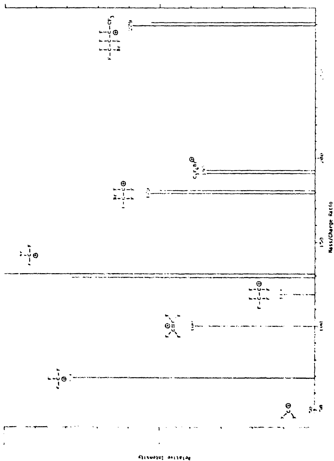
Figure I-4. Mass Spectrum of Component Assigned as \text{CF}_2\text{BrCF}_2\text{CFXCF}_3 .
