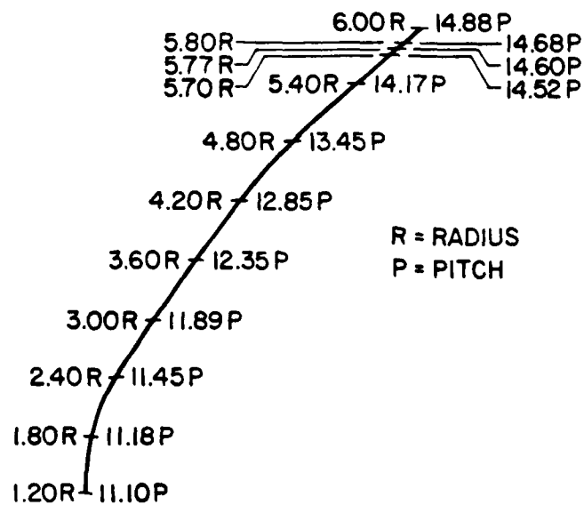
FIGURE 9: PITCH DIAGRAM
