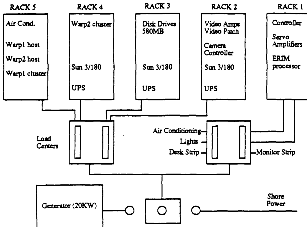
Figure 5-1: Wiring Schematic for AC Power
