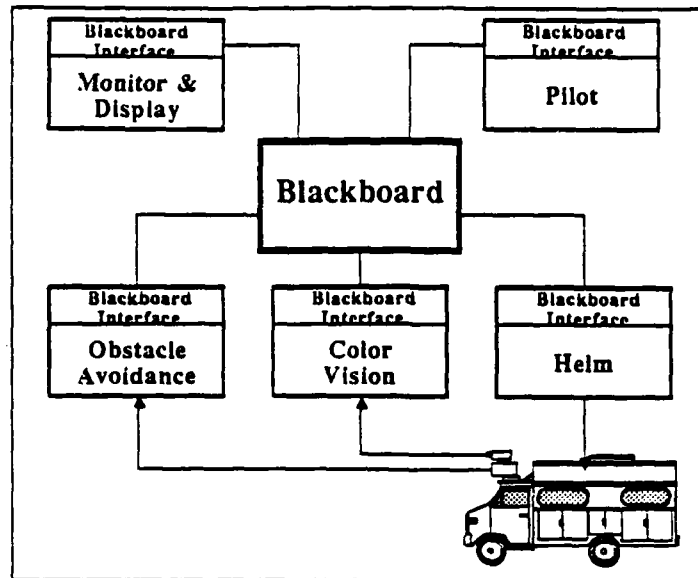
Figure 19: Navlab software architecture
