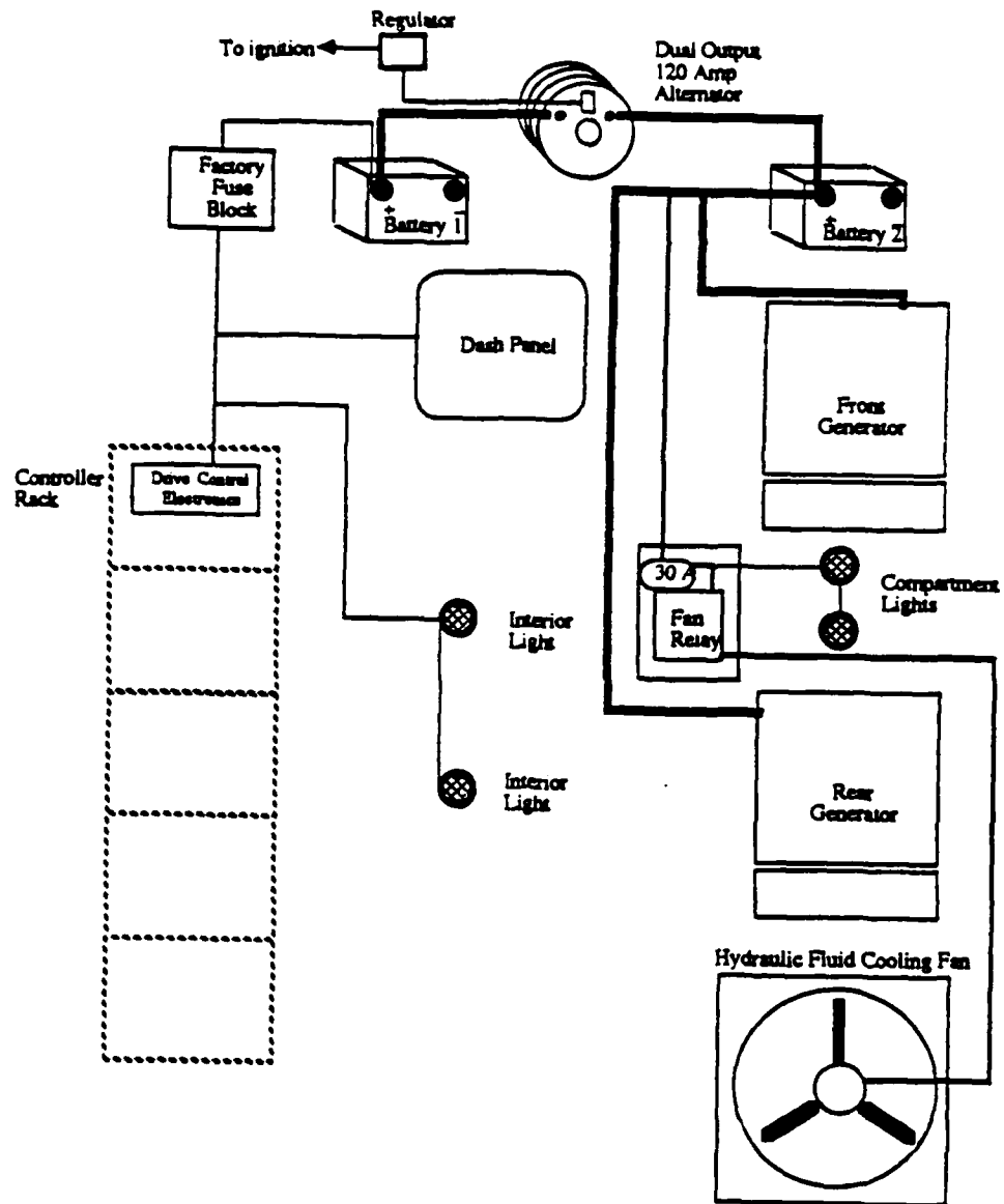
Figure 5-2: Wiring Schematic for DC Power
