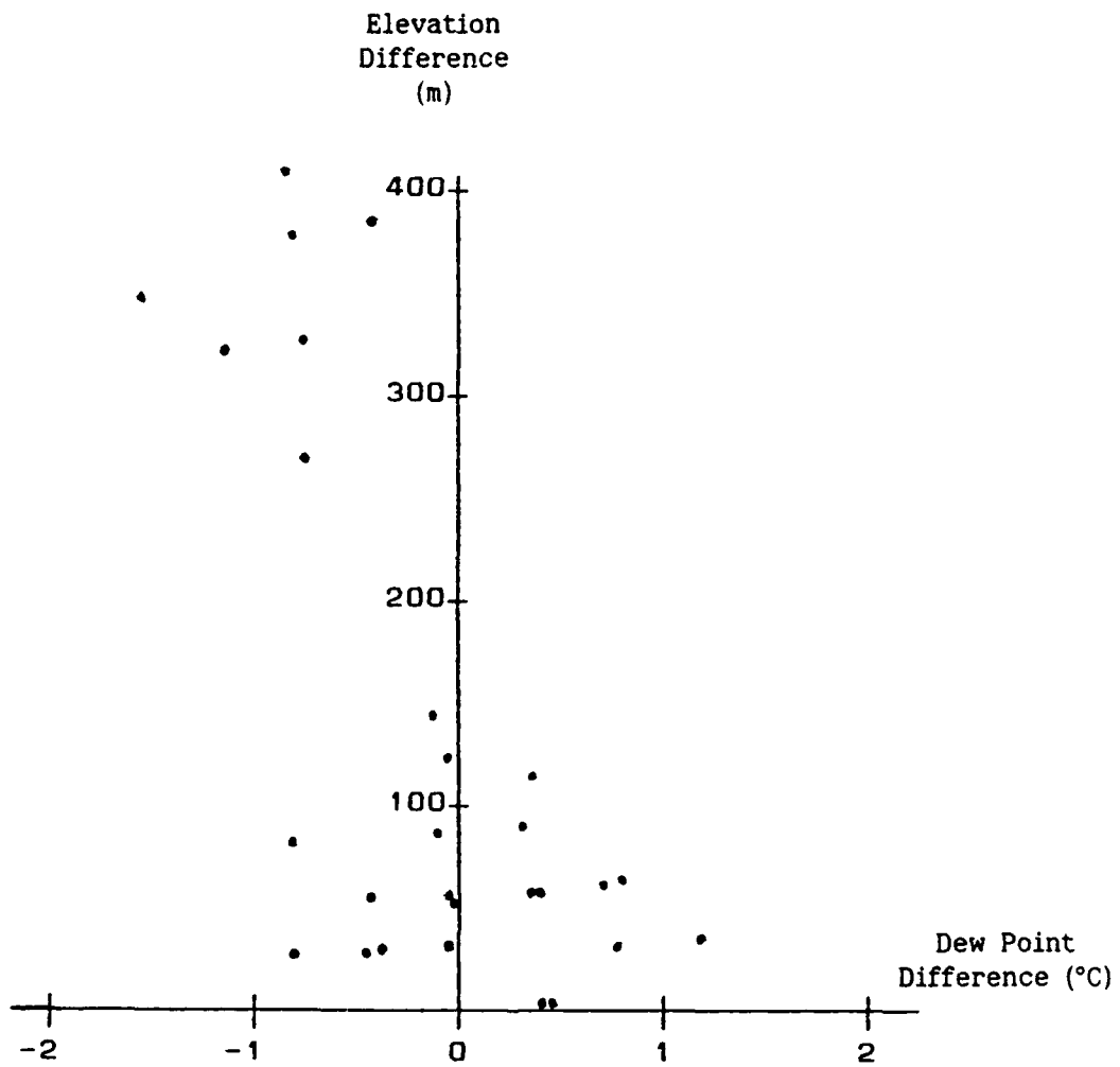
Figure 17. Graph to compare difference in elevation with difference in dew point during the time 2000-2259 GMT (1500-1759 CDT).
