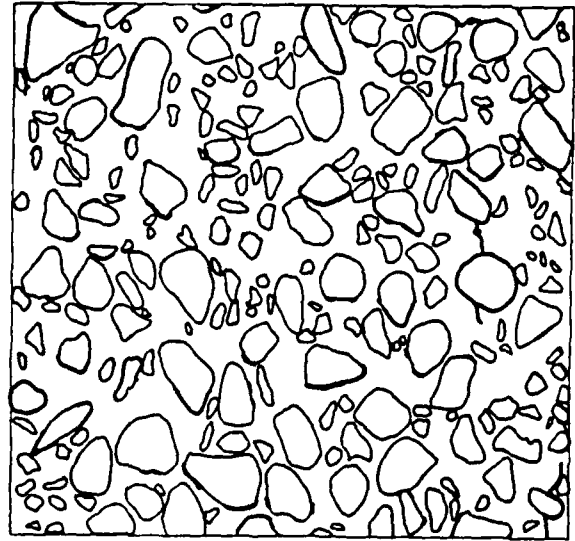
LOAD UP TO 0.83 f'_c IN THE PRE-PEAK REGION
