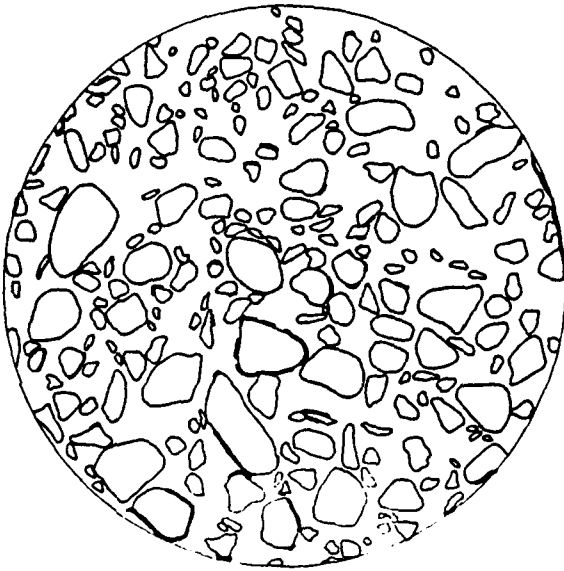
LOAD UP TO 0.83 f'_c IN THE PRE-PEAK REGION
