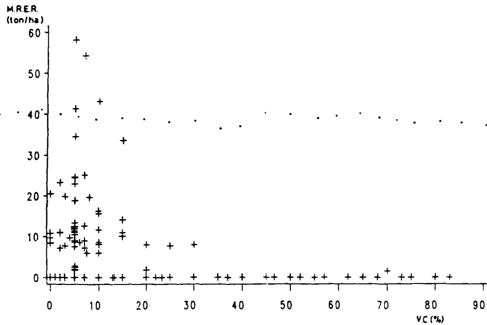
Fig. 111.4 Relationship between rill erosion rate and vegetation cover
