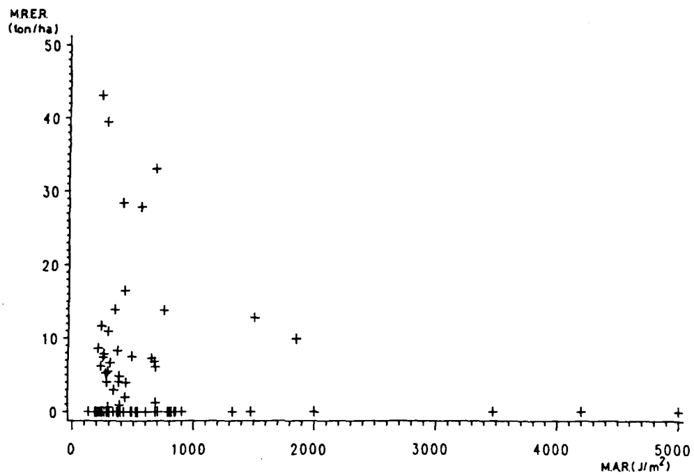
Fig. 111.3 Influence of aggregate resistance on rill erosion
