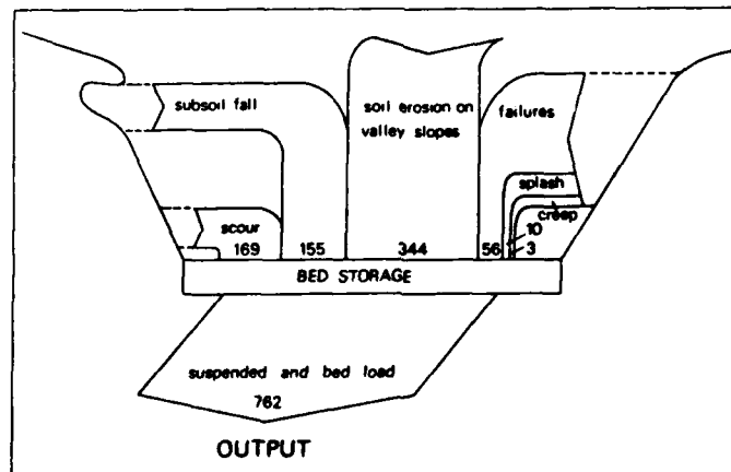
Fig. 22. Sediment budget for the Schrondeweilerbaach catchment 1979-1981. Numbers are in kg.ha -1 .yr -1 .
