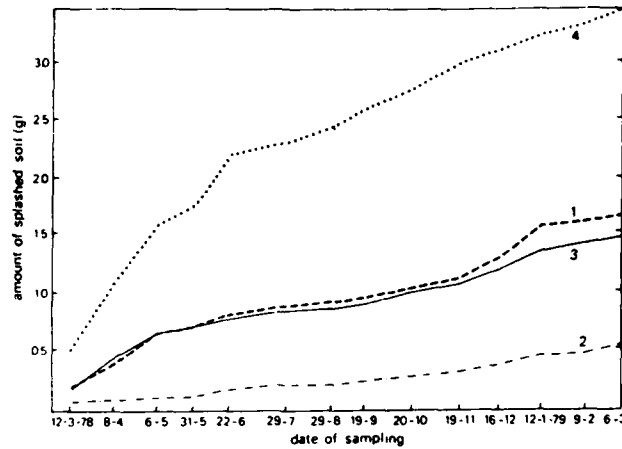
Fig. 6. Cumulative amount of soil splashed from undisturbed soil samples during laboratory experiments. 1. forest (colluvium) 2. pasture 3. forest (A1) 4. arable farmland
