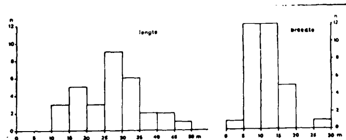
Fig. 12. Blowouts classified according to length and width
