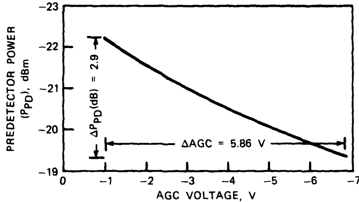
FIGURE 1-13. Detector Input Power Versus AGC Voltage (Low-Pass Filter).
