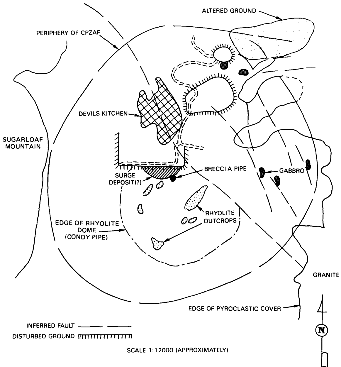
(a) Geology of proposed CPZAF. FIGURE 1-4. Portion of Coso Volcanic Field Showing Coso Production Zone Arcuate Feature (CPZAF).
