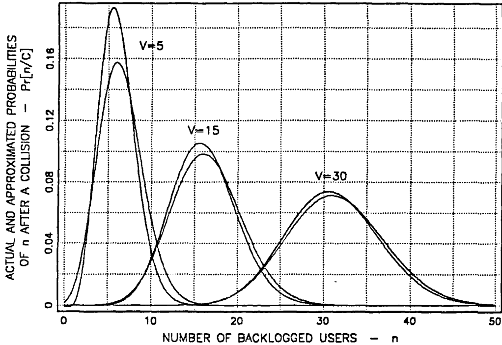
Figure 2.7: Comparison of the Actual and Poisson Approximating Probability Distributions of the Number n of Backlogged Users after a Collision Occurs in a Slotted CSMA/CD Network with Two Power Levels. ( G_s = 2 )
