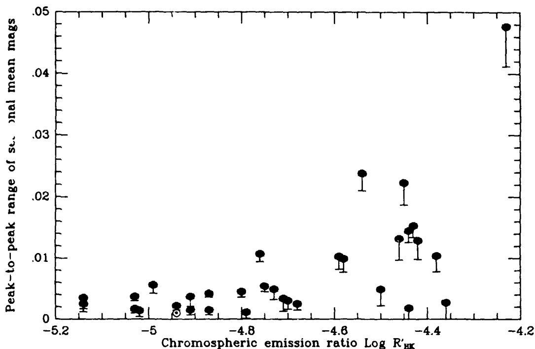
Figure 18. Interseason range of variation over four years plotted as a function of the chromospheric emission ratio \log R'_{HK} . The error bar "tails" indicate the 95% confidence interval for the range: if the bars lie above zero, the star is considered variable.
