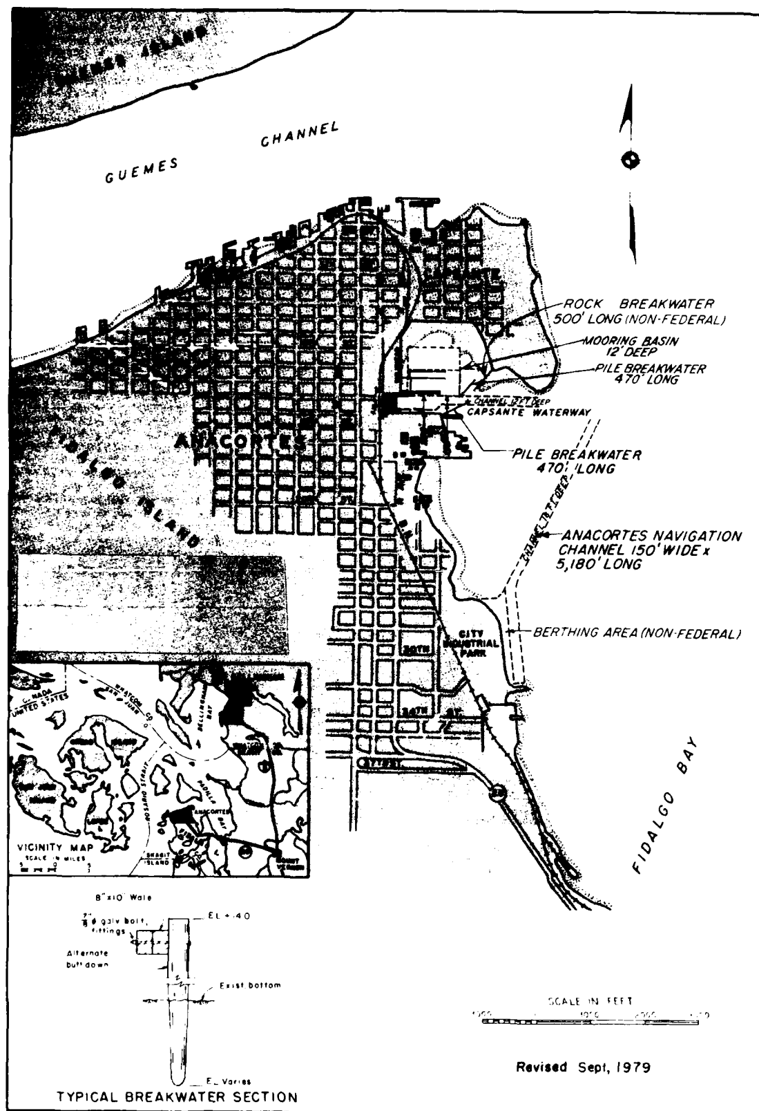
Figure 66. Site layout of Anacortes Harbor, Washington (revised 1979)
