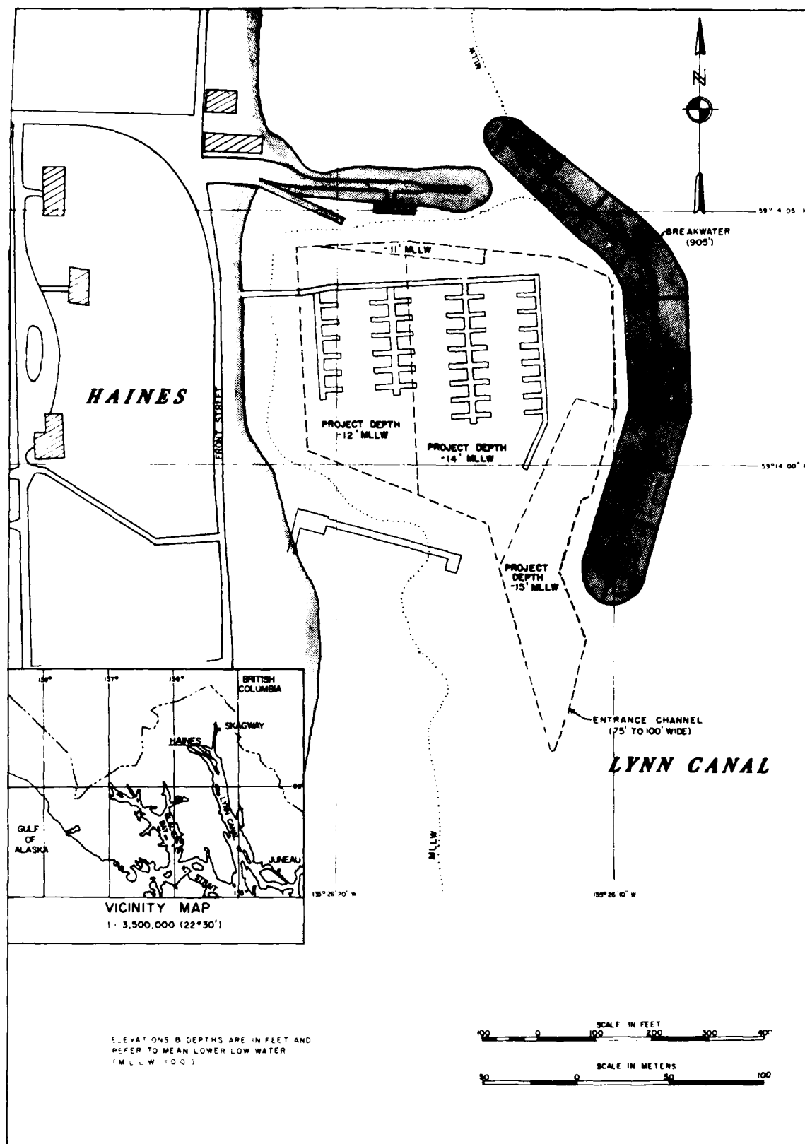
Figure 11. Site layout for Haines Harbor, Alaska (revised 1981)
