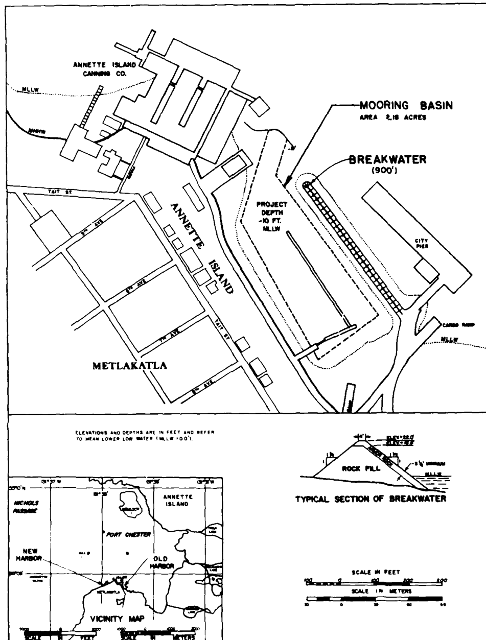
Figure 29. Site layout of Metlakatla Old Harbor, Alaska
