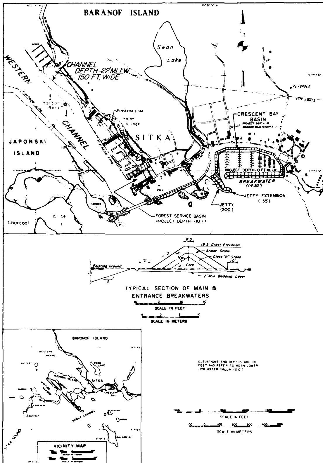
Figure 46. Site layout of Sitka Harbor, Alaska (revised 1981)
