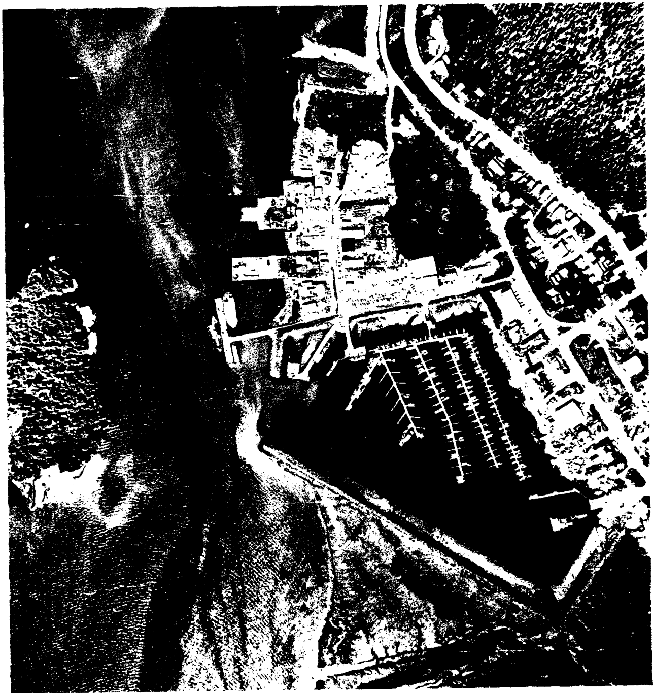
Figure 4. Aerial photograph of Cordova Harbor, Alaska, 1977
