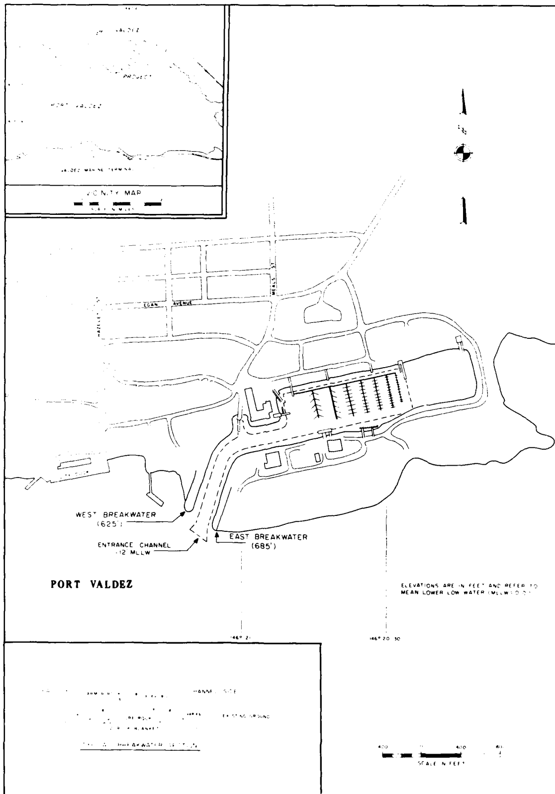
Figure 48. Site layout of Valdez Harbor, Alaska, 1985
