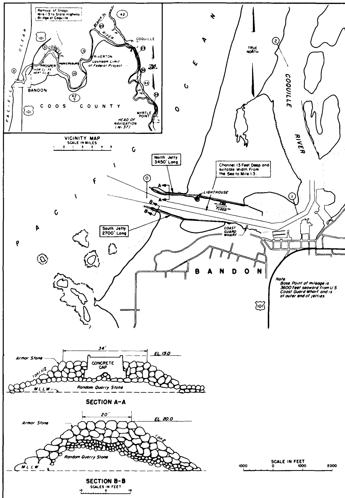
Figure 55. Site layout of Coquille River, Oregon (revised 1981)
