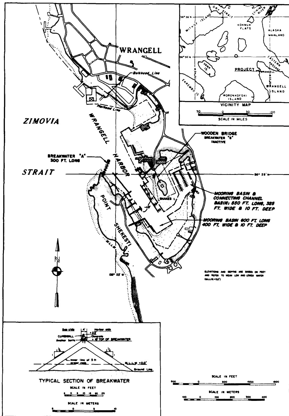
Figure 50. Site layout of Wrangell Harbor, Alaska (revised 1981)
