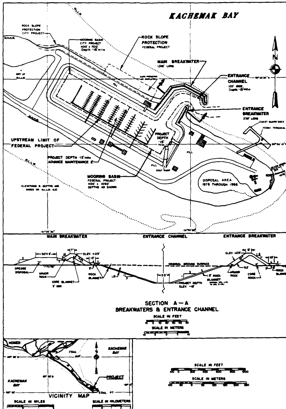
Figure 13. Site layout of Homer Harbor prior to expansion during 1984-1985 (revised 1978)
