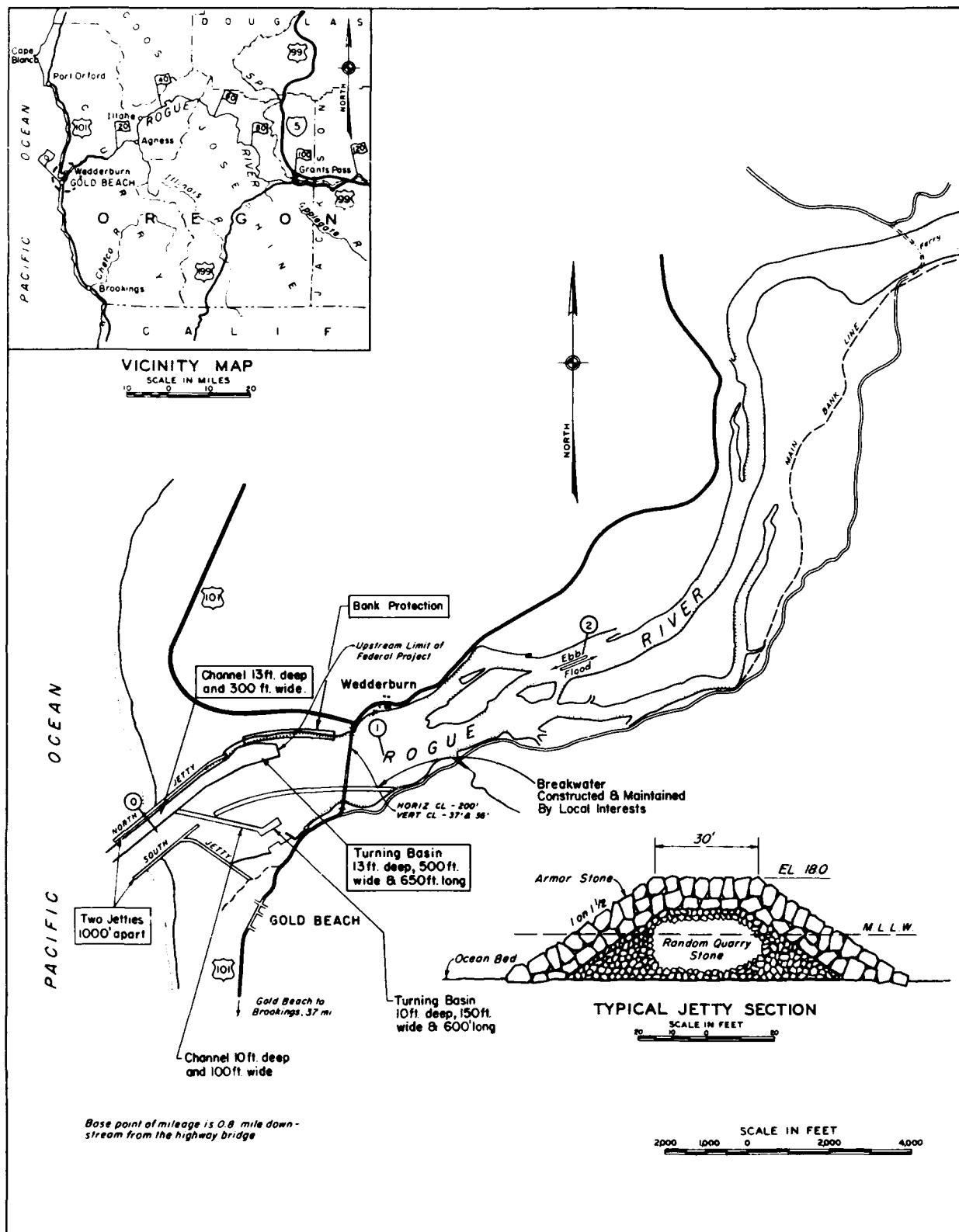
Figure 59. Site layout at Rogue River, Oregon (revised 1977)
