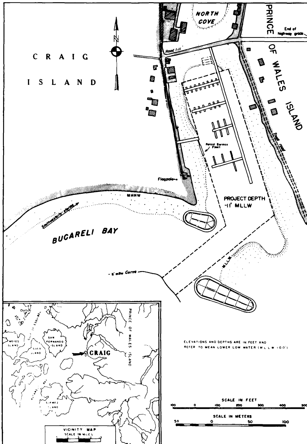
Figure 7. Site layout of Craig Harbor, Alaska (revised 1985)
