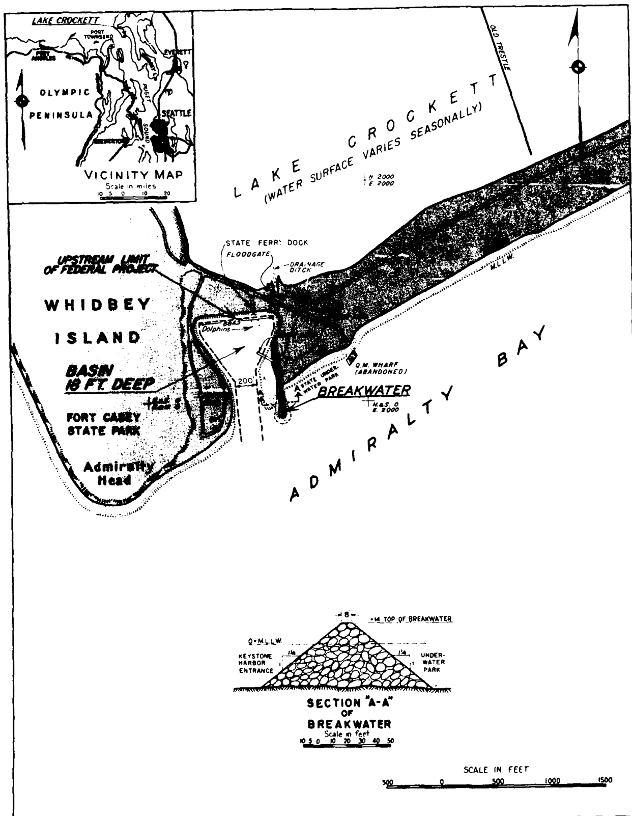
Figure 72. Site layout at Lake Crockett, Washington (revised 1979)
