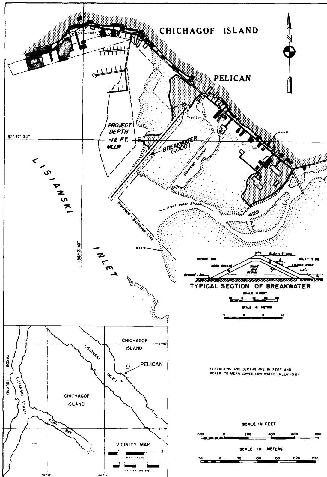
Figure 38. Site layout of Pelican Harbor, Alaska (revised 1981)
