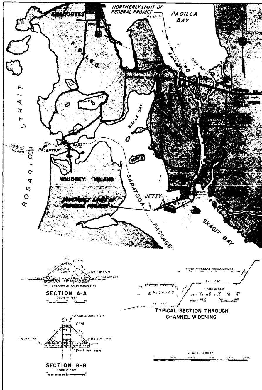
Figure 79. Site layout of Swinomish Channel, Washington (revised 1979)
