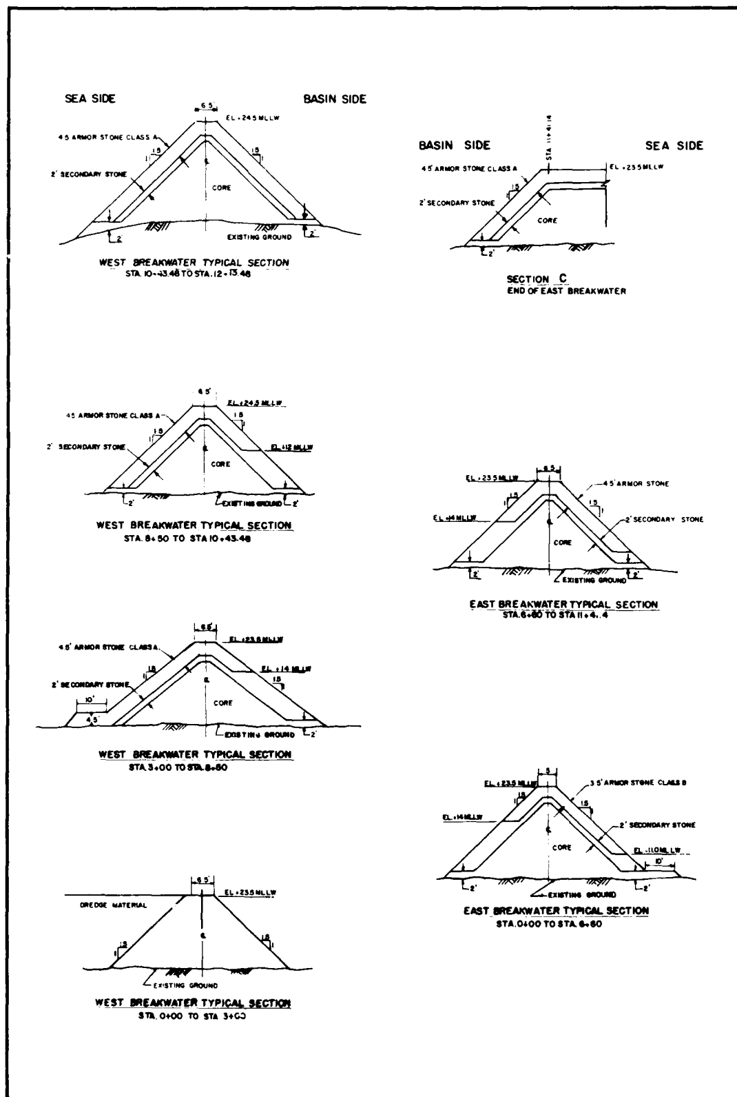
Figure 32. Breakwater cross sections, Metlakatla New Harbor, Alaska
