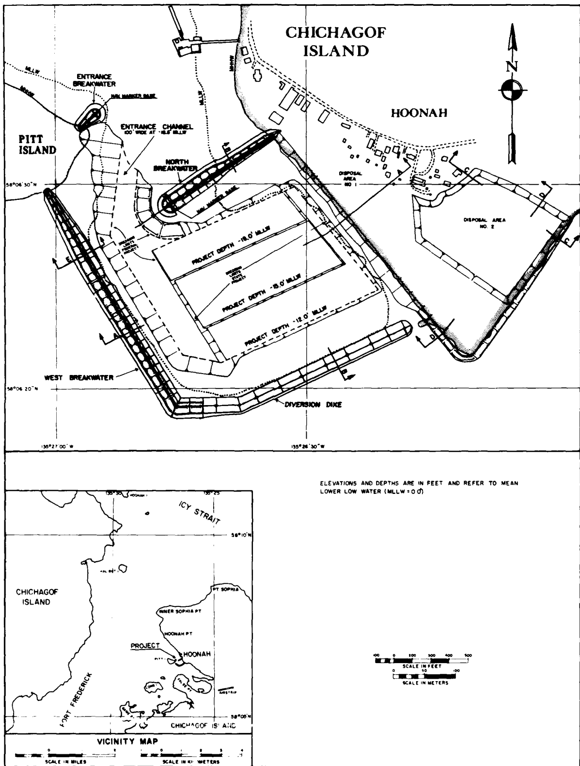
Figure 16. Site layout of Hoonah Harbor, Alaska (revised 1981)
