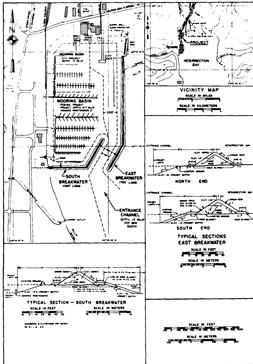
Figure 44. Site layout of Seward Harbor, Alaska (revised 1984)
