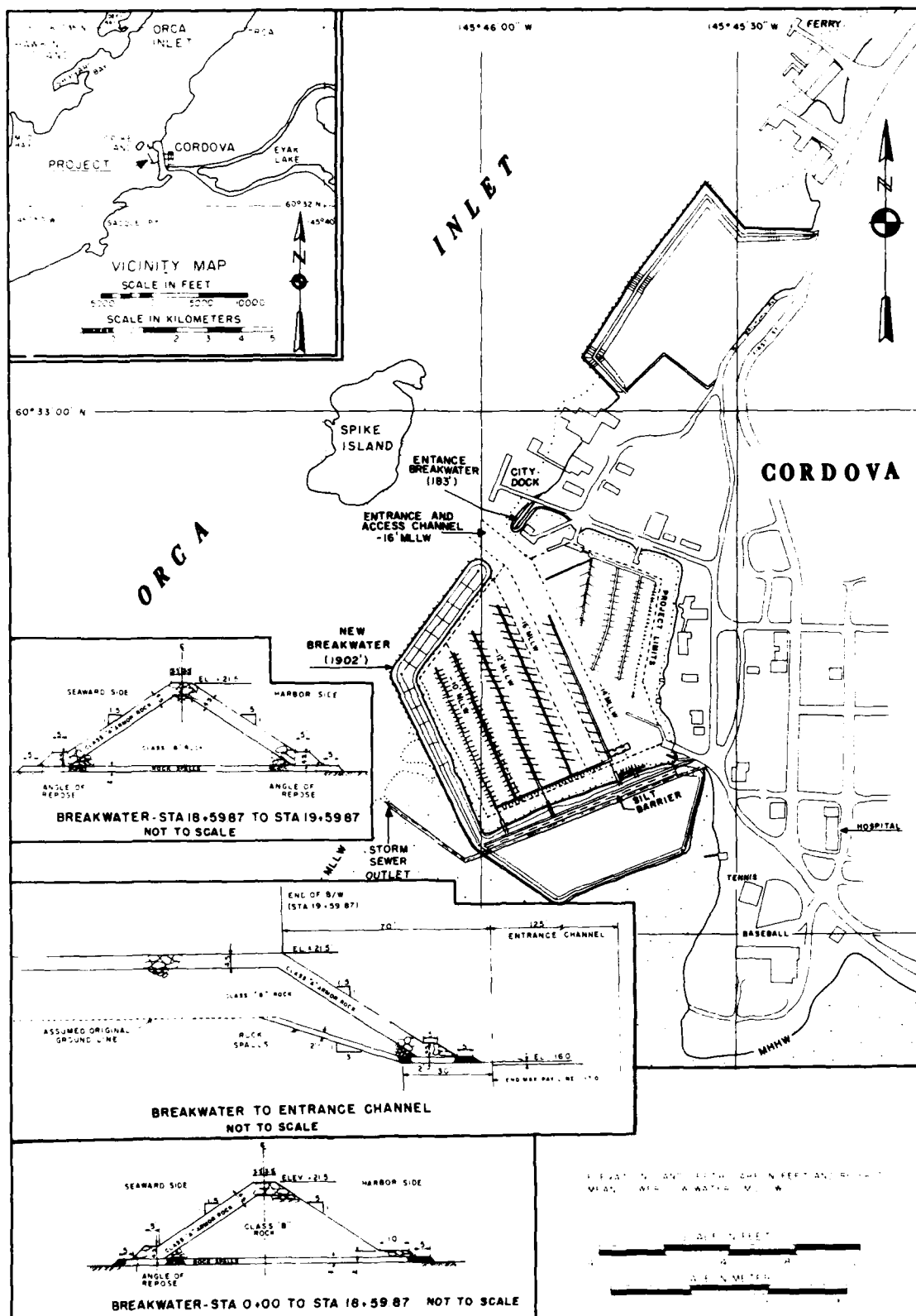
Figure 5. Site layout of Cordova Harbor, Alaska (revised 1985)
