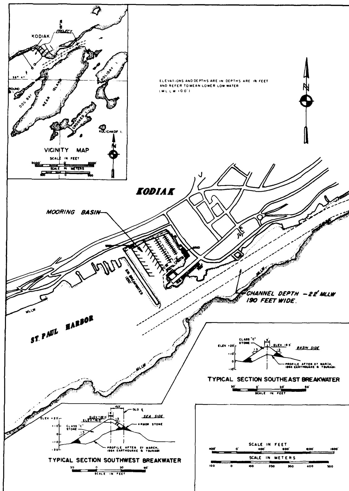
Figure 27. Site layout of Kodiak Harbor, Alaska (revised 1978)
