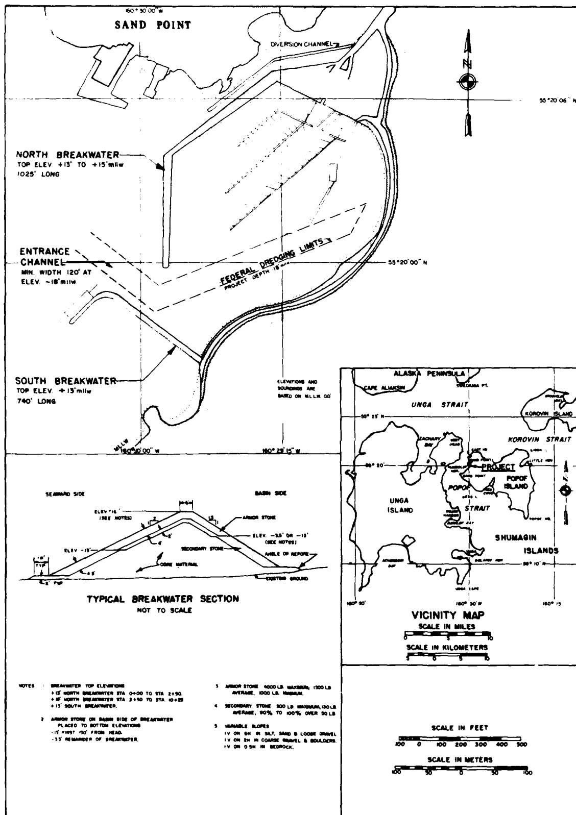
Figure 19. Site layout of Humboldt Harbor, Alaska (revised 1984)
