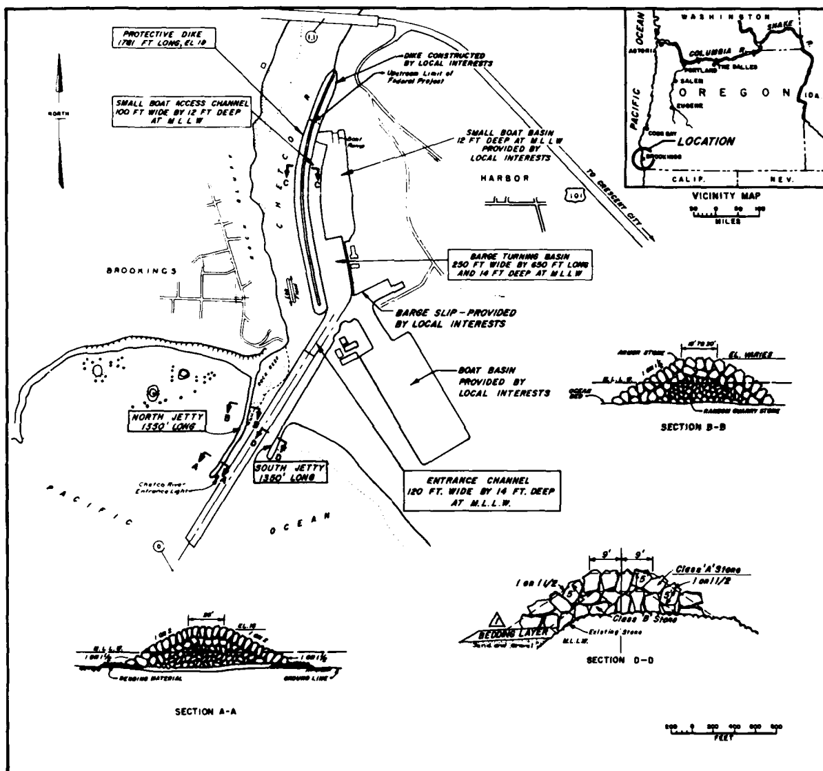
Figure 52. Site layout of Chetco River, Oregon (revised 1979)
