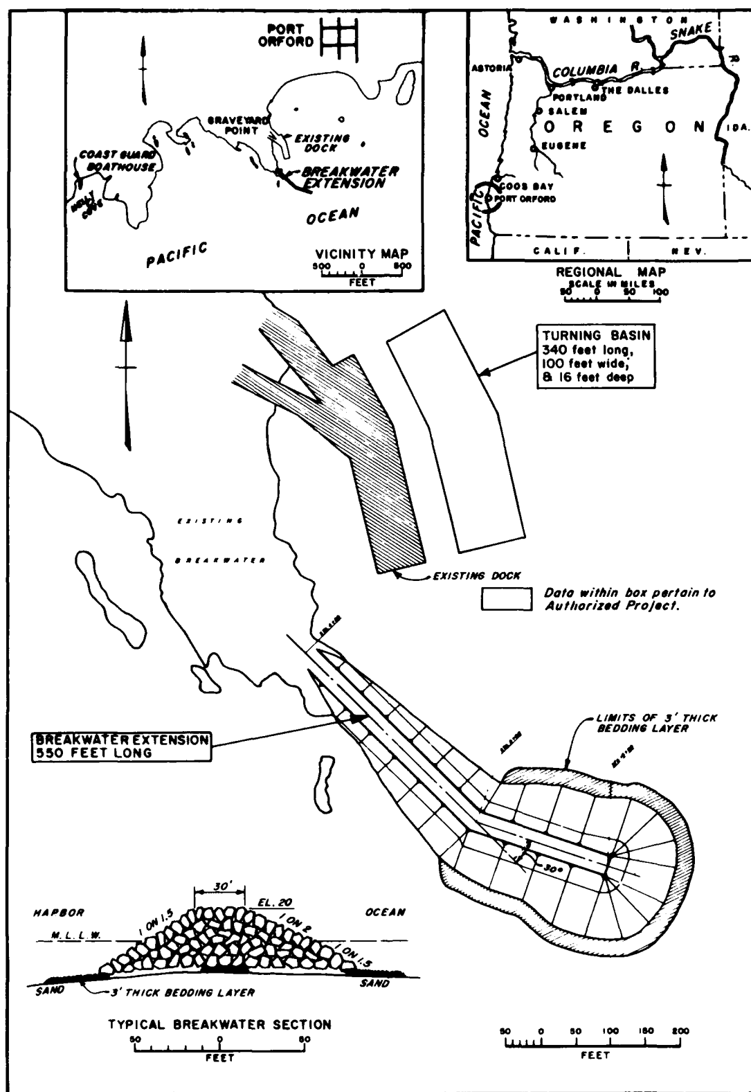
Figure 58. Site layout of Port Orford, Oregon (revised 1971)
