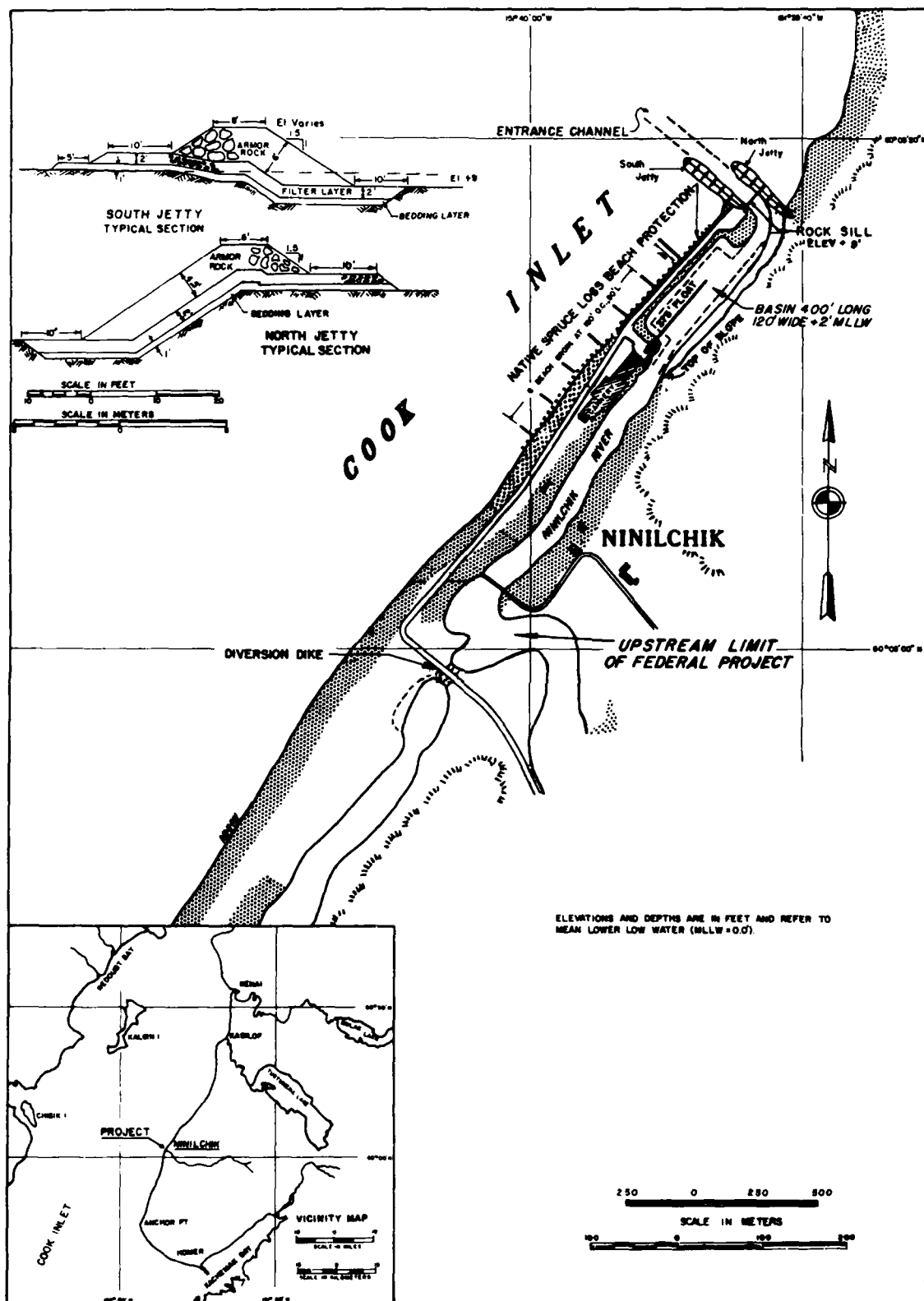
Figure 34. Layout of Ninilchik Harbor, Alaska (revised 1981)
