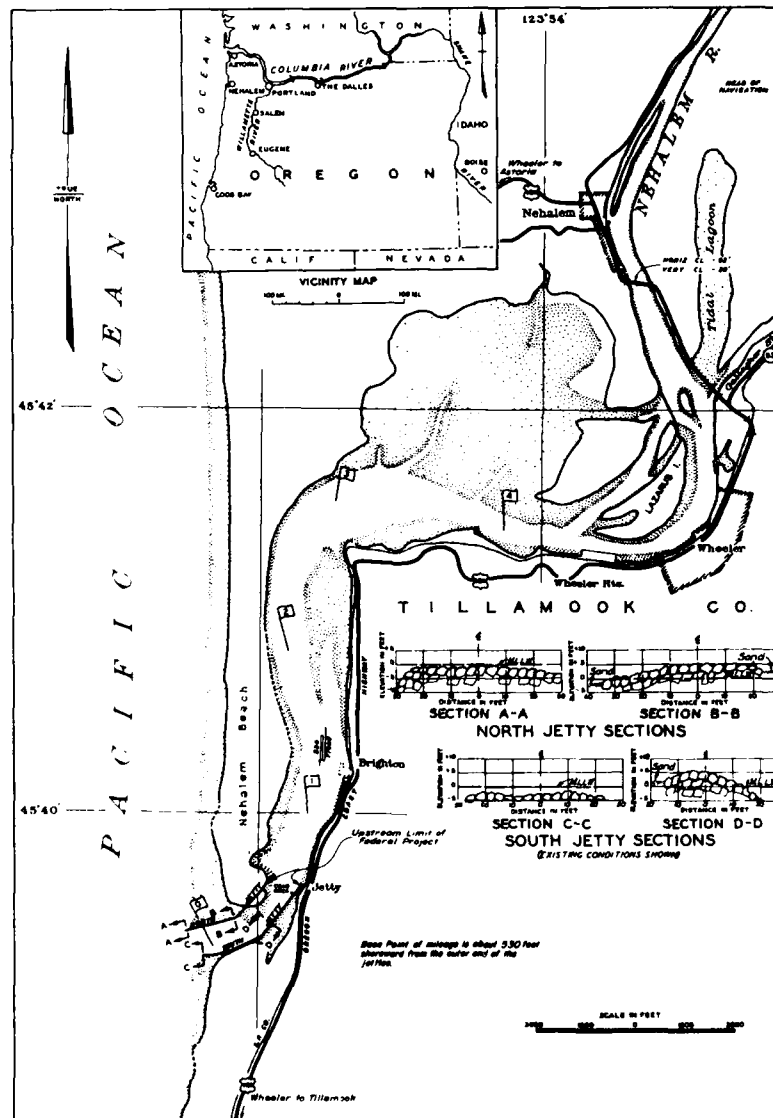
Figure 57. Site layout of Nehalem Bay, Oregon (revised 1979)
