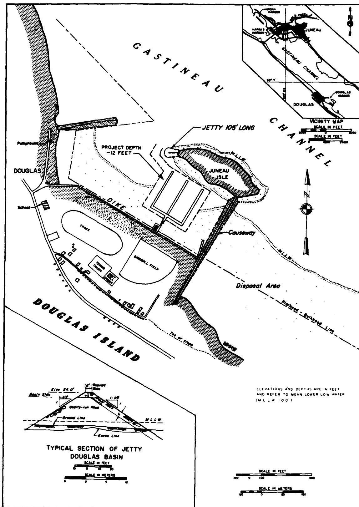
Figure 9. Site layout of Douglas Harbor, Alaska (revised 1978)
