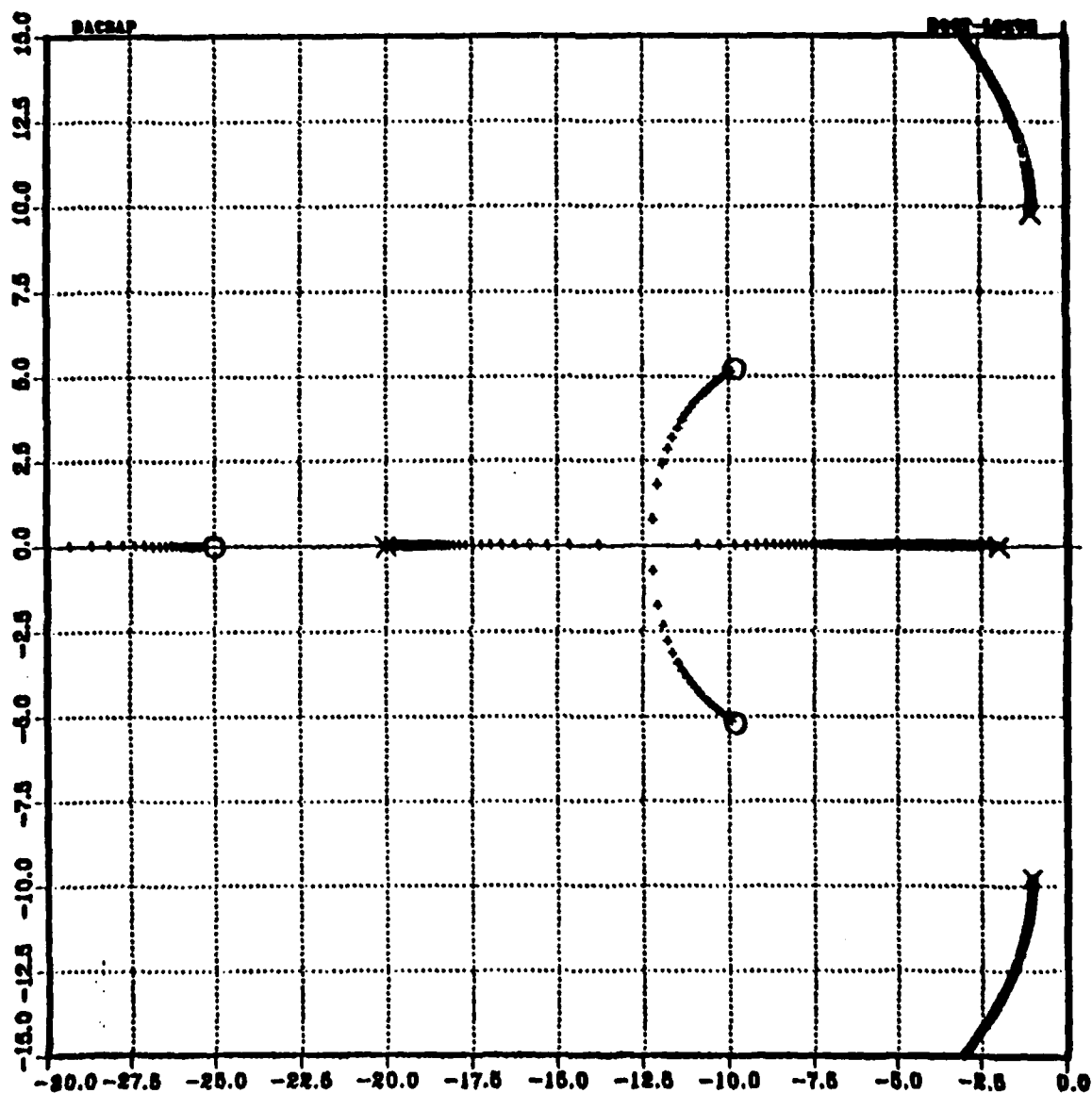
Figure 60. Offsetting The Zeros For The First Time. Desired Roots; -10.000 \mp j5.000 , -25.000
