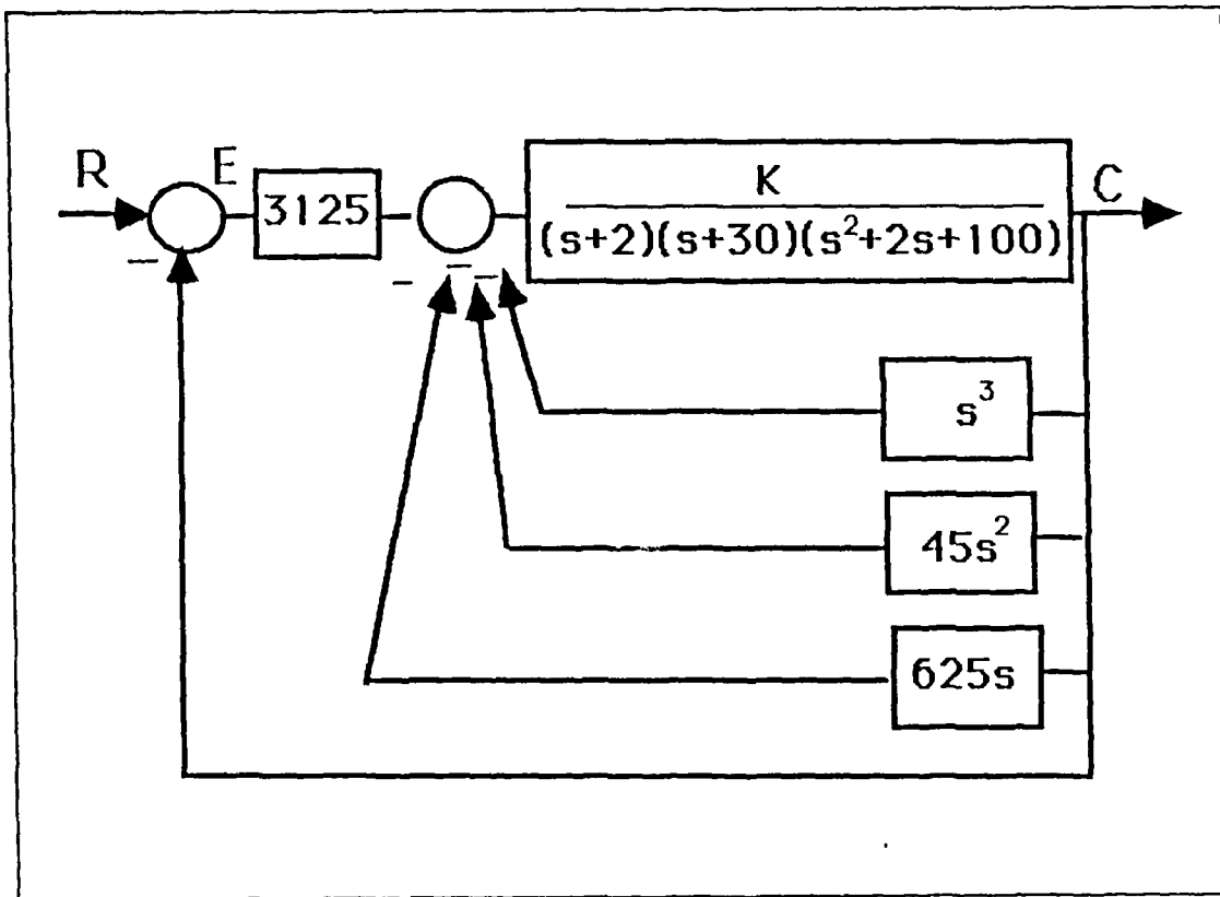
Figure 32. Rearranged Block Diagram
