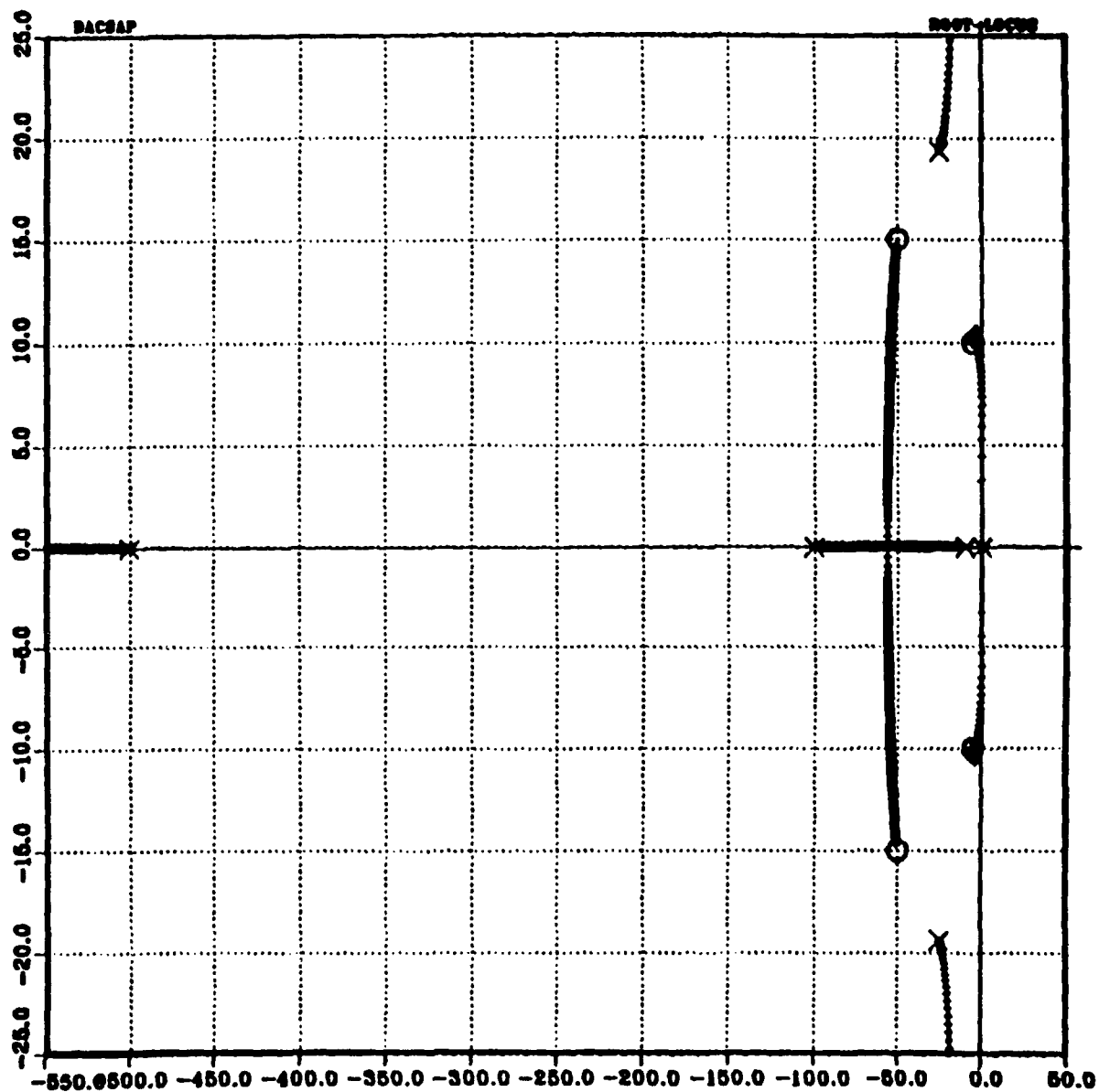
Figure 65. Offsetting The Zeros For The Second Time. Desired Roots; -5.000 \mp j10.000 , -50.000 \mp j15.000 , -300 \mp j200
