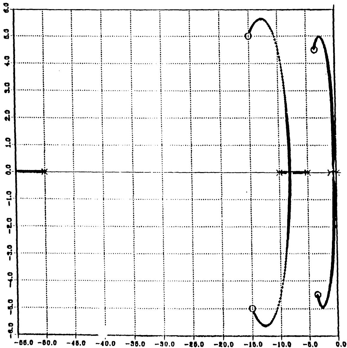
Figure 56. Offsetting The Zeros For The Second Time. Desired Roots: -3.000 \pm j5.000 , -15.000 \pm j5.000
