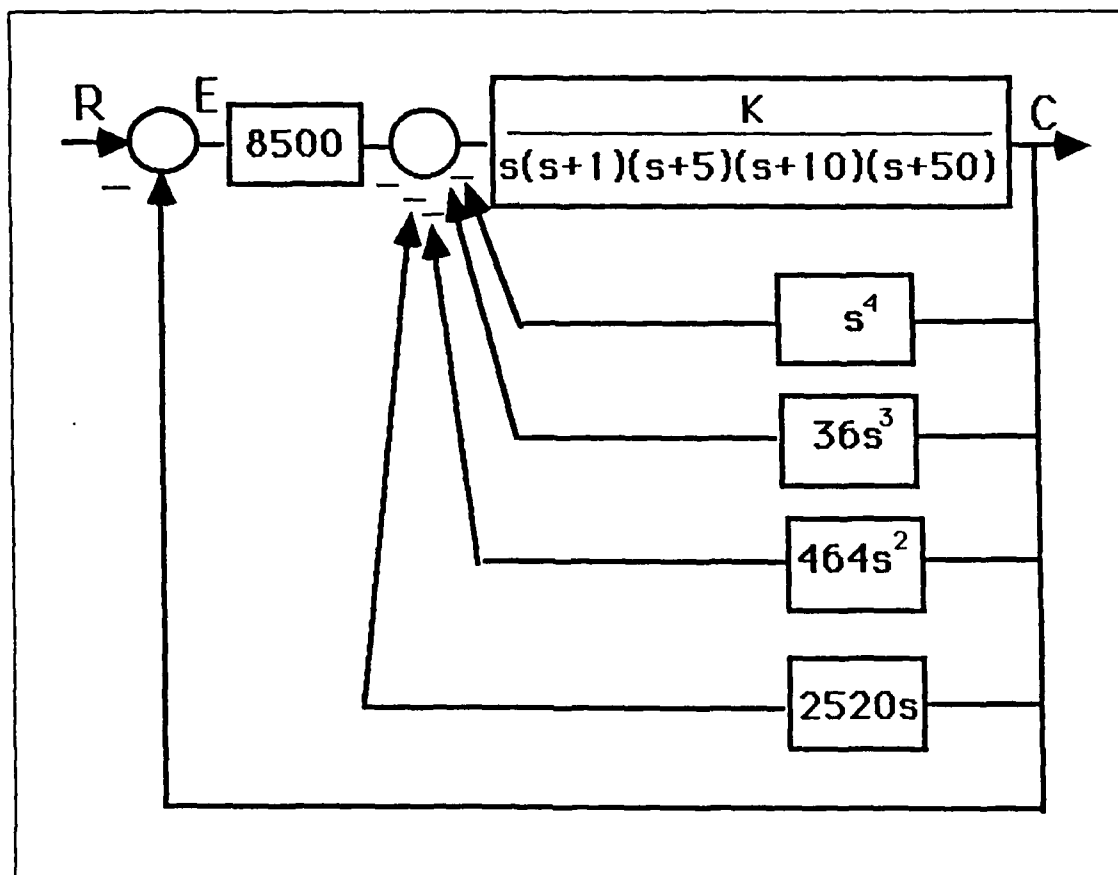
Figure 24. Rearranged Block Diagram
