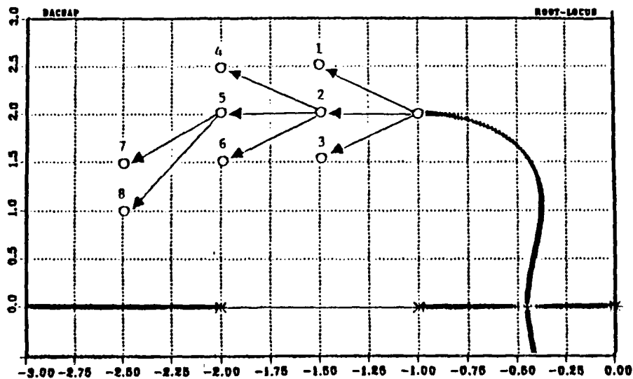
Figure 52. Arbitrarily Chosen Offset Zero Location (I)
