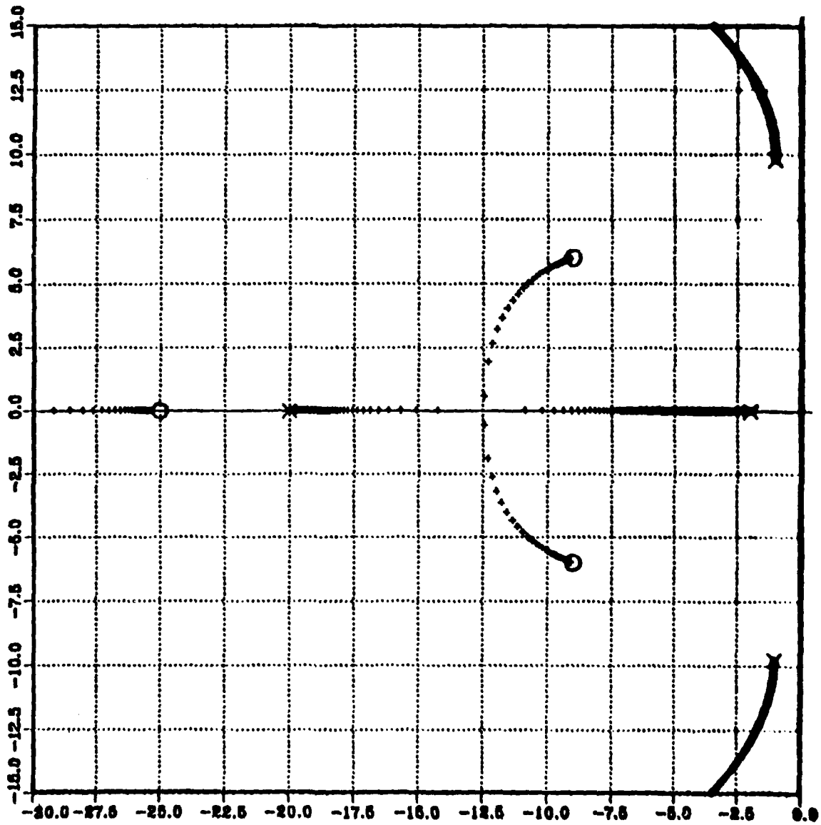
Figure 62. Offsetting The Zeros For The Third Time. Desired Roots; -10.000 \pm j5.000 , -25.000
