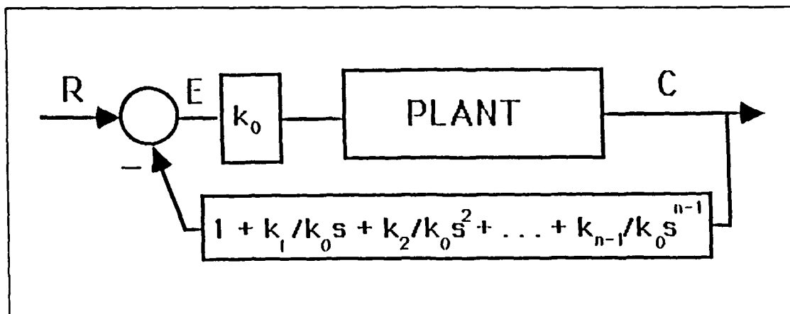
Figure 4. Rearrangement To Preserve Unity Feedback.
