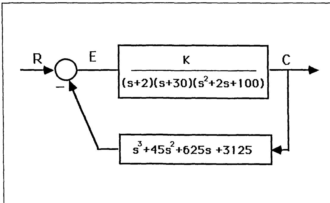
Figure 30. Basic State Feedback Block Diagram
