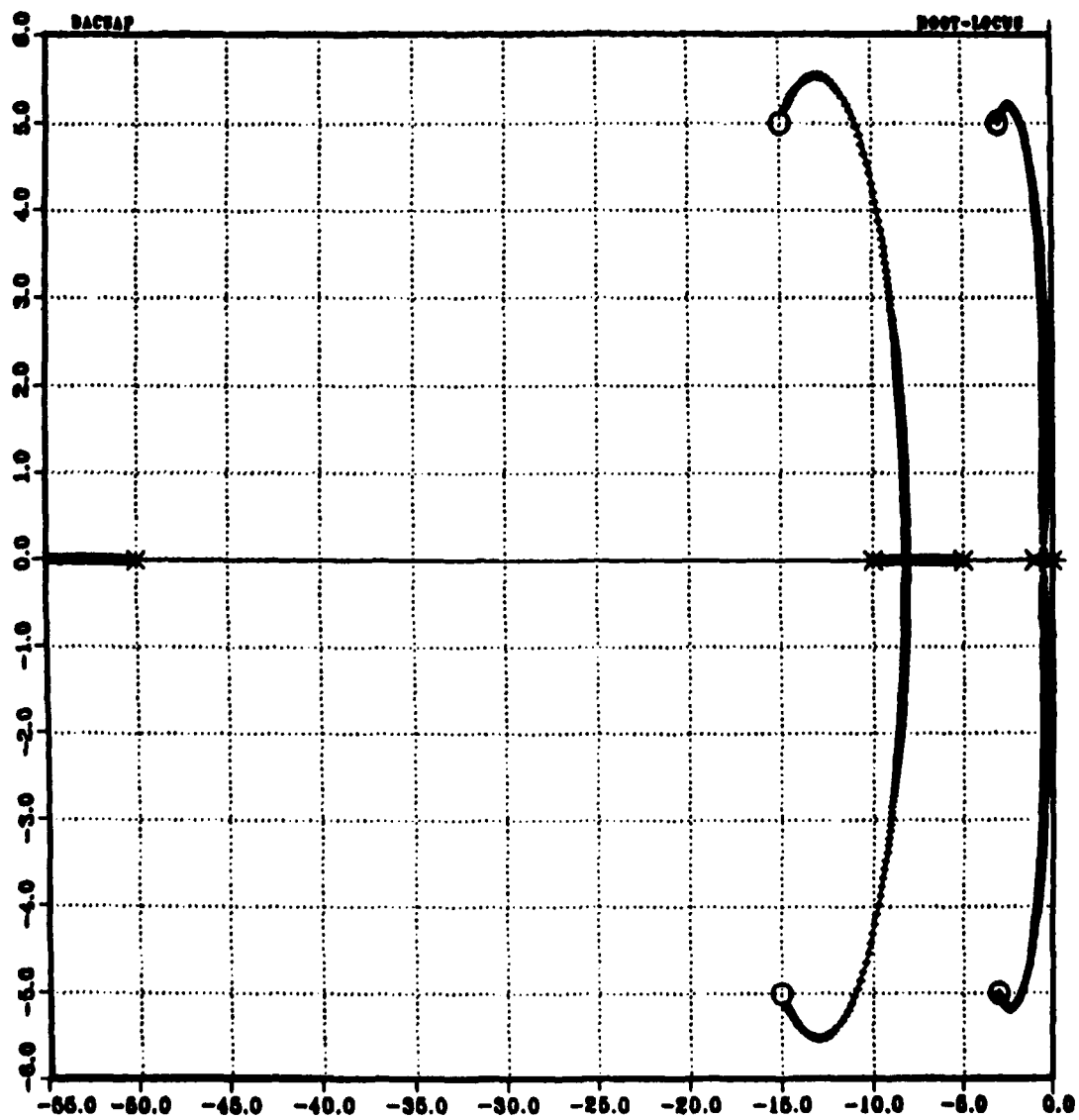
Figure 26. Root Locus of the Compensated System
