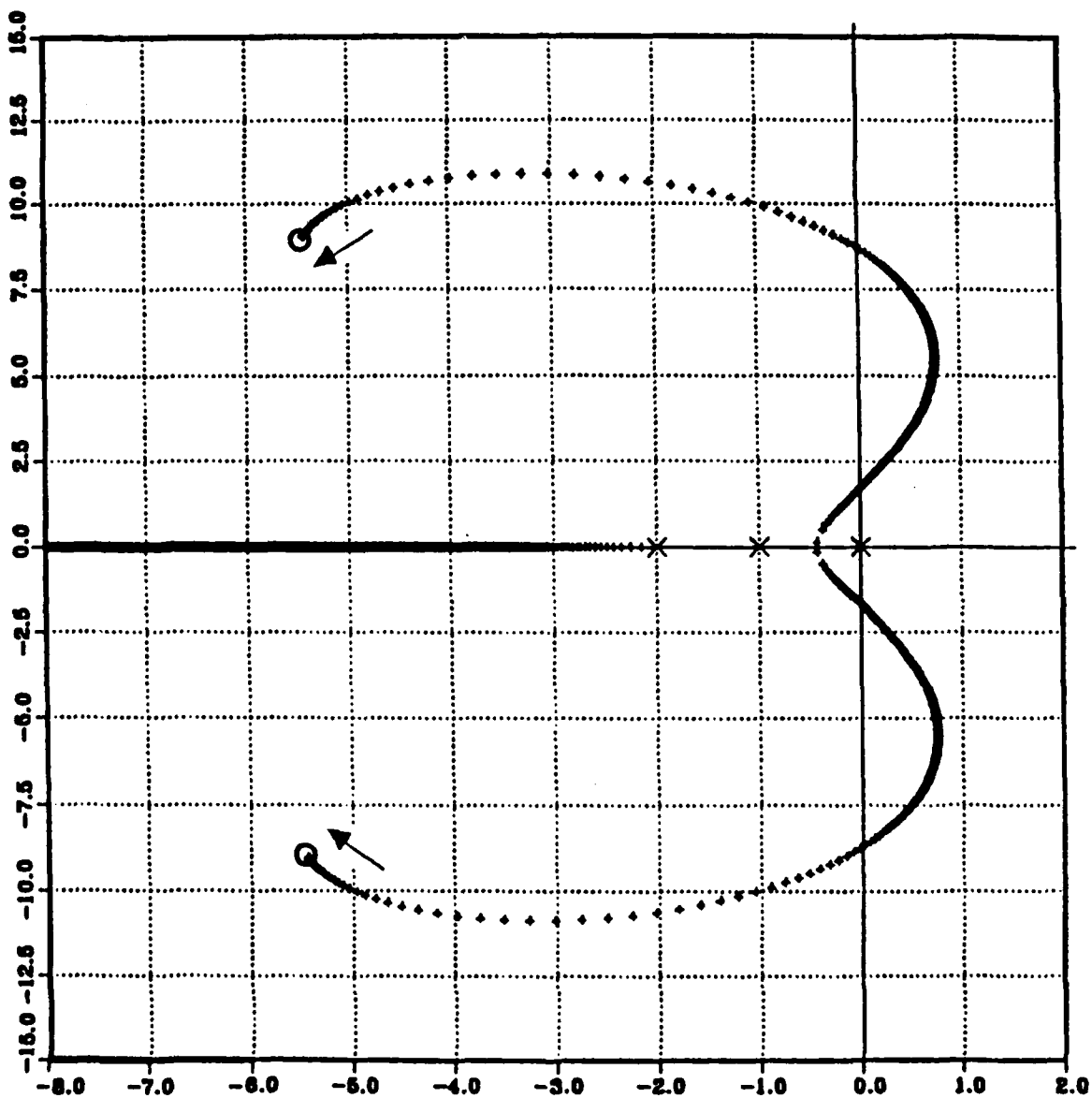
Figure 50. Offsetting Zeros by Matrix Methods. N-th Root at -50. Desired Roots; -5.000 \pm j10.000
