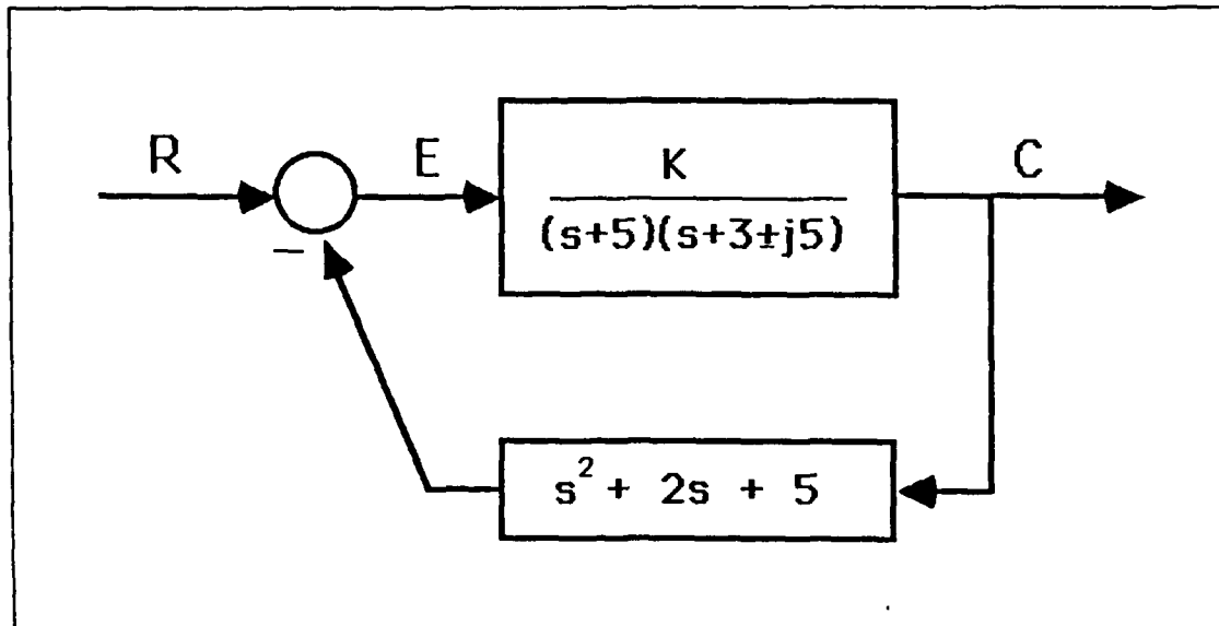
Figure 14. Basic State Feedback Block Diagram
