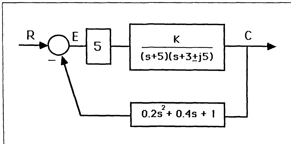
Figure 15. Unity Feedback Preservation
