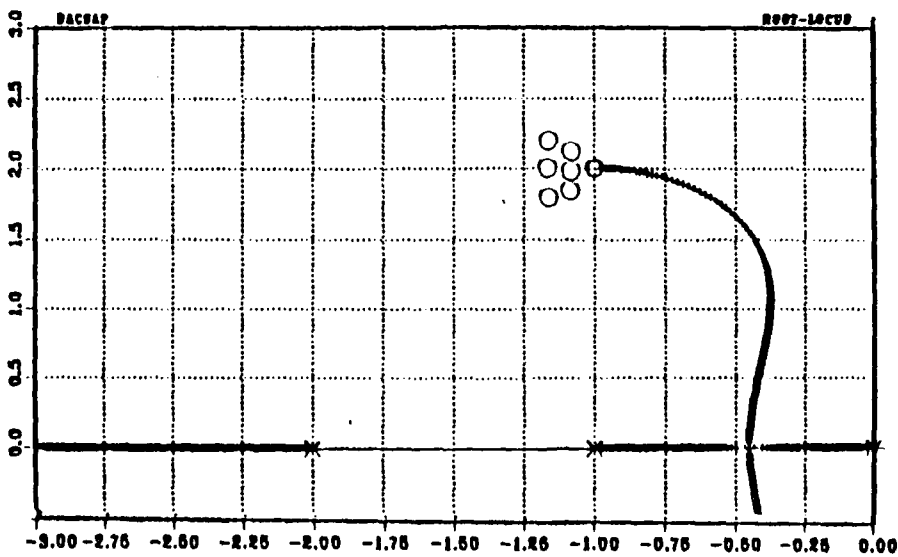
Figure 53. Arbitrarily Chosen Offset Zero Locations (II)
