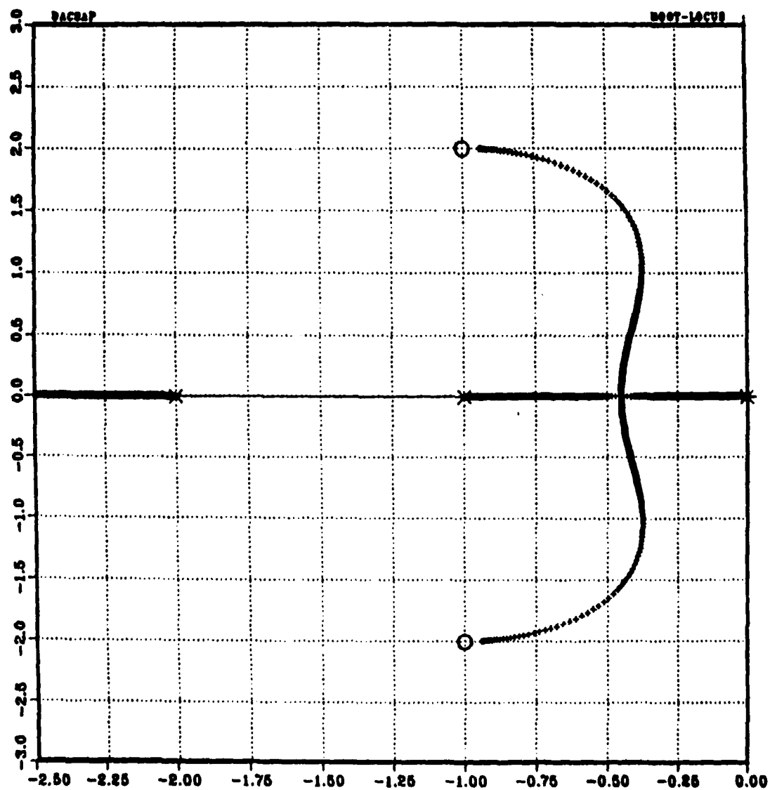
Figure 40. Compensated System Root Loci. Zeros at Location of Desired Roots; -1.000 \pm j2.000
