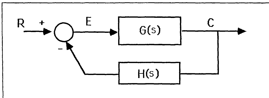
Figure 5. State Feedback Considered As A Function, H(s) .
