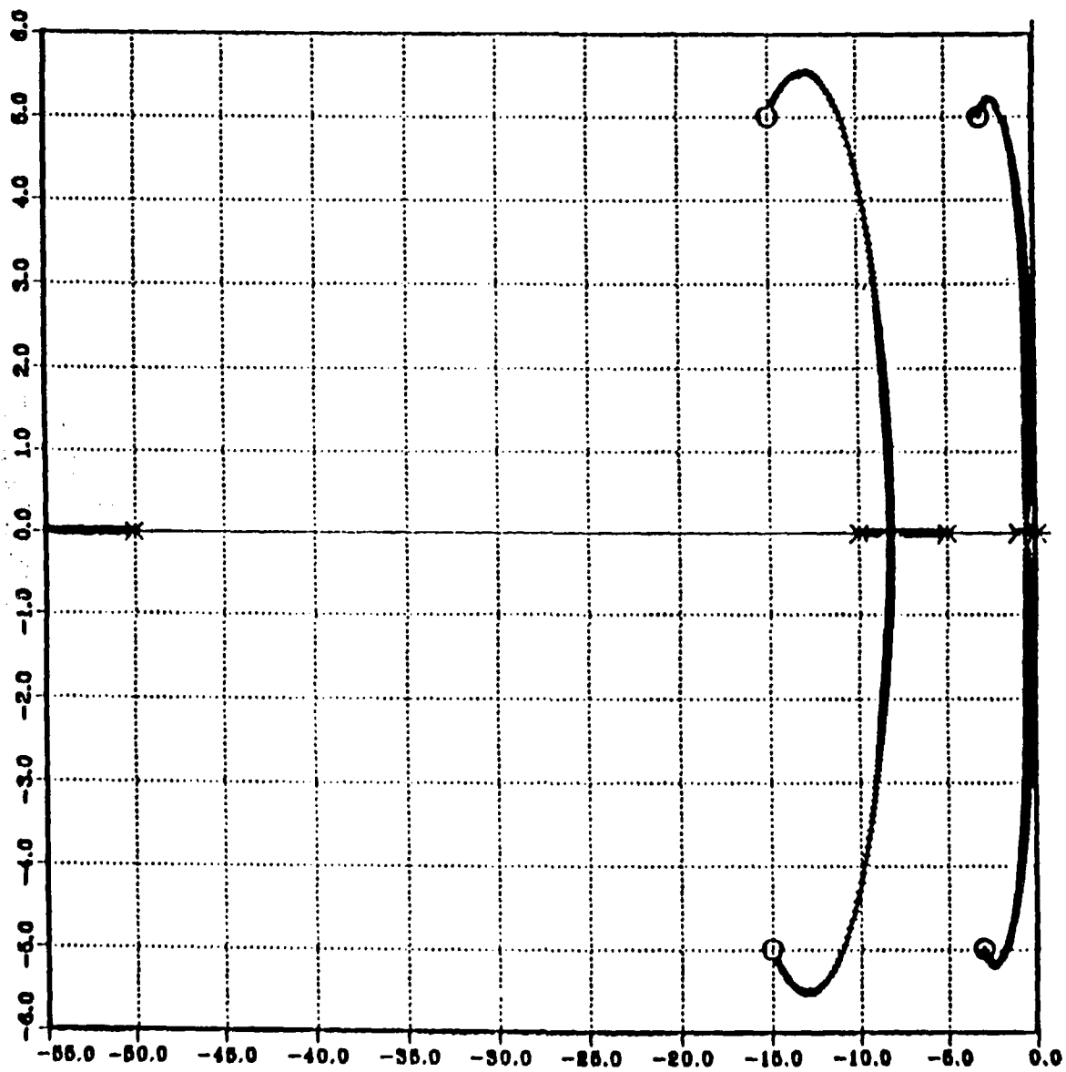
Figure 54. Original Compensated System Root Loci. Desired Roots; -3.000 \pm j5.000 , -15.000 \pm j5.000
