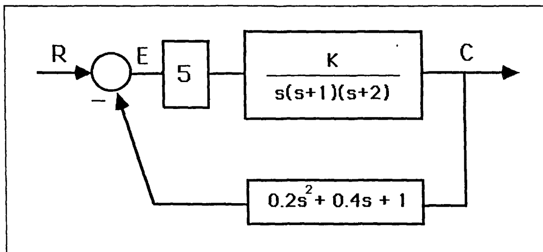
Figure 7. Unity Feedback Preservation
