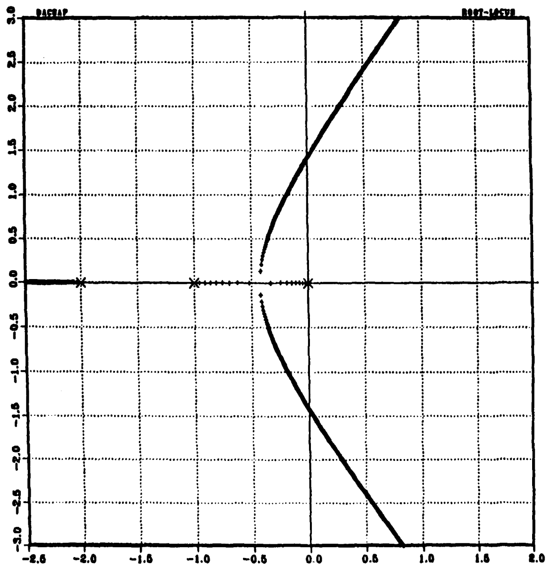
Figure 9. Root Locus of the Uncompensated System
