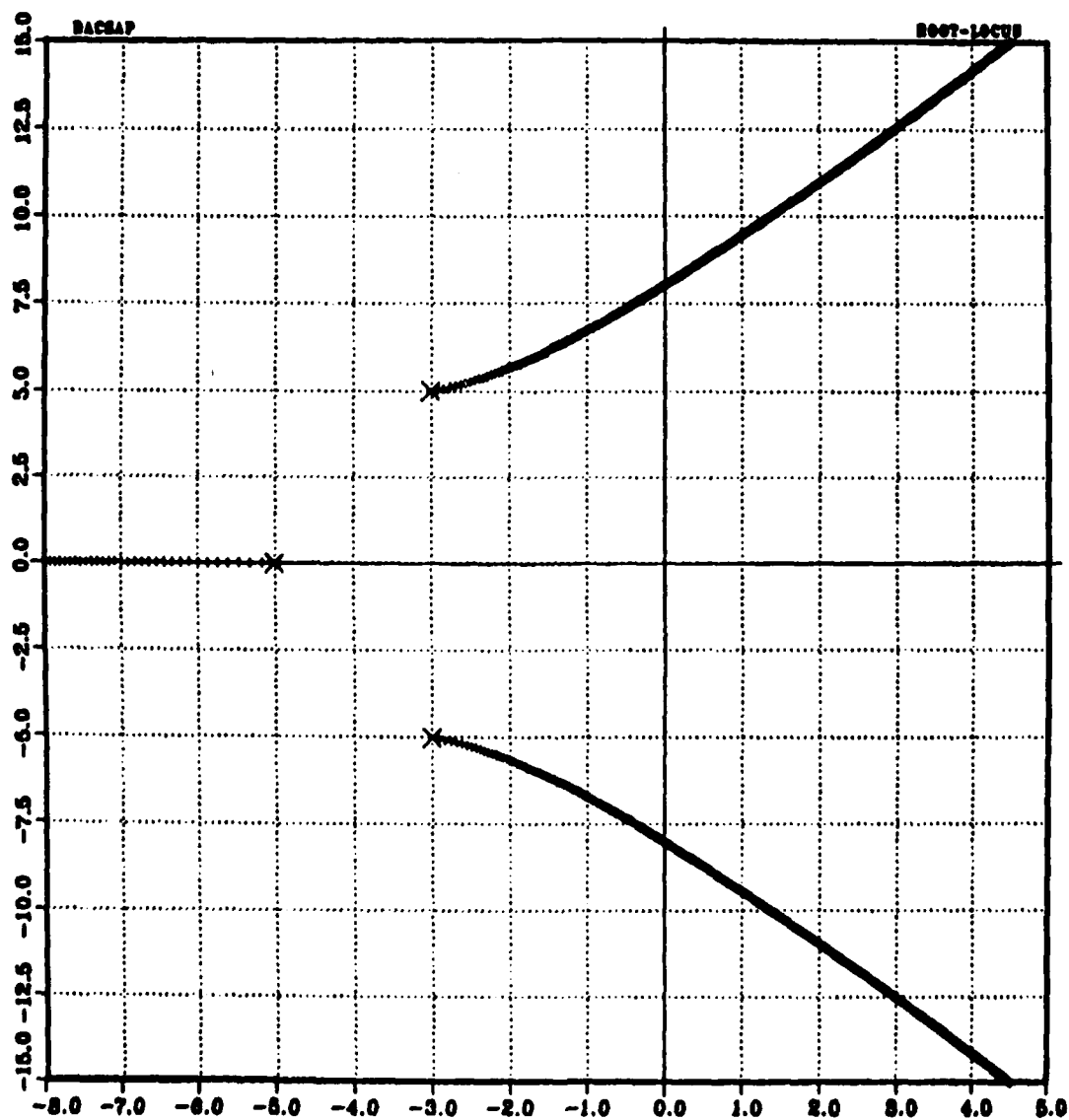
Figure 17. Root Locus of the Uncompensated System
