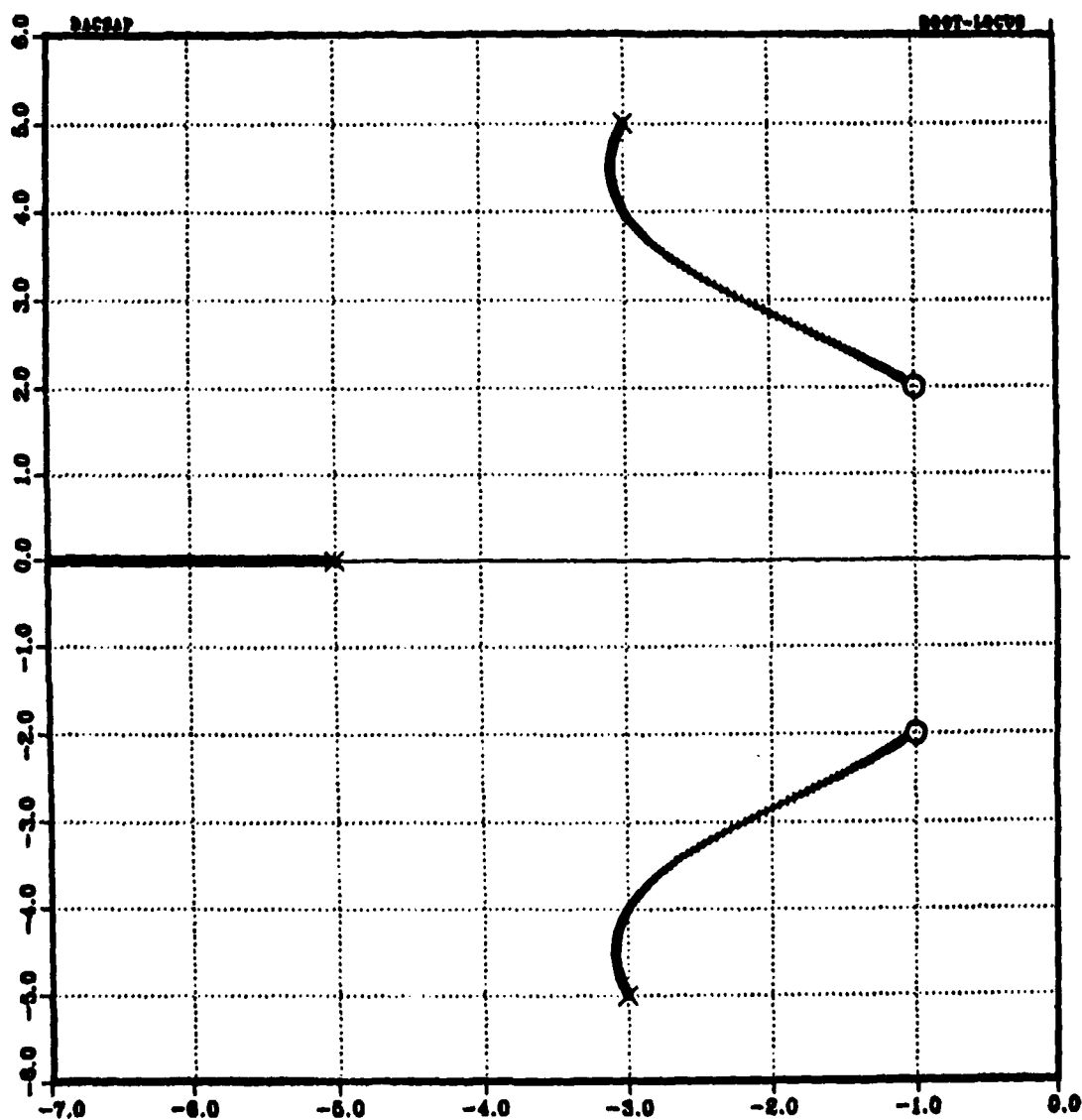
Figure 18. Root Locus of the Compensated System
