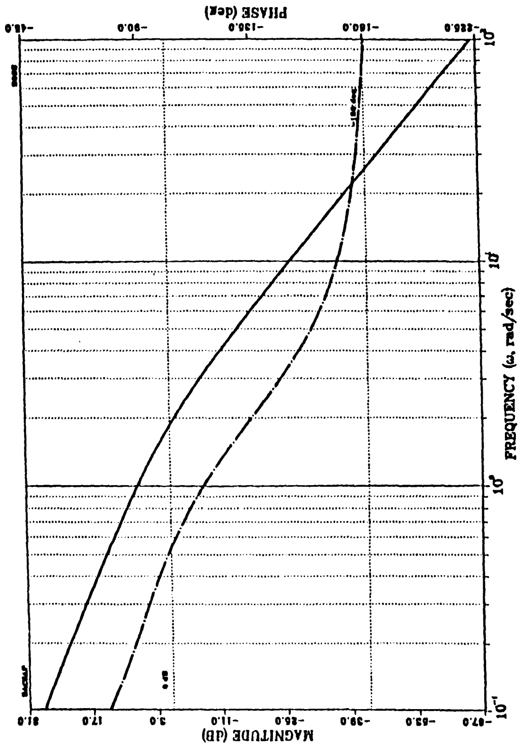
Figure 19. Compensated System Open Loop BODE Diagram
