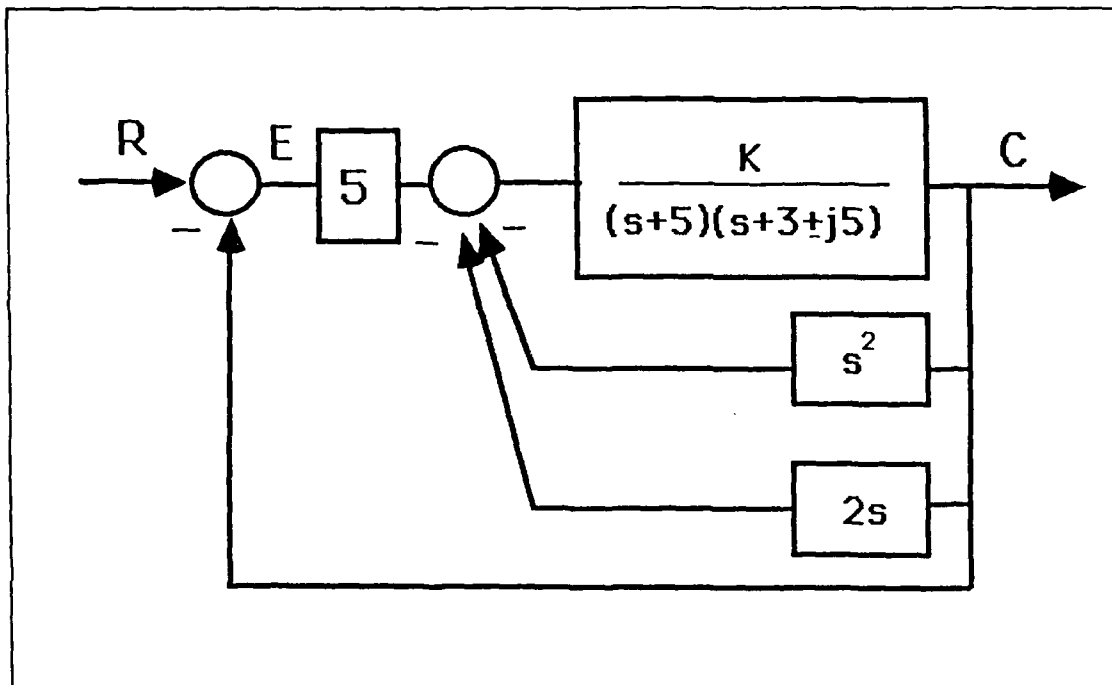
Figure 16. Rearranged Block Diagram
