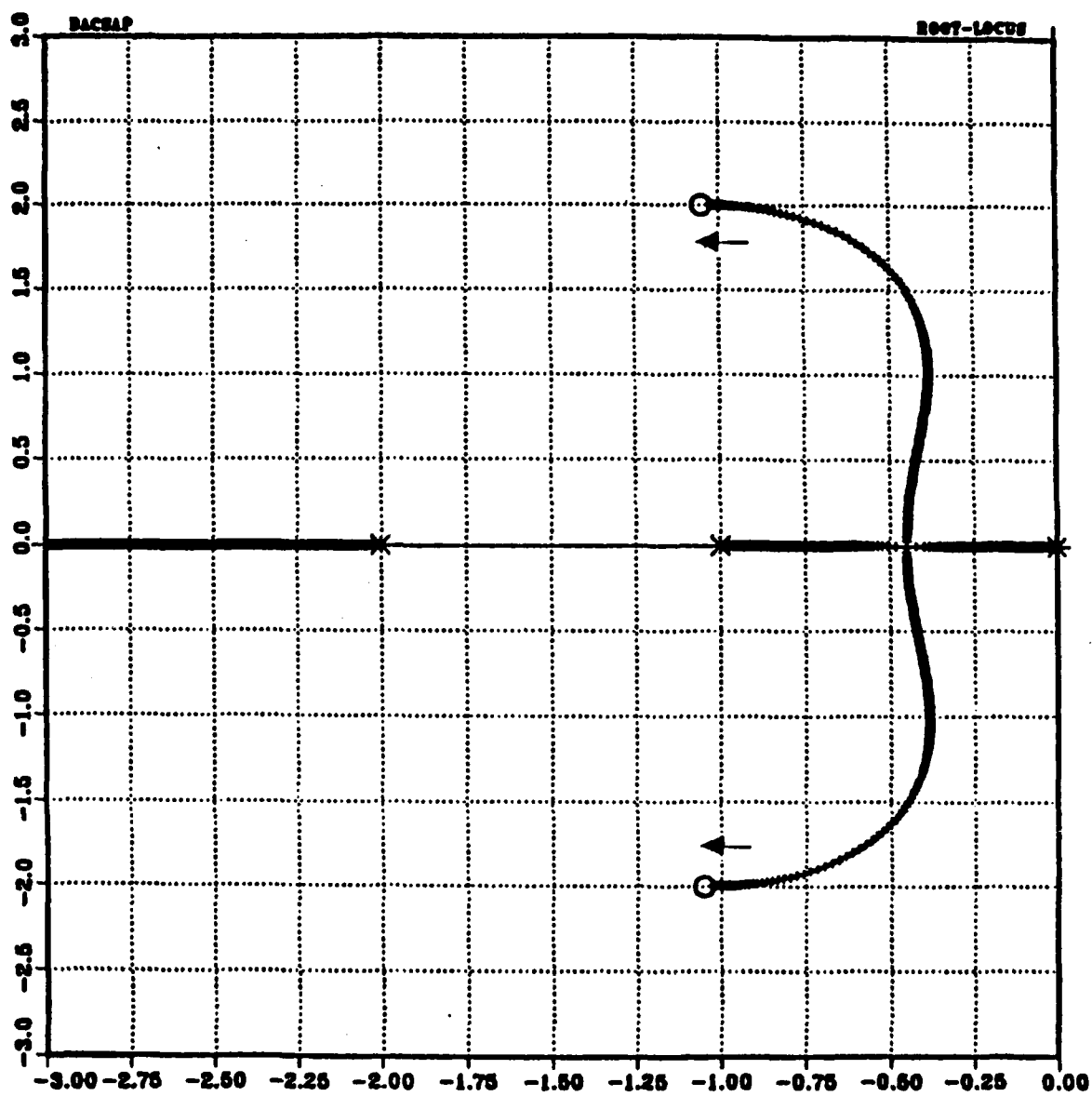
Figure 42. Offsetting Zeros by Matrix Methods. N-th Root at -50. Desire Roots; -1.000 \pm j2.000
