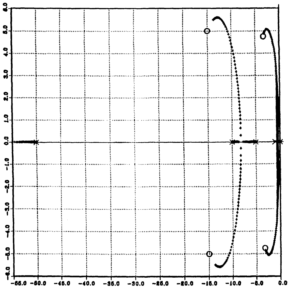
Figure 55. Offsetting The Zeros For The First Time. Desired Roots; -3.000 \pm j5.000 , -15.000 \pm j5.000
