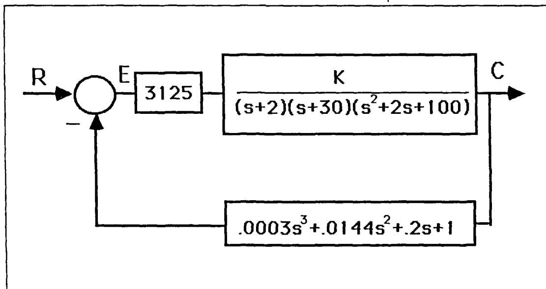
Figure 31. Unity Feedback Preservation
