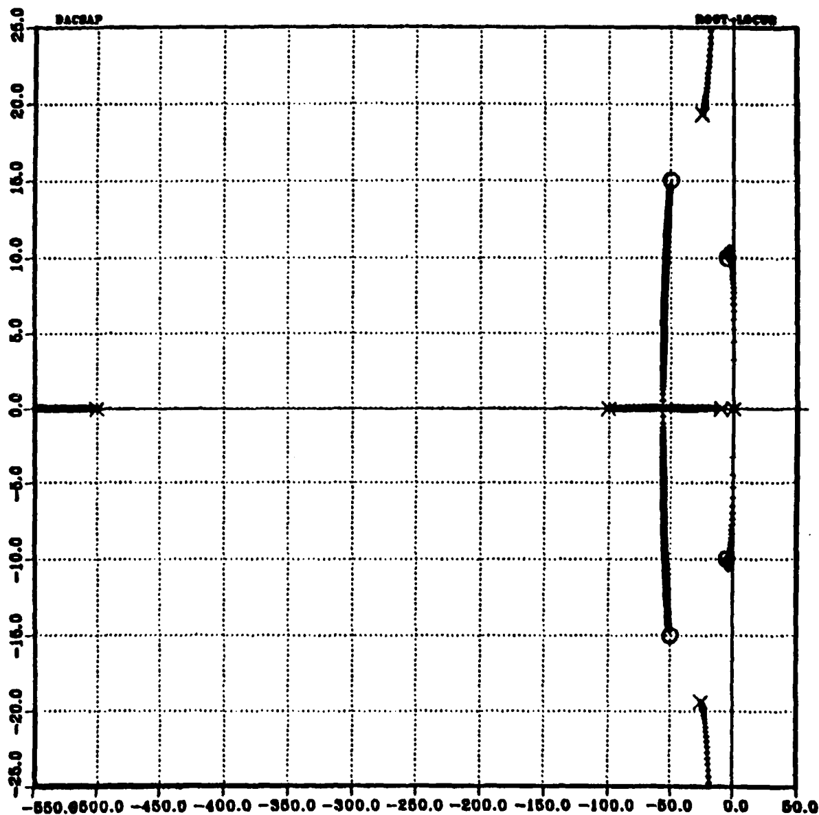
Figure 66. Offsetting The Zeros For The Third Time. Desired Roots; -5.000 \pm j10.000 , -50.000 \pm j15.900 , -300 \pm j200
