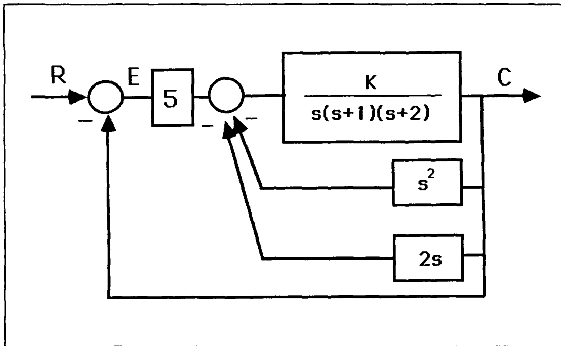
Figure 8. Rearranged Block Diagram
