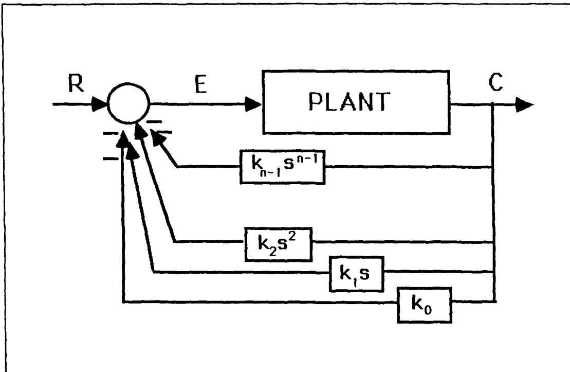
Figure 2. Basic State Feedback Block Diagram
