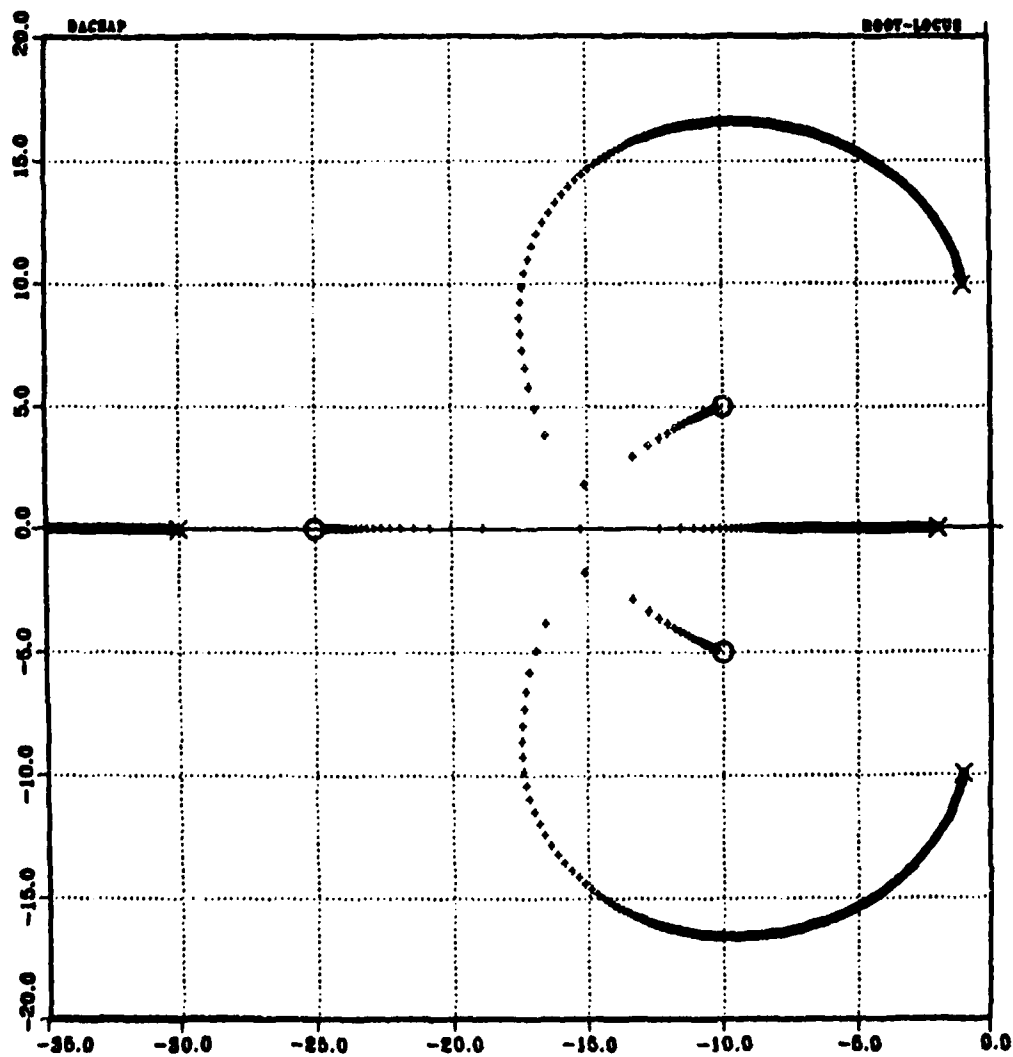
Figure 34. Root Locus of the Compensated System
