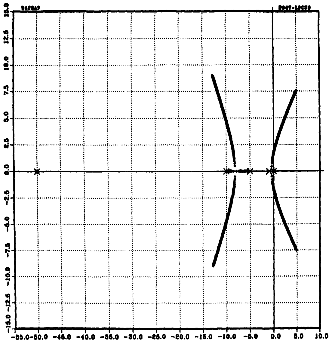
Figure 25. Root Locus of the Uncompensated System
