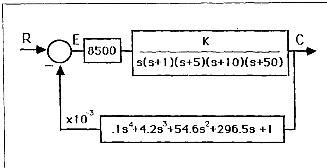
Figure 23. Unity Feedback Preservation
