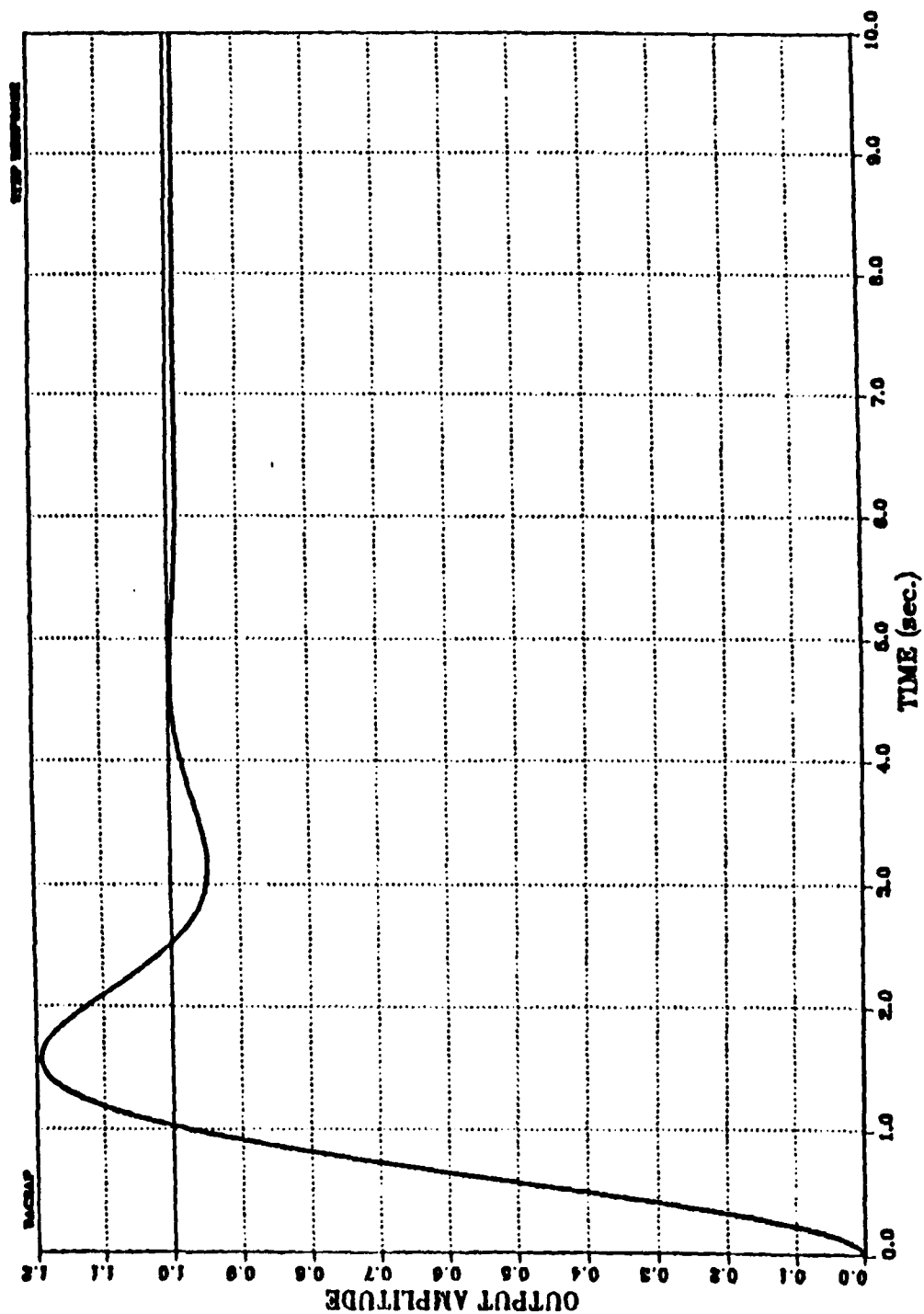
Figure 21. Step Response of the Compensated System
