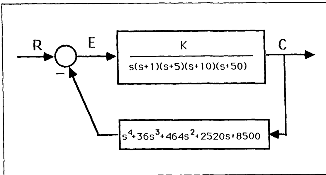
Figure 22. Basic State Feedback Block Diagram
