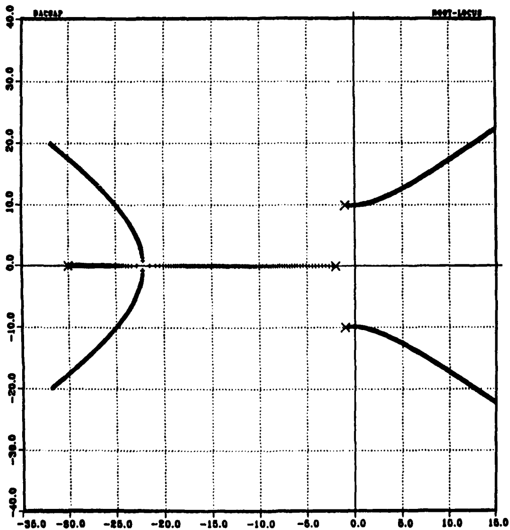
Figure 33. Root Locus of the Uncompensated System
