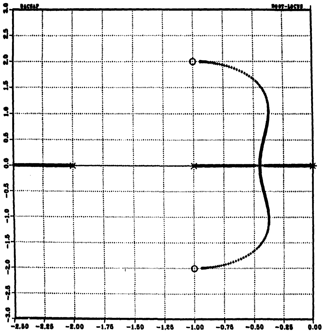
Figure 10. Root Locus of the Compensated System
