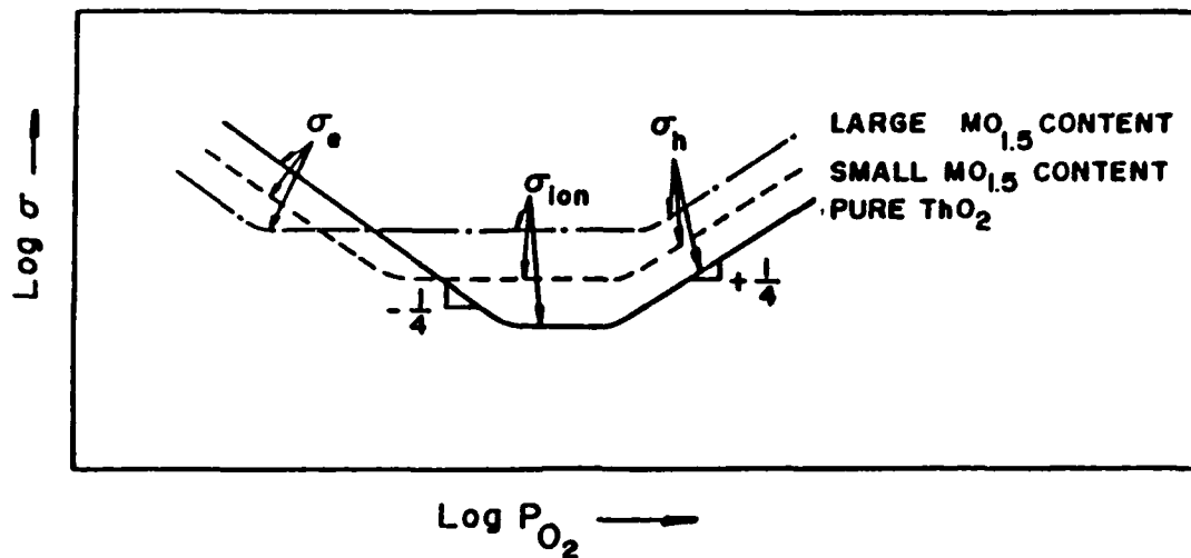
Figure 3. Schematic diagram of the variation of electrical conductivity of ThO_2 and ThO_2(Y_2O_3) solid solutions with oxygen pressure at constant temperature. Source: Ref. 9.
