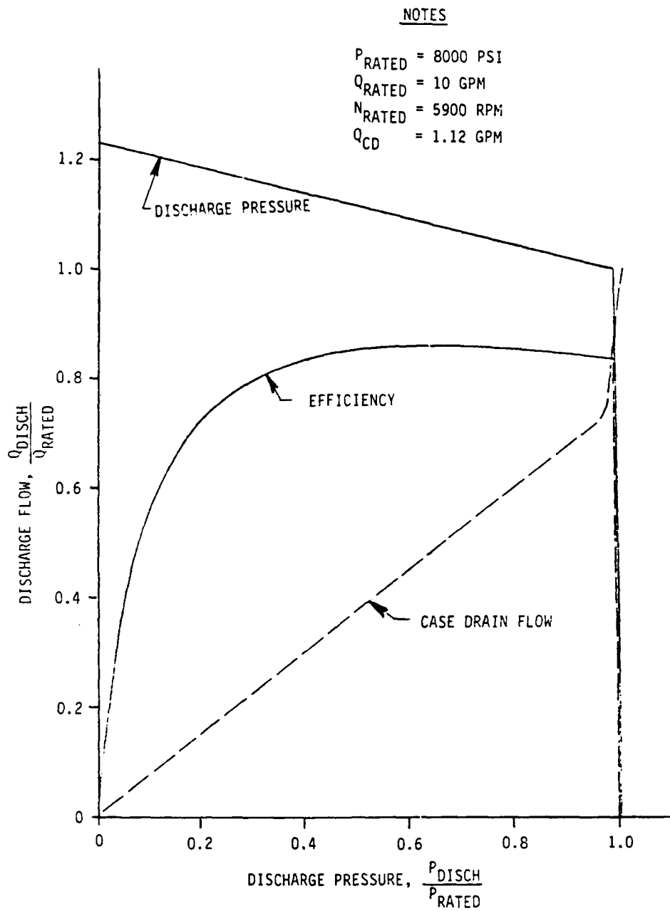
Figure B-22. Baseline pump performance characteristics
