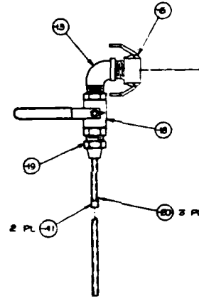
JET PROBE
