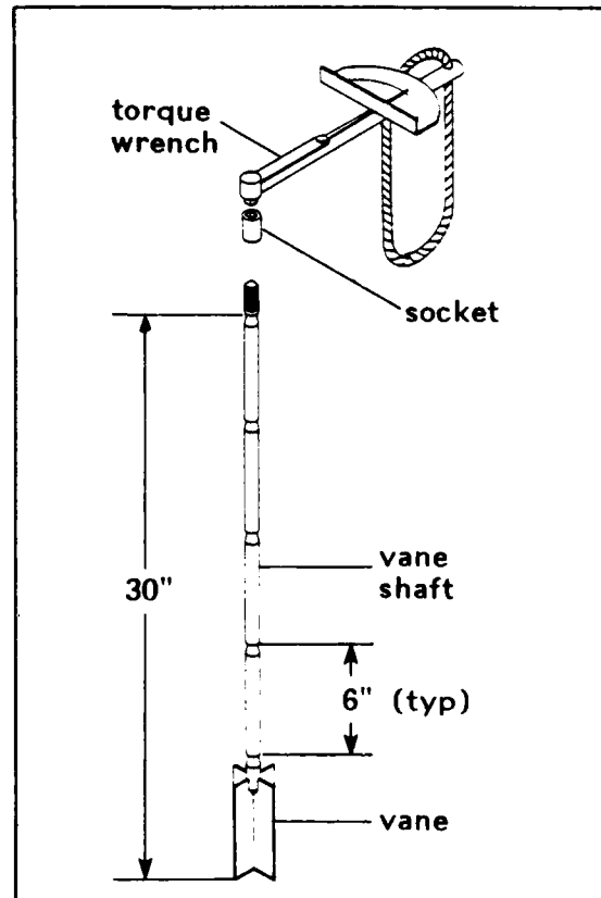
Figure 1.13. Vane shear.
