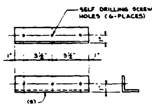
DETAIL G
