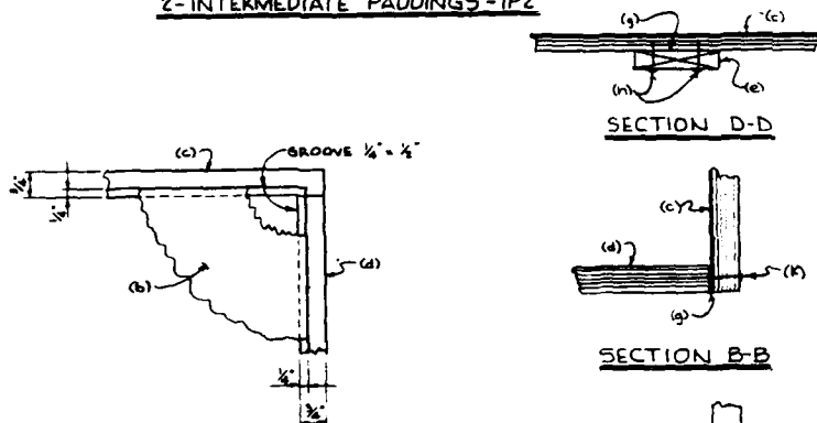
VIEW C-C
