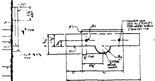
ONE-GROOVING TOOL (ASSEMBLY)-IT1
