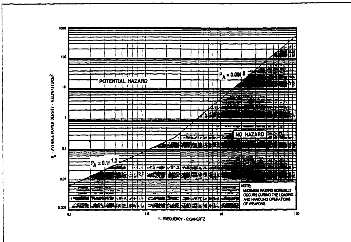
Figure 4. Weapons Requiring Restrictions - Radar frequencies
