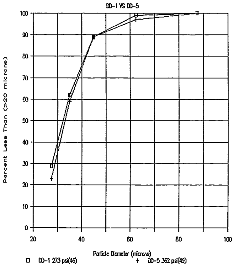
Figure 5.3 Particle Size Distribution for DD-1 and DD-5 Aft of the Propellant Grain
