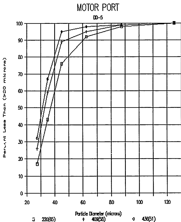
Figure 5.2 Particle Size Distribution for DD-5 in Motor Port
