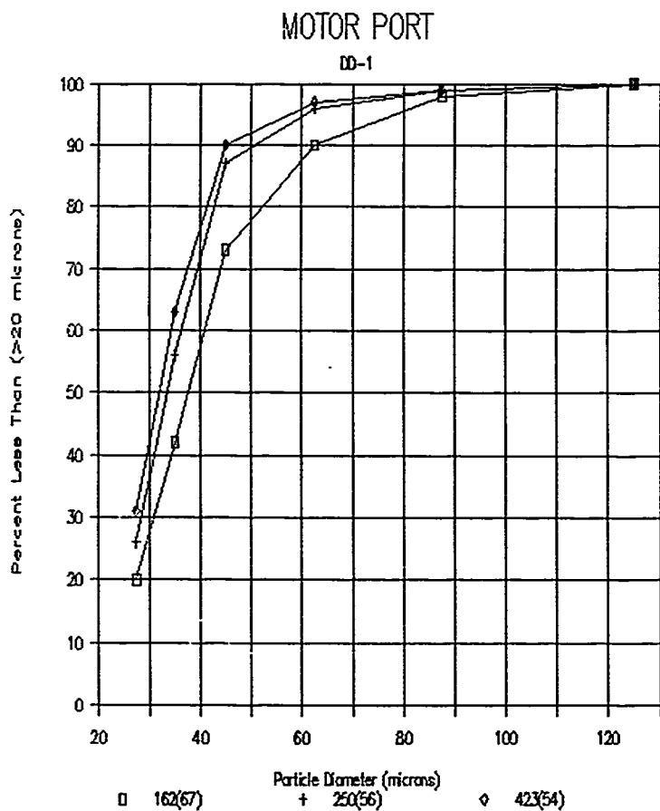
Figure 5.1 Particle Size Distribution for DD-1 in Motor Port
