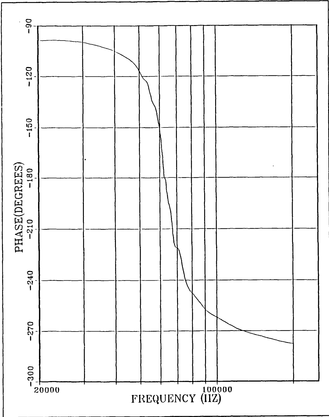
Figure 15. Single Stage Bandpass Filter Phase Response
