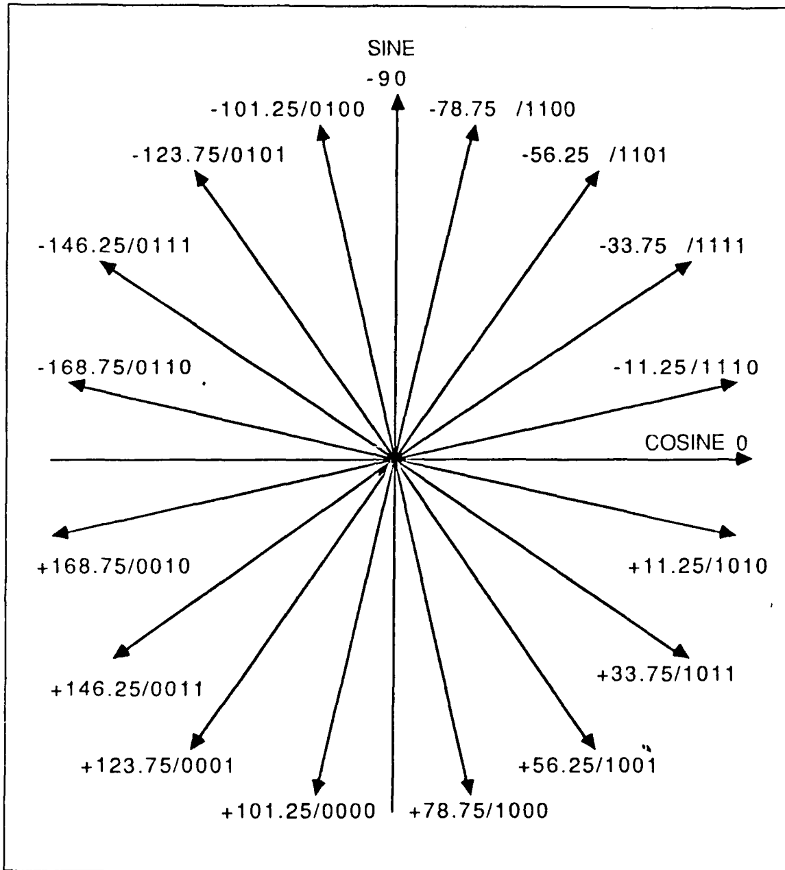
Figure 2. Off-Set 16-PSK Signal Constellation
