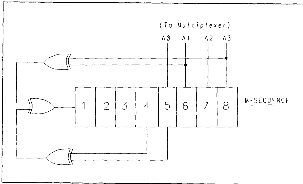
Figure 8. Block Diagram of (4,5,6,8) Feedback Shift Register
