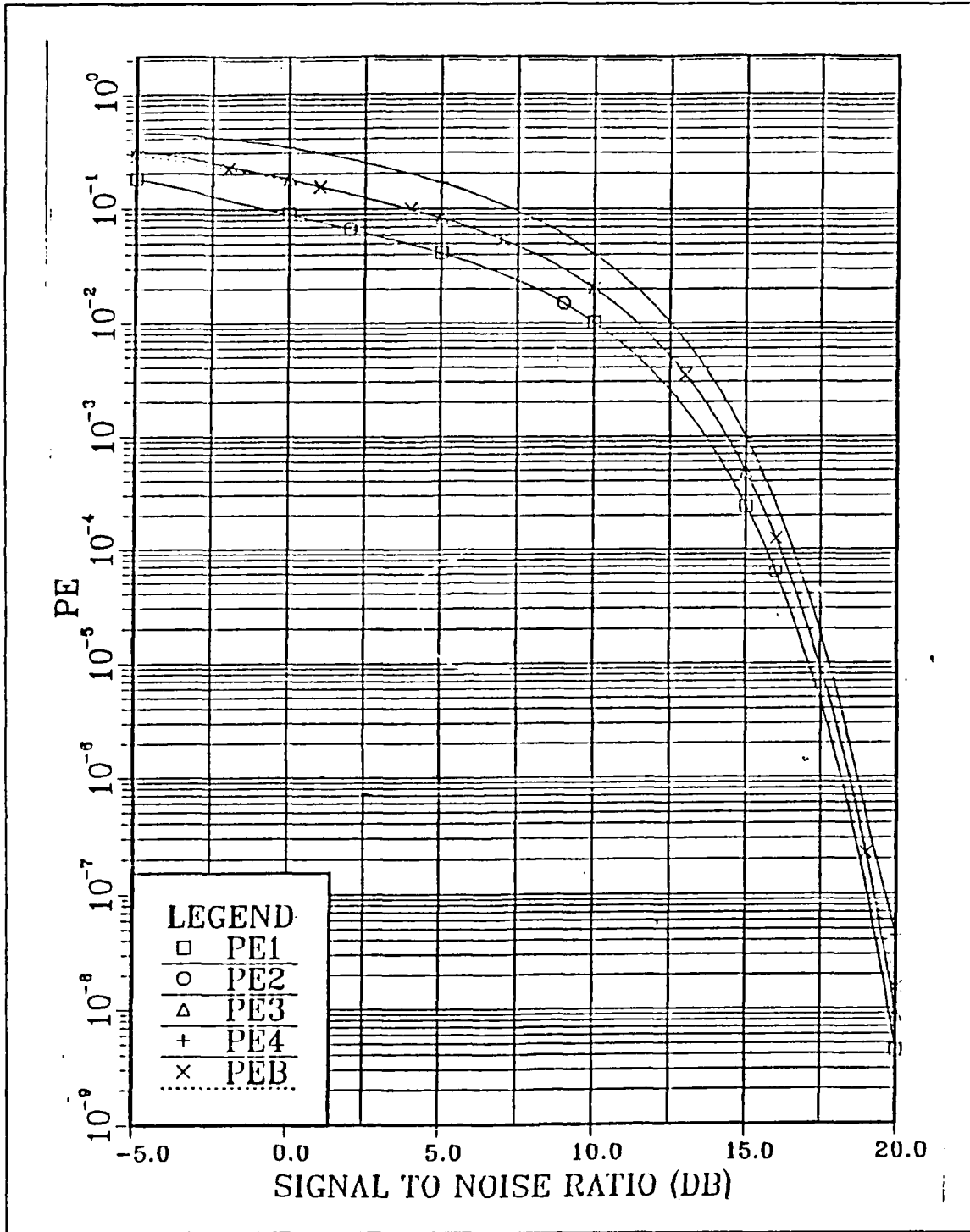
Figure 31. Theoretical Performance of 16-PSK DBD Receiver
