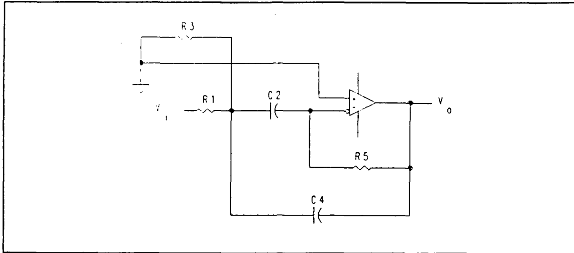
Figure 6. Active Bandpass Filter
