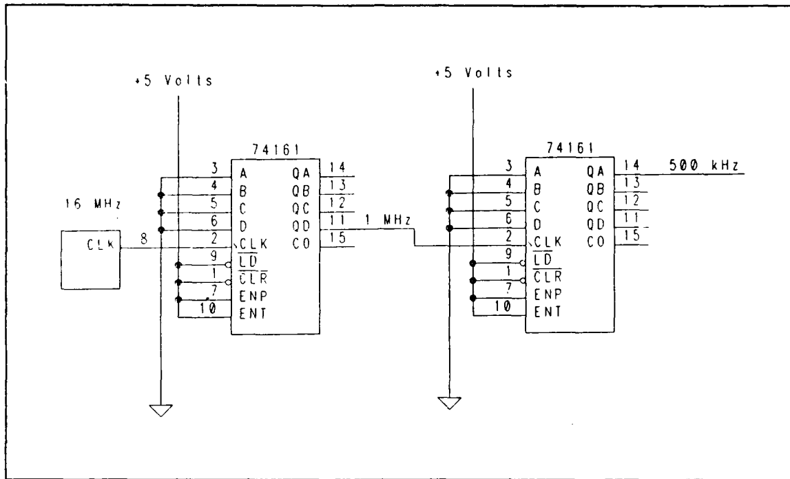
Figure 10. Implementation of System Clock
