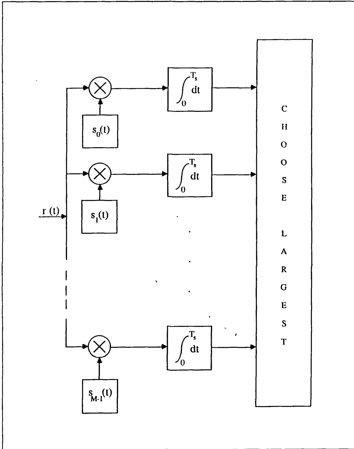
Figure 29. M-PSK Symbol Detection Receiver
