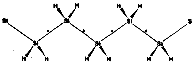
Figure 47.1 Sketch of the polysilane chain. 7 Conformational energies are calculated as a function of the rotation angles about skeletal bonds b and c .
