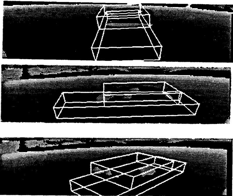
Figure 6-1: Object recognition
