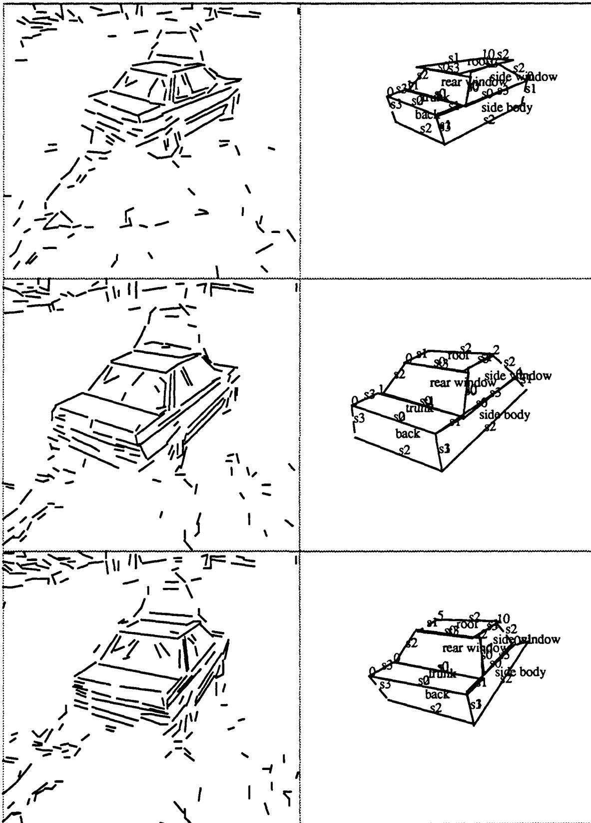
Figure 4-4: Original lines and verified matches from another three images
