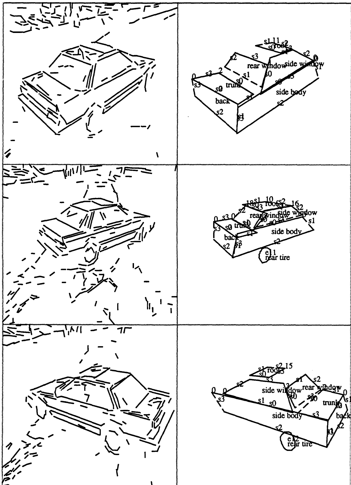
Figure 4-5: Original lines and verified matches from the final three images
