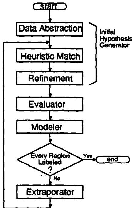
Figure 36: Context control
