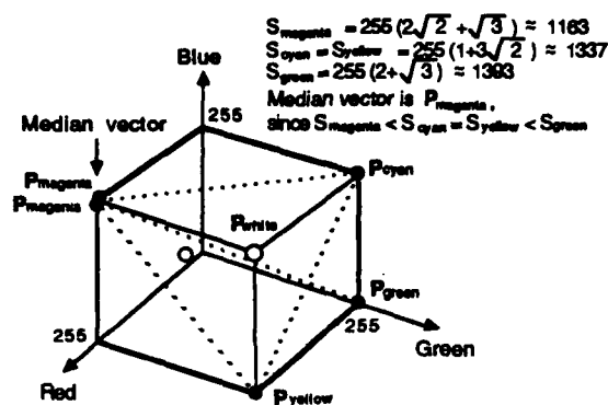
Figure 47: Vector median in three dimensional space
