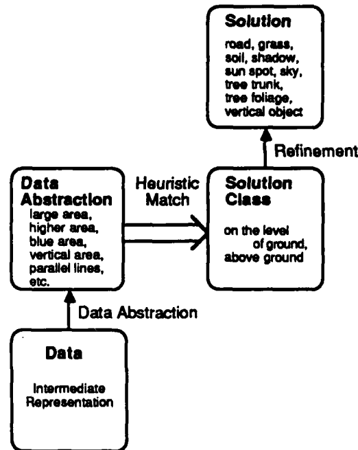
Figure 31: Classification problem solving model applied to initial hypothesis generator
