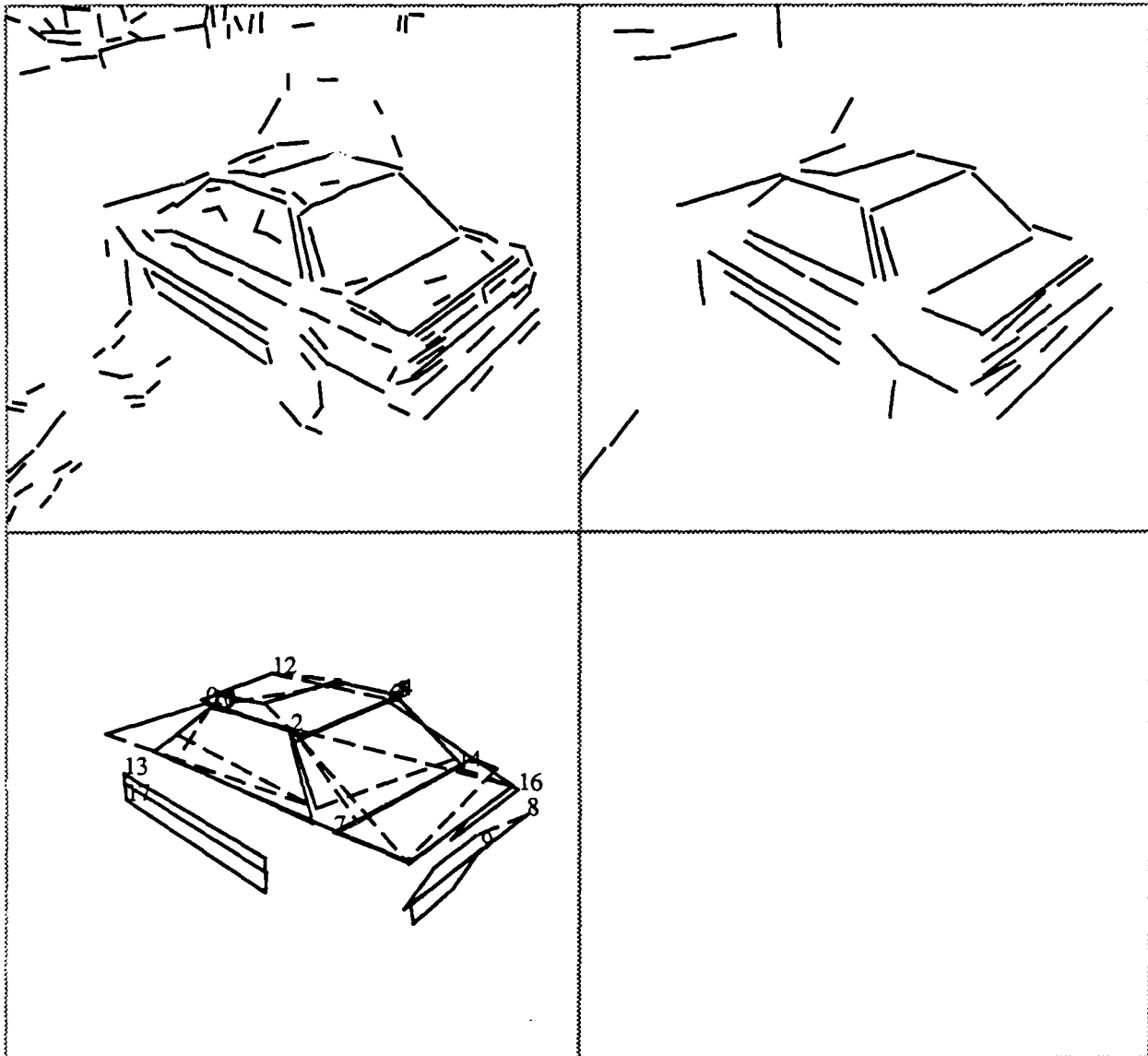
Figure 4-2: Second image: original lines, merged and thresholded lines, and extracted trapezoids
