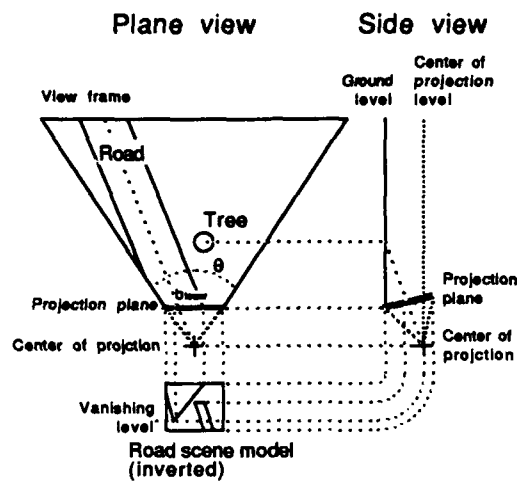
Figure 42: Inverse projection
