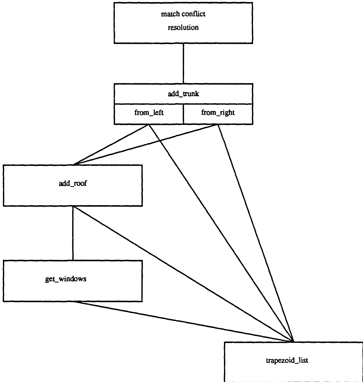
Figure 3-4: Hierarchy of search procedures
