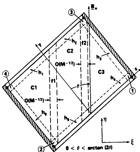
FIG. 10. Subregions in magnetohydrodynamic channel flow at high external magnetic fields
