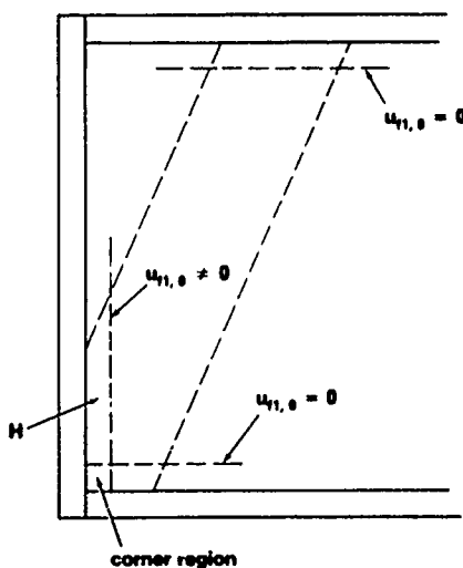
FIG. 11. Hartmann layer adjacent to free shear layer f1 . The O(M^{1/2}) free shear layer velocity u_{f1,0} is zero at t = \sec \theta for all \zeta and at t = 0 for \zeta > 0 . There are no O(M^{1/2}) velocities in the Hartmann layers between the free shear layer and the perfect conductors, so that P_{T\mu} = O(M^{1/2}) in these layers.
