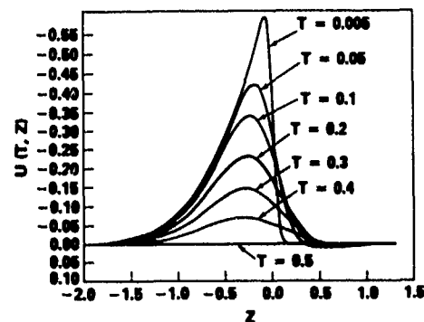
FIG. 9. Rescaled free shear layer velocity profiles U(T, Z) .
