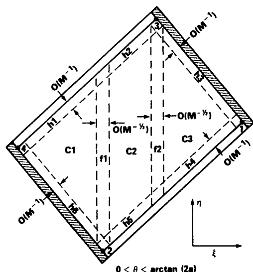
FIG. 3. Subregions in magnetohydrodynamic channel at high external magnetic fields
