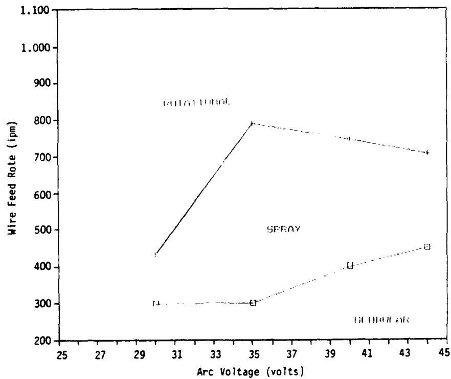
Figure 18. Metal transfer regions for 95% Ar/5% O 2 (TIME torch, 3/4" stickout).
