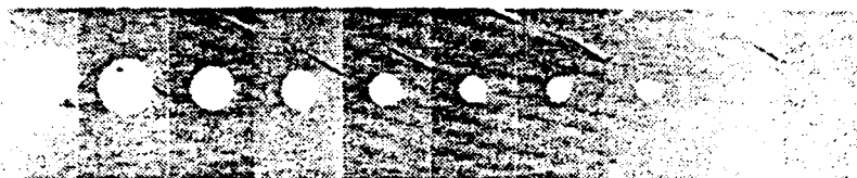
Figure 18. Experimental underwater photographs of a 2-foot-diameter white disc taken at ranges of from 30 feet (left) to 120 feet (right) with the light source 30 feet behind the camera.
