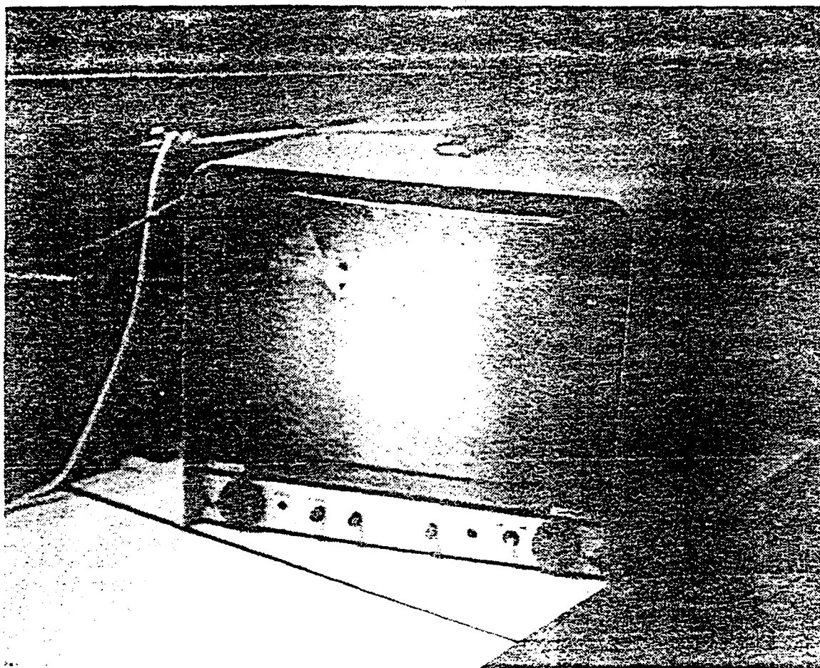
Figure 40. Shipboard monitor, showing a compass hanging 3 m below the television camera in 3600 m of water over a silting ocean bottom
