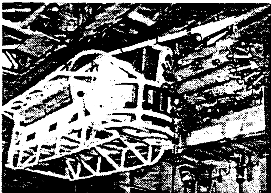
Figure 12. NRL's renowned deep-towed "fish" became a combined search and sampling vehicle with the addition of a multiple water sampler, seen here attached to the aft end of the fish. Signals telemetered down the towing cable activated the water sampler when other sensors on the "fish" indicated that the hulk containing the chemical-warfare munitions was nearby.
