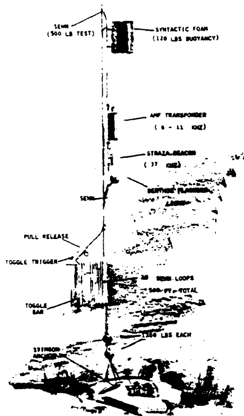
Attachments at bottom end of line that lifted Alvin to the surface. By means of Mizar's underwater tracking instruments, NRL personnel positioned this equipment within 250 feet of the submersible.
