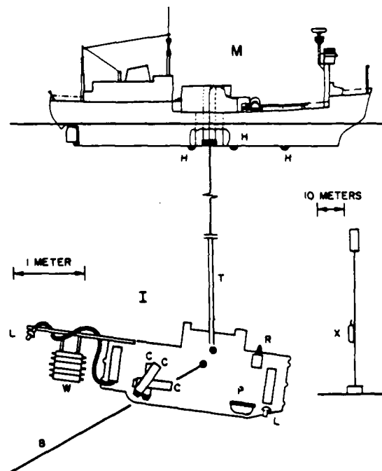
Figure 40. NRL's ability to investigate the abyss stems from elements in the system illustrated above. From the surface platform Mizar (M), the instrumented platform (I) is lowered through a well by electrical tow cable (T) to a position above the sea floor, which is monitored by acoustic pinger (P). Electronic flash lamps (L) provide light for cameras (C) which photograph the ocean bottom and instruments, such as the water sampler (W) and bottom dredge or trawl sampler (shown in photograph), which is tethered to the towed platform by bridle (B). Precise acoustic navigation is provided by the anchored reference transponder (X), the responder (R), and Mizar 's hull hydrophones (H). The entire system is controlled from a laboratory aboard Mizar . Note difference in scale between the instrumented platform and the remainder of the illustration.
