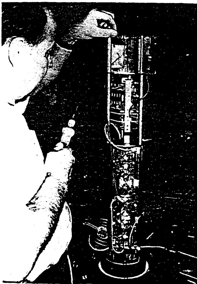
Figure 39. Underwater television electronics, showing filters, carrier generator, modulation device, and line driver; configured for insertion into a pressure-resistant housing
