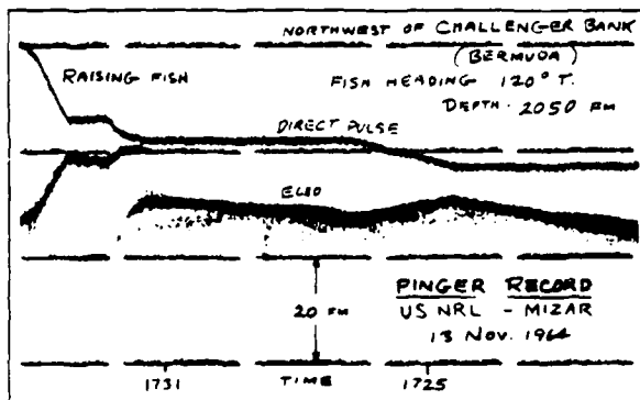
Figure 11 Pinger Record
