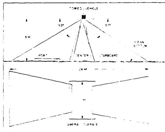
Figure 5. Camera Coverage
