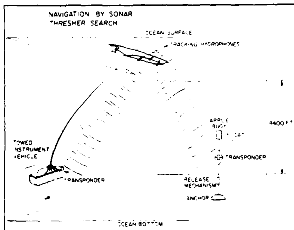
Figure 7. Acoustic Navigation System
