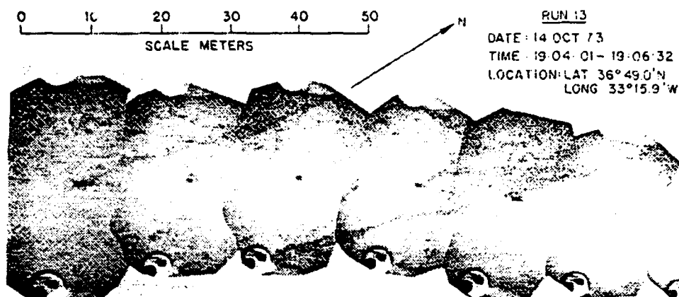
Figure 2. The two dark lines in this montage of seven LIBEC photographs are vertical openings or fissures which parallel the sides of the median Rift Valley in the Mid-Atlantic Ridge.
