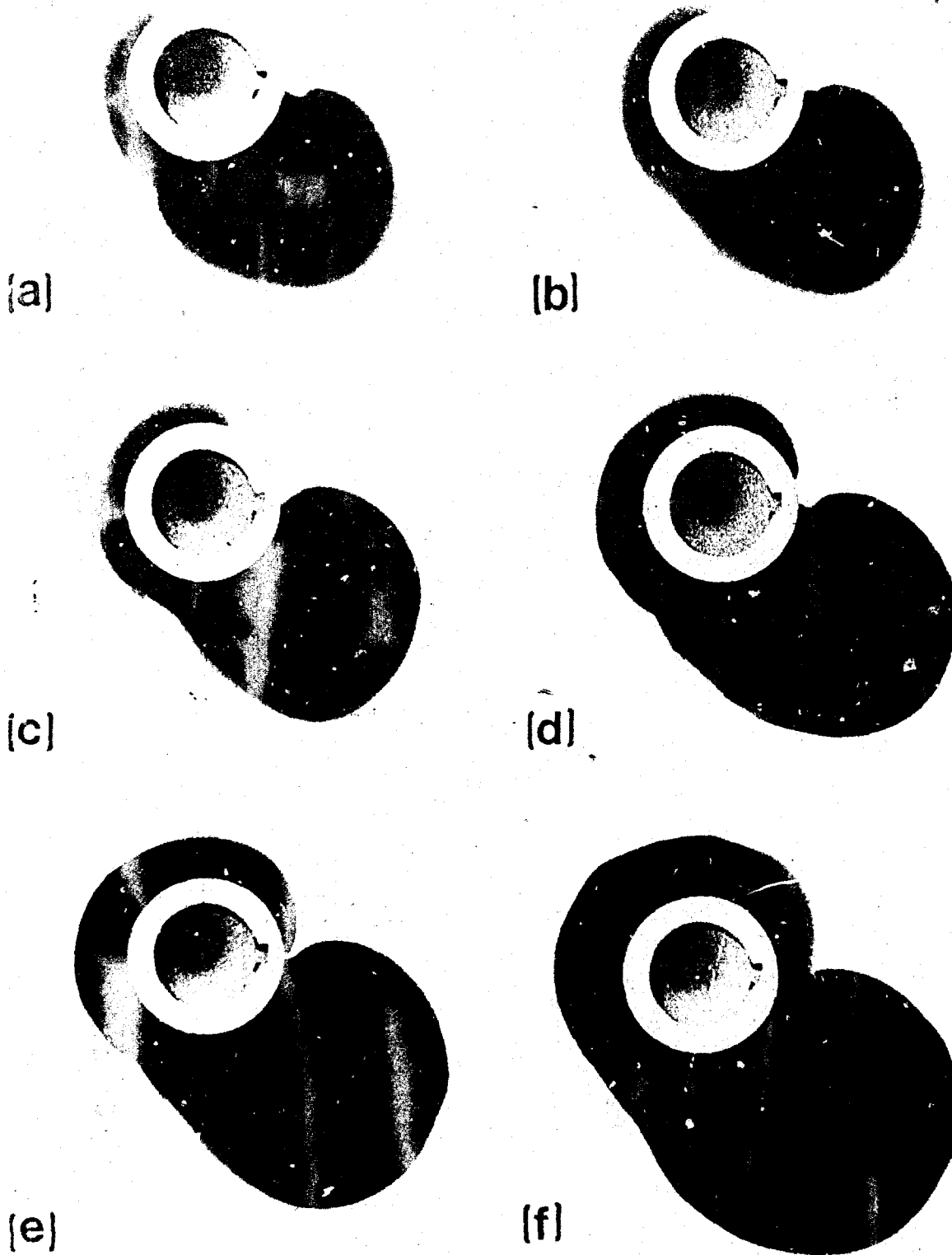
FIG. 9. Subsequent photographs of a (laboratory-generated) lens-like eddy responding to the presence of a solid cylinder. The sequence shows the structure of the eddy and the intrusion during the various stages of the interaction. Physical constants f = 3.35 \text{ s}^{-1} , \Delta\rho/\rho = 1.0052 ; T = 21.5^\circ\text{C} . The process shown in (a-f) lasted for about 20 seconds; the diameter of the cylinder is 5 cm. Note that, (i) a padlock flow is indeed established, as predicted by the theory, (ii) the eddy does not rotate around the cylinder, (iii) the lens remains roughly circular as assumed in the development of the theory, and (iv) during the interaction the eddy grows in time because of the continuous injection of dyed salty water through the bottom (see text).
