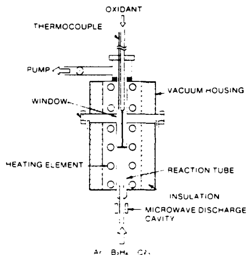
Fig. 1. Schematic of the HTFFR.
