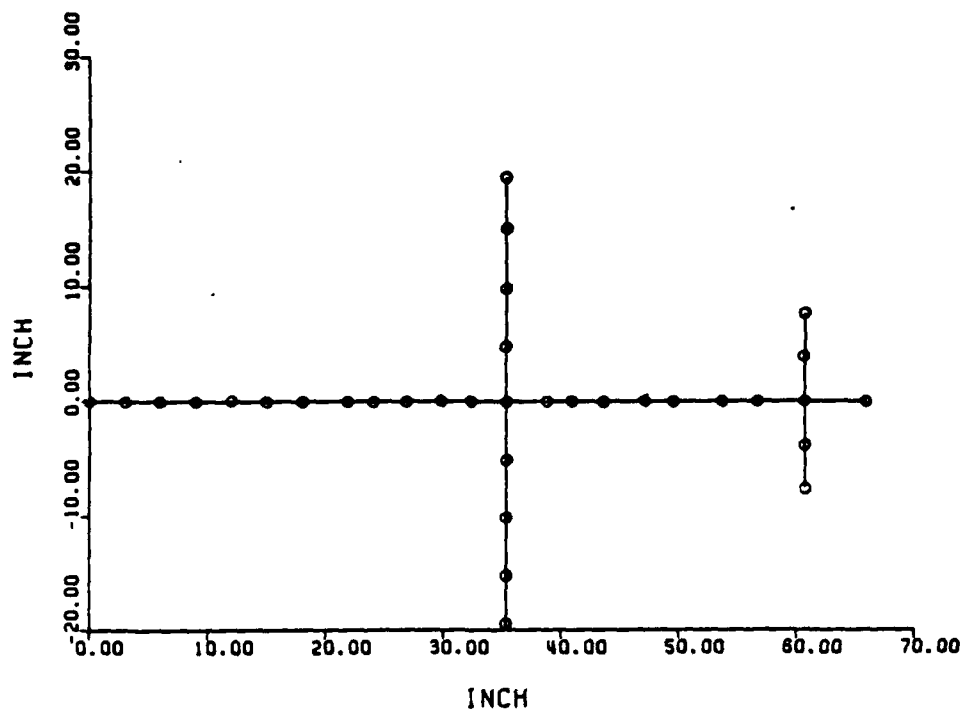
Figure 9. NASTRAN beam model.
