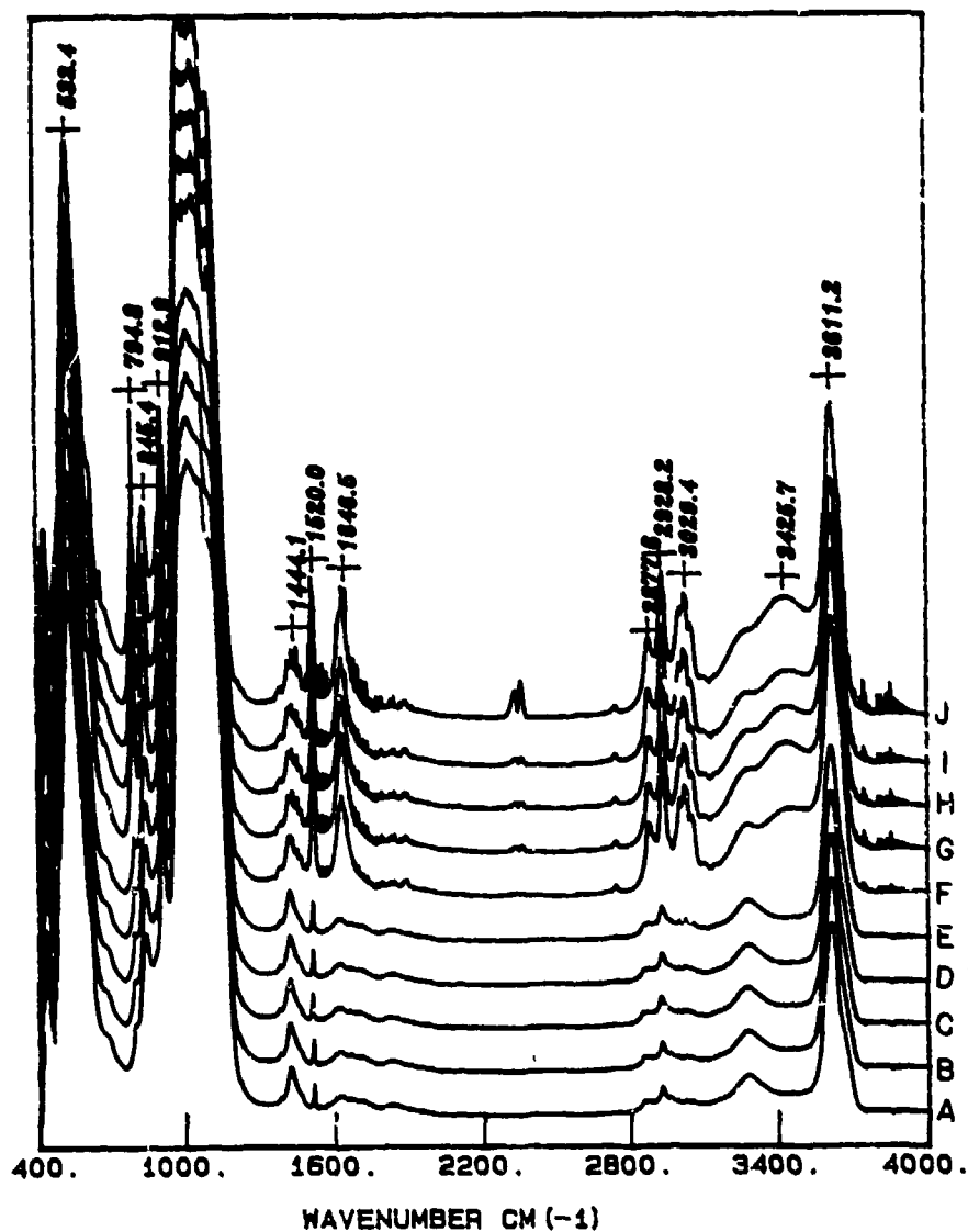
Figure 73. Controlled Desorption Spectra of the p-Xylene: Na-SAz-1 Complex in the 400-4000 \text{cm}^{-1} Region. See Text for Complete Description.
