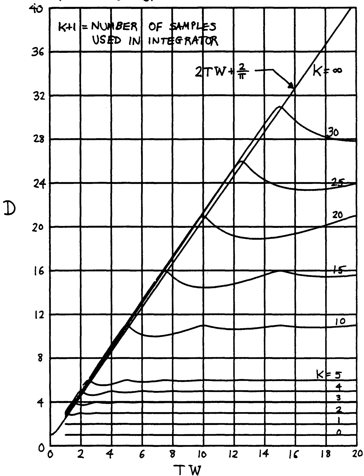
EQUIVALENT DEGREES OF FREEDOM D VERSUS SEARCH AREA TW
