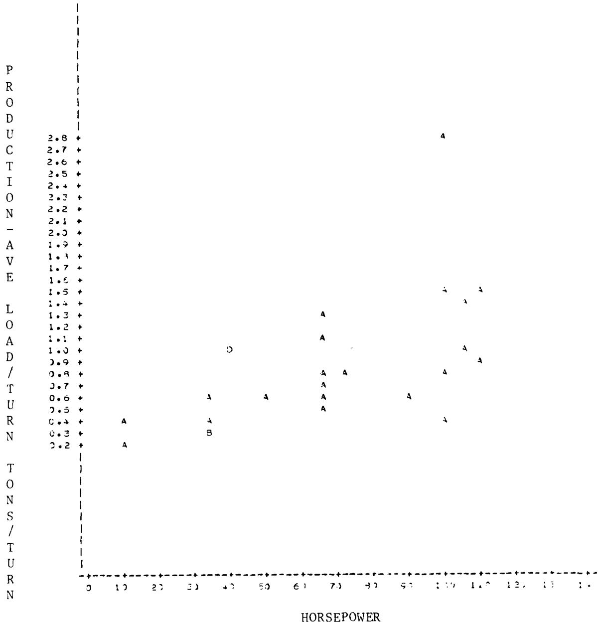
FIGURE 4. PLOT OF AVE. LOAD PER TURN VS. CABLE YARDER HORSEPOWER
