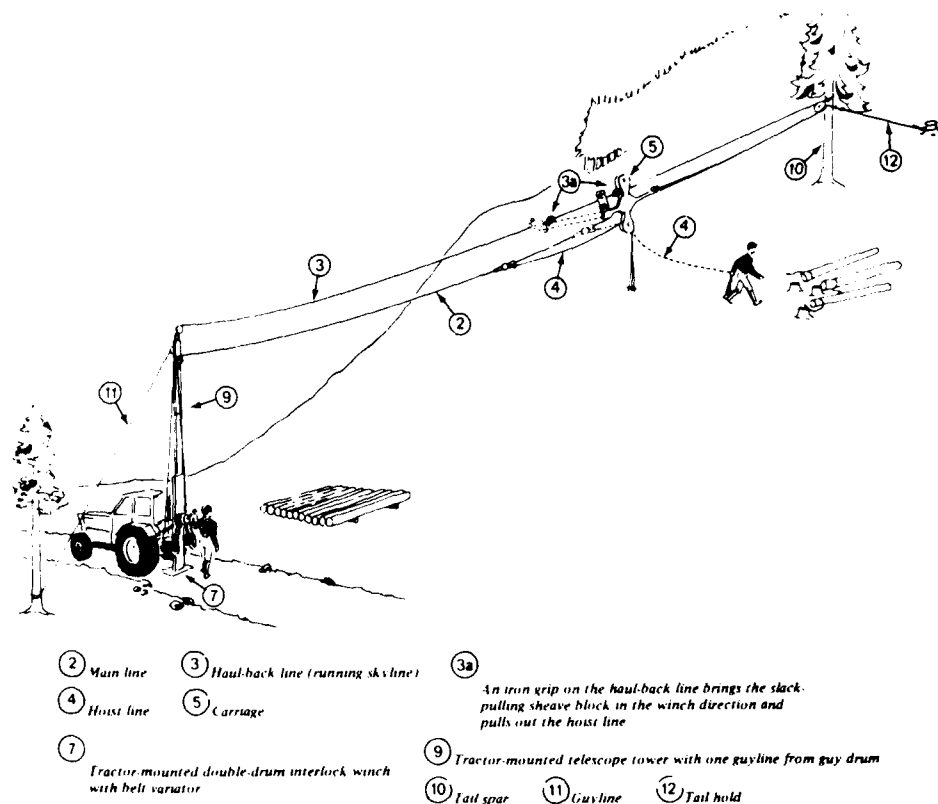
Figure 13. Cable crane yarding with the Igland Interlock winch and carriage with a slack pulling block.
