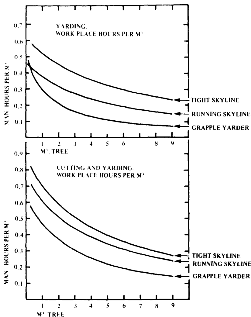
Figur 35. The average productivity in manhours per cu.m. for yarding and for cutting and yarding. The productivity is the average of 85 cable systems in Japan, Sovjet Union, Central Europe, Northern Europe, United States and British Columbia.
