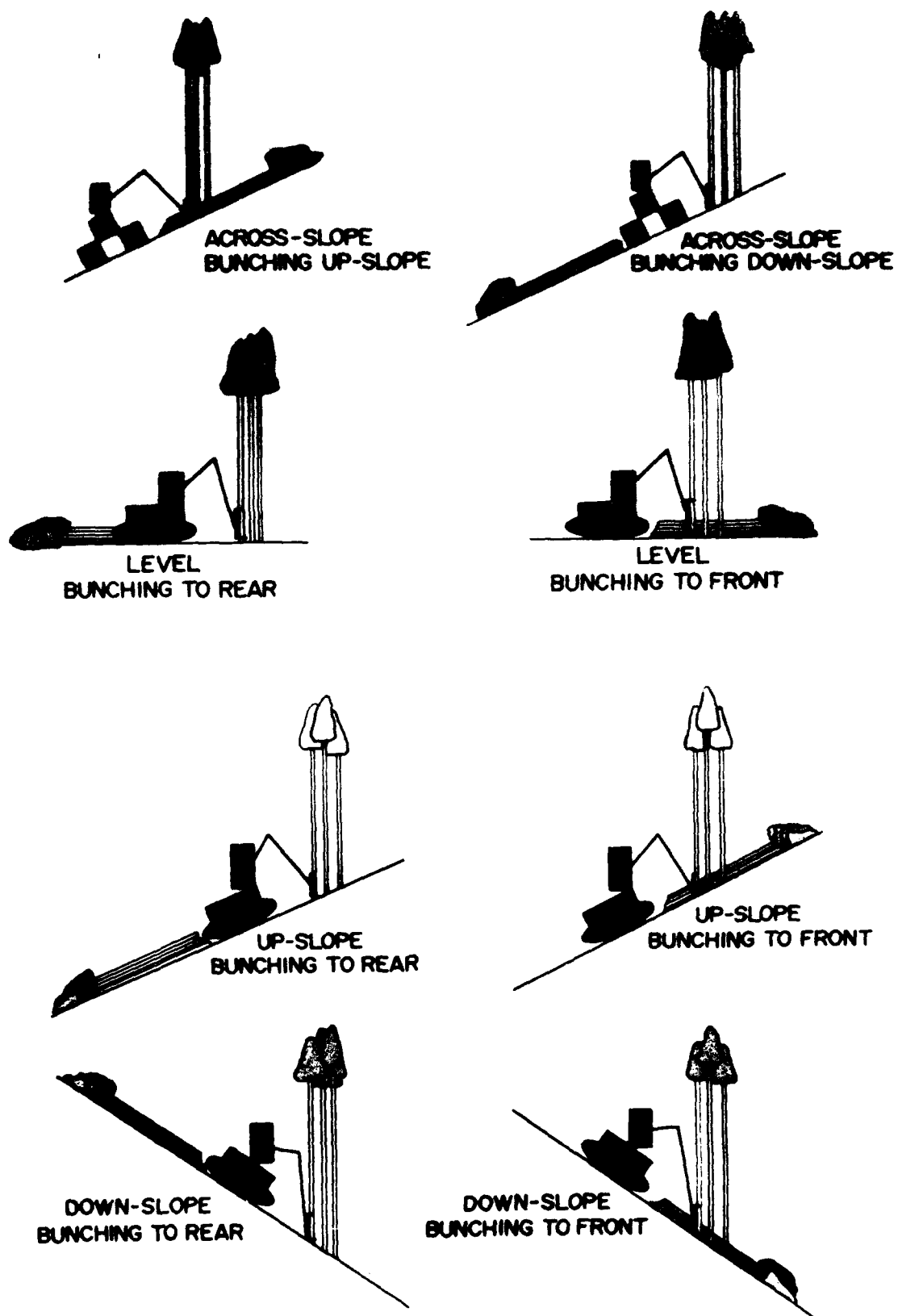
Figure 2. Felling patterns tested with Timbco Hydro-Buncher.
