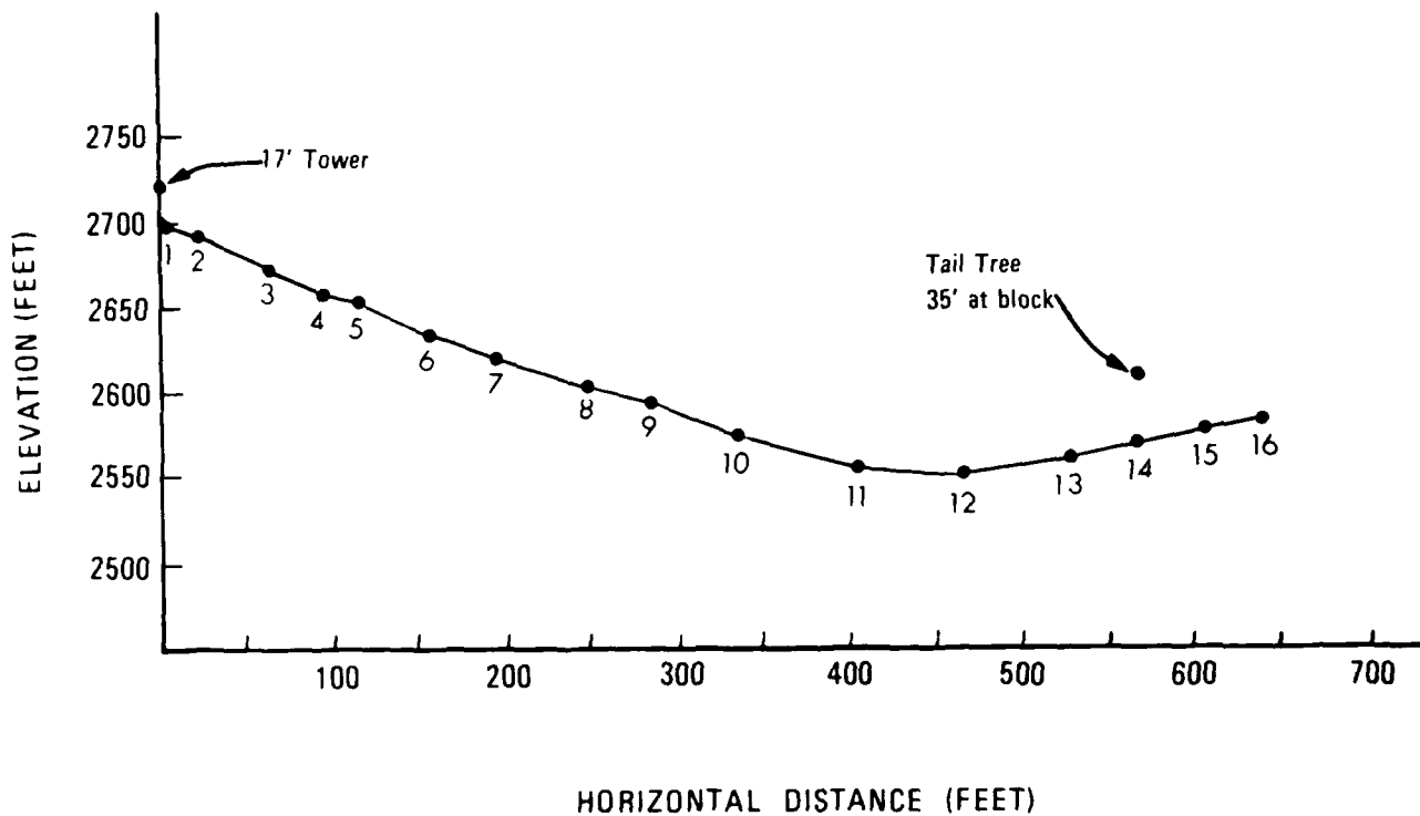
Figure 2. Logging Profile for Study of Bitterroot Miniyarder
