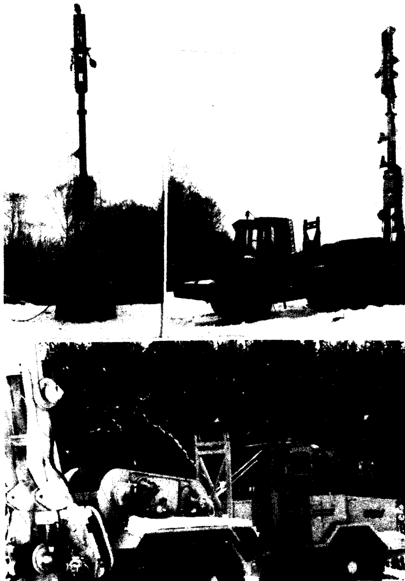
Figure 4. The Moxy yarder with Lantec 3-drum interlock winch.
