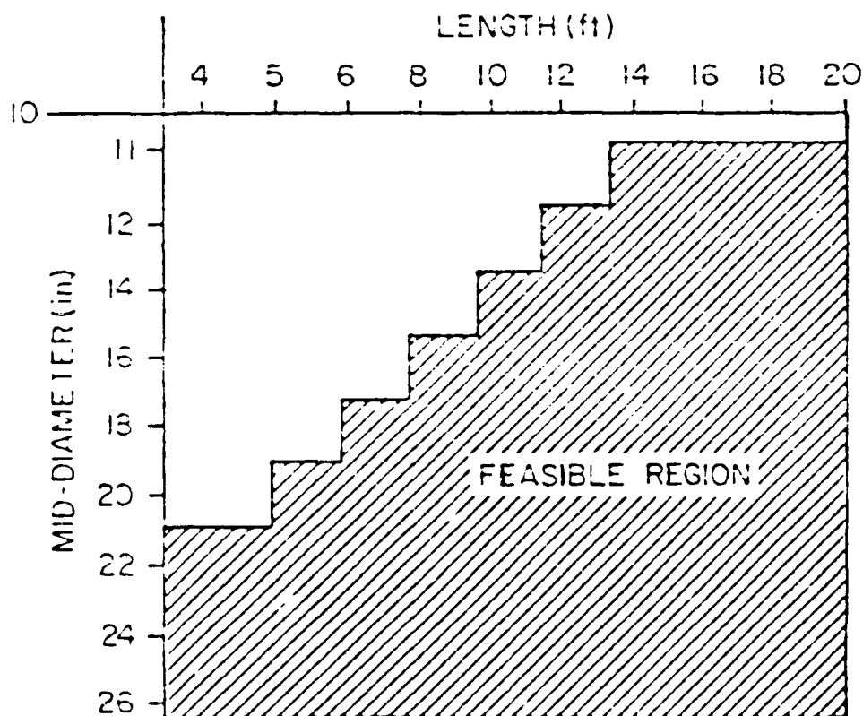
Figure 4.--Matrix of mid-diameters and lengths for residue pieces of at least 9.0 cubic feet. Piece is 9.0 cubic feet or larger if its mid-diameter and length fall on or below the stairstep line.
