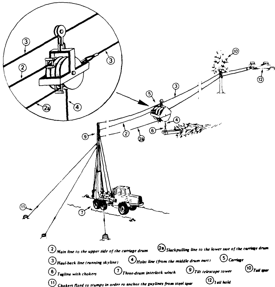
Figure 5. The Moxy cable crane with running skyline and drum carriage.
