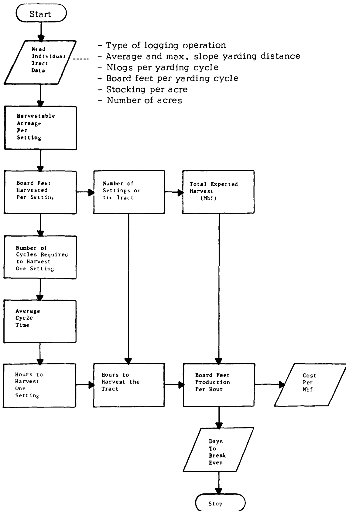
Figure 2. Flowchart of the Appalachian Thinner's Economic Model.
