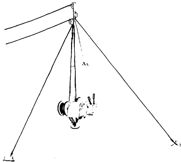
Figure 12. Igland Interlock winch with telescope tower. The farm tractor may be disconnected and moved away while the cable crane remains rigged up.
