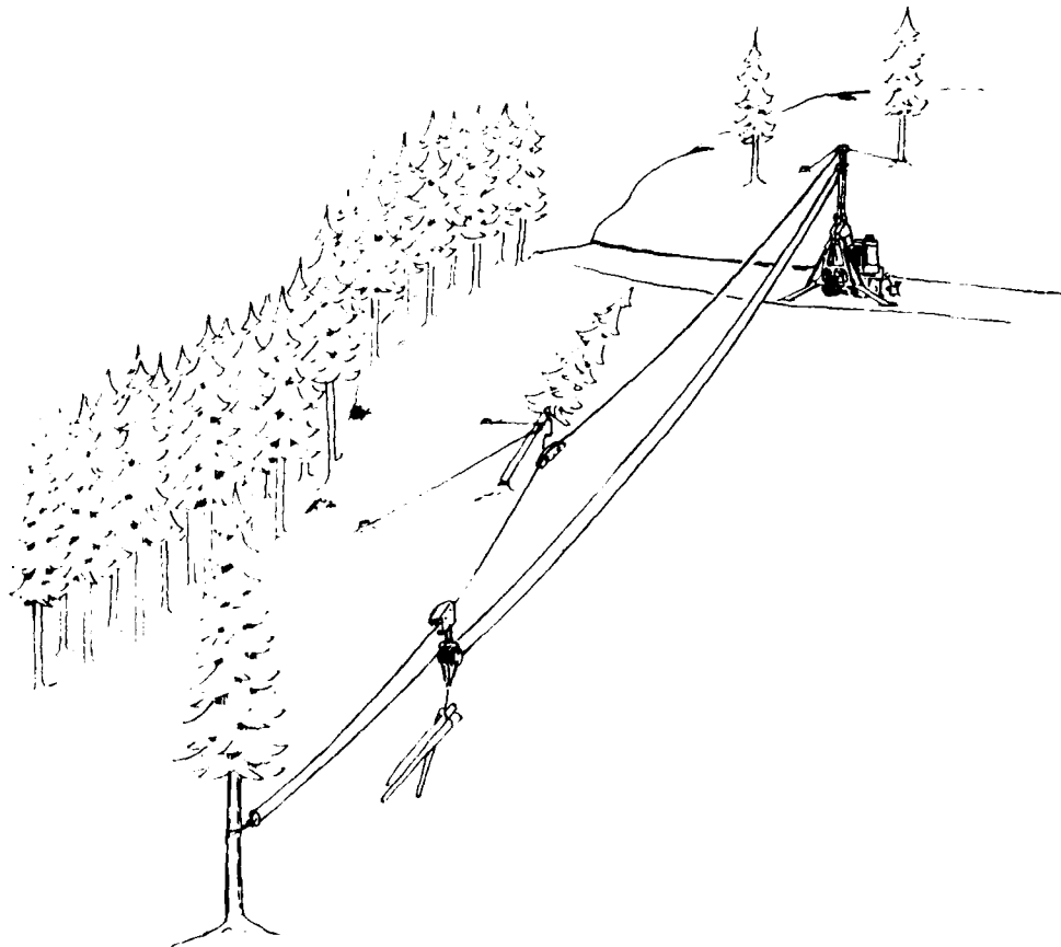
Figure 8. The Owren Vario Winch as running skyline with support on the haul-back line.
