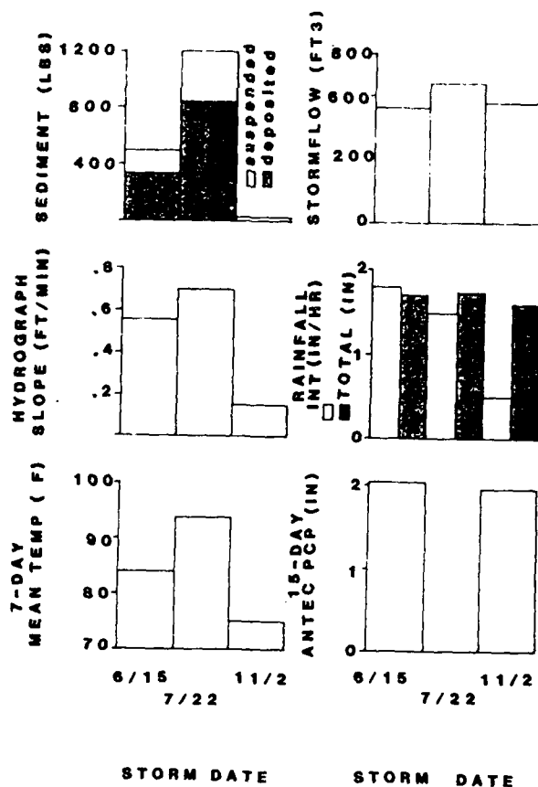
Figure 3. Comparison of storm parameters for three events on Segment 1.
