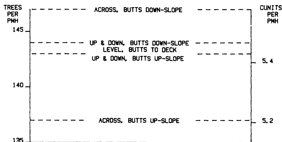
Figure 6. Production rates for combination felling patterns. (Assume: 150 residual trees/ac, 400 cut trees/ac, 6-in DBH and accumulated basal area of 0.39 sq ft)
