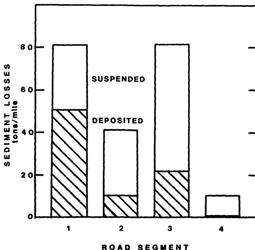
Figure 2. Suspended and deposited (cross-hatched) sediment losses (tons per mile) for the four road segments.
