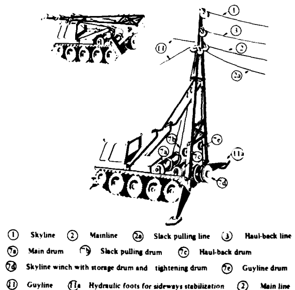
Figure 18. Owren Vario-Crane with the tilt tower rigged up and laid down.
