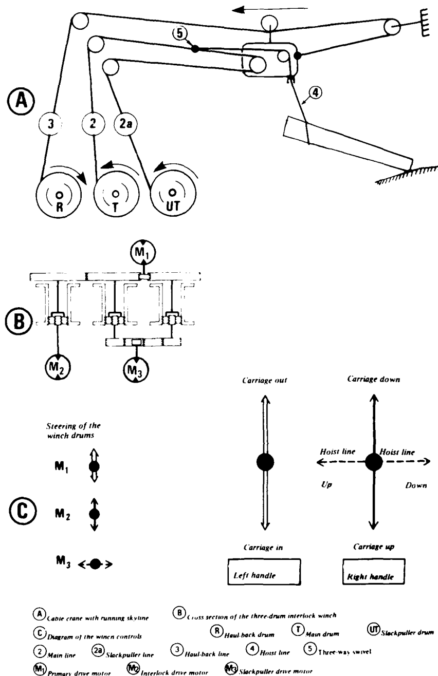
Figure 6. Cable crane with running skyline and triple-drum interlock winch.
