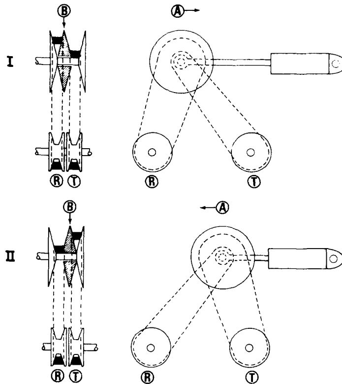
Figure 11. The belt variator in the Igland interlock winch.
