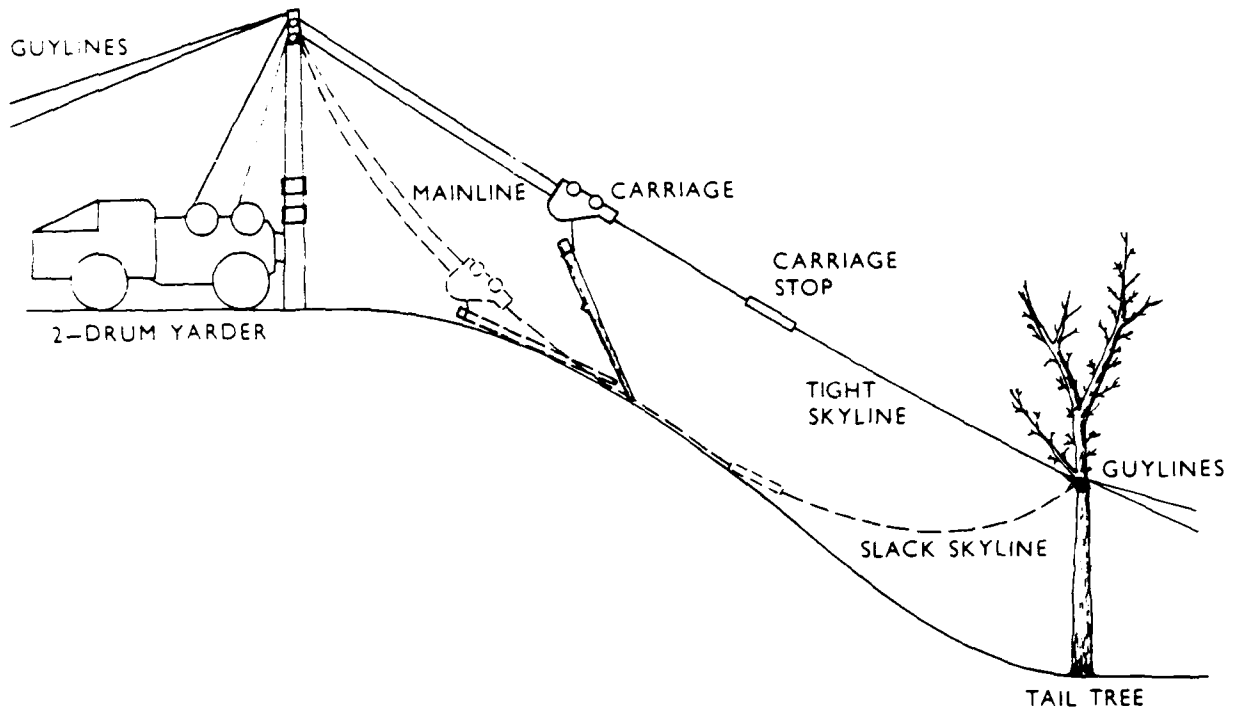
Figure 1. Typical Live Skyline Yarder Configuration
