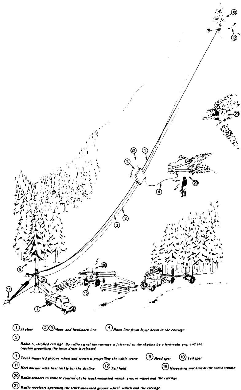
Figure 1. The Nestestog radio-controlled truck mounted cable crane and radio-controlled carriage.
