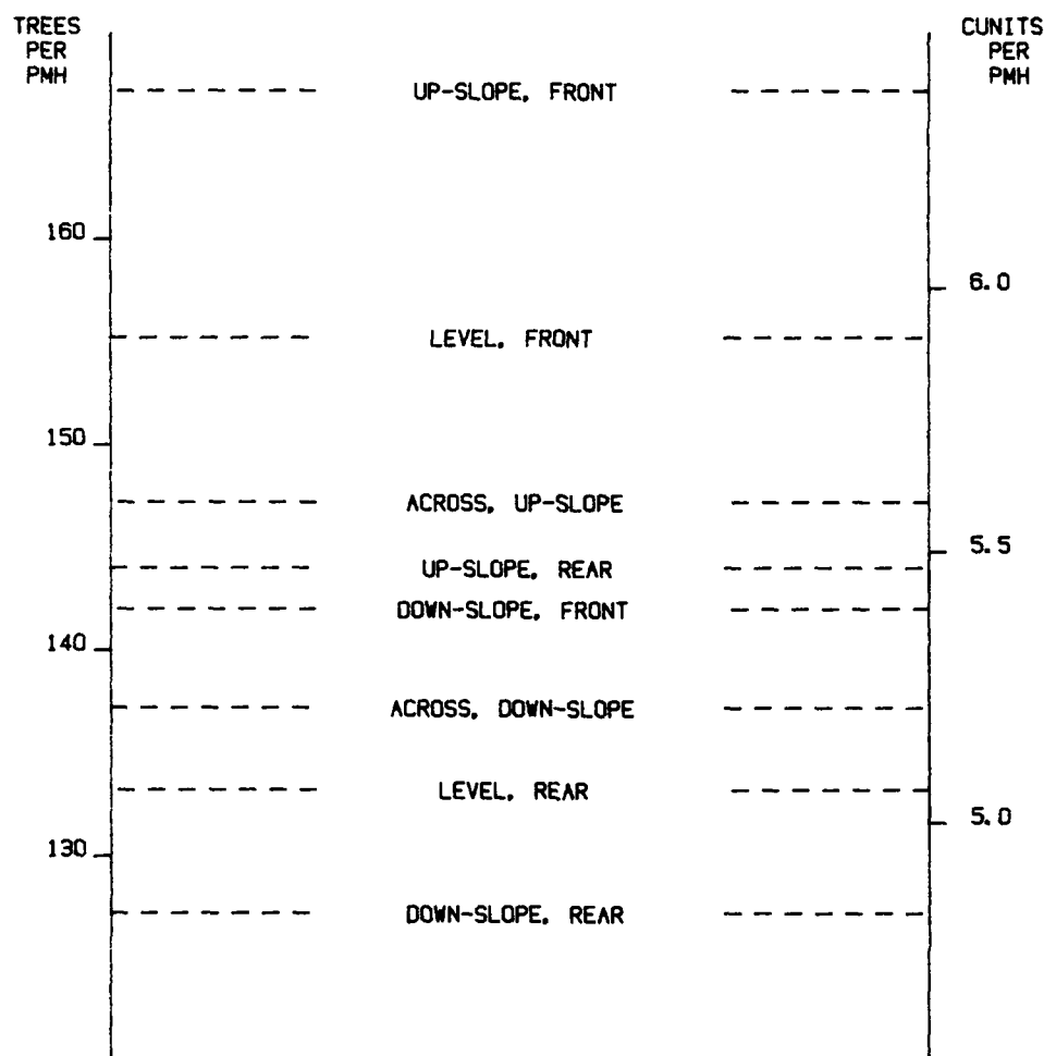
Figure 5. Production rates for felling patterns with Timbco. (Assume: 150 residual trees/ac, 400 cut trees/ac, 6-in DBH and accumulated basal area of 0.39 sq ft)
