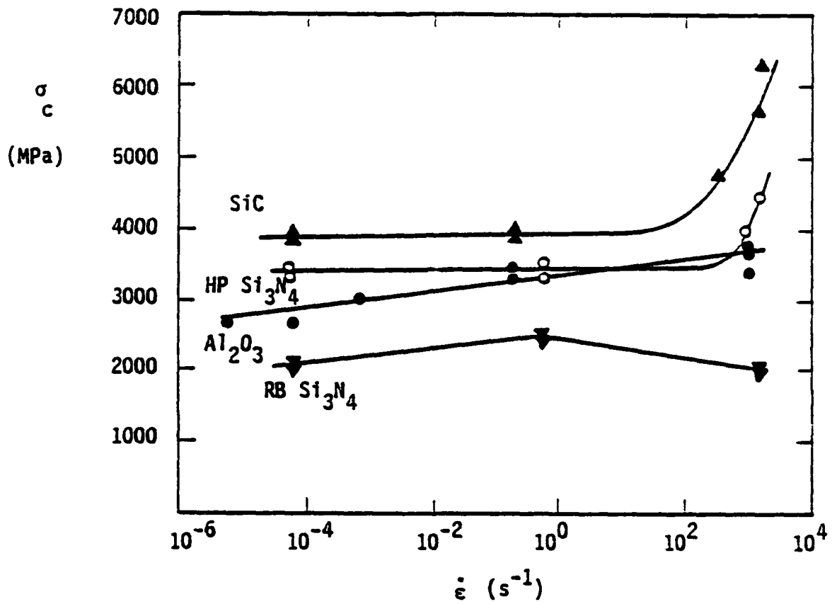
Figure 1. Compressive Strength Versus Strain Rate for Several Monolithic Ceramics at 23°C. The decrease in strength for reaction bonded (RB) Si 3 N 4 at \dot{\epsilon} \approx 10^3 \text{ s}^{-1} is caused by a transition in fracture mode from transgranular to intergranular.
