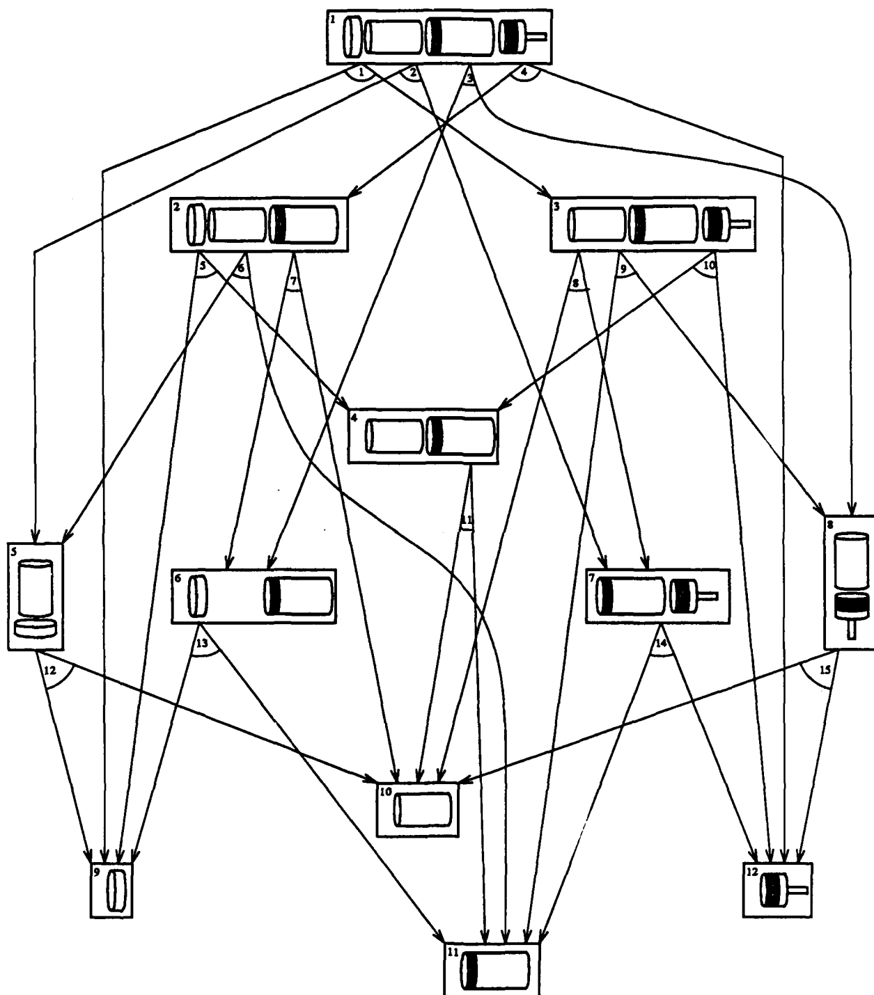
Figure 15: The AND/OR graph for the assembly shown in figure 3
