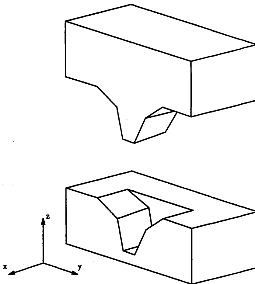
Figure 22: Two parts that have seven planar contacts
