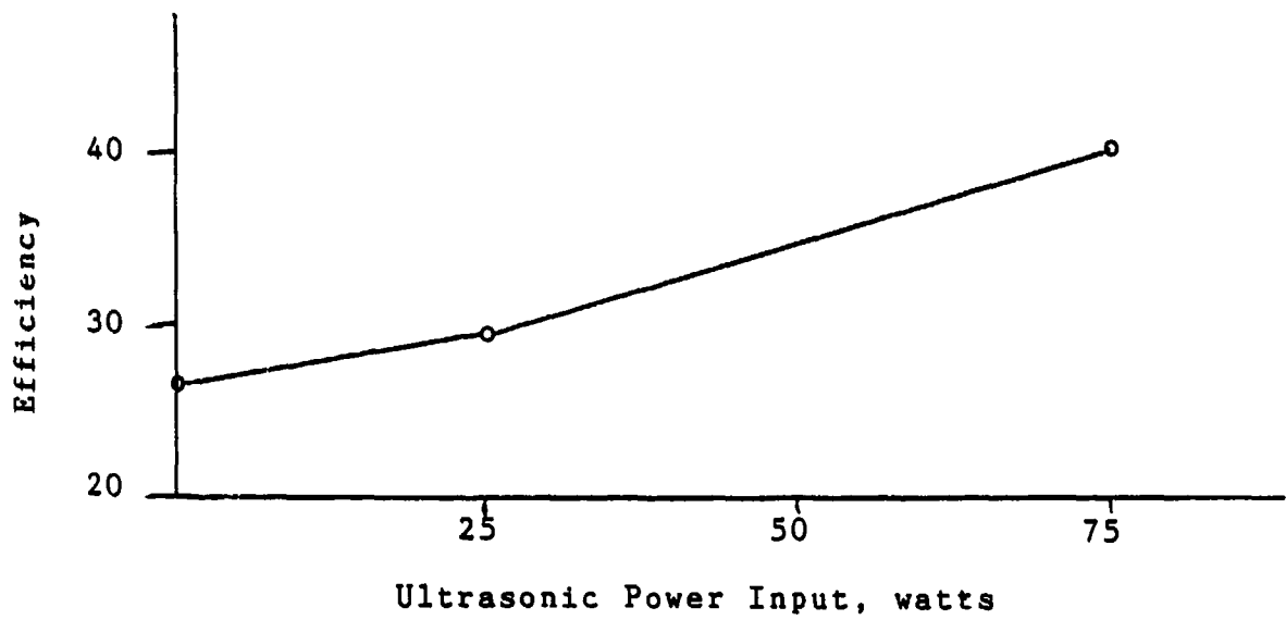
Figure 5-7. Parametric Evaluation of the Effect of Ultrasonic Power Input on Coalescence Efficiency
