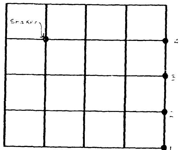
Figure 4 Forced response, accelerometer and shaker locations
