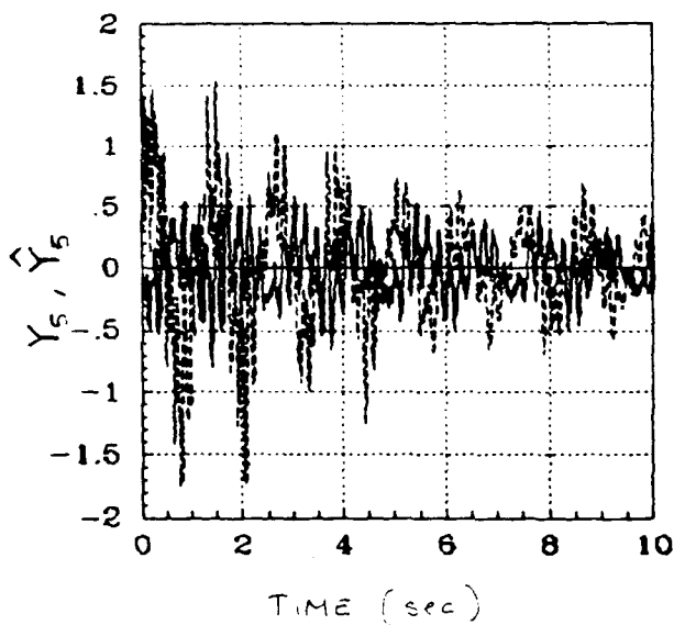
Figure 7 Y_5 and \hat{Y}_5 vs. time for grid free response
