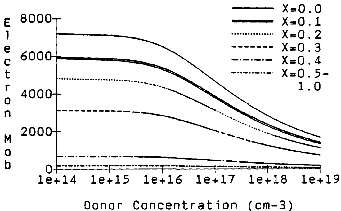
Fig. 4: Electron mobility vs donor concentration with the Al mole fraction, x as a parameter and the electric field equal to 1.0 KV/cm.
