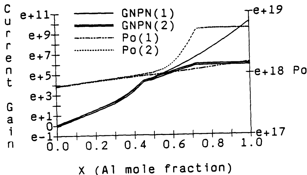
Fig. 9: Current gain ( J_{ni}/J_s ), GNPN, and inversion charge density, Po, as a function of the Al mole fraction, x. The symbol (1) indicates that the effective velocity is calculated using only the thermal velocity while (2) indicates that both the thermal velocity and the drift-diffusion velocities were used. The spike layer is in the semiconductor, V_{ce} = 2.0 and J_s = 75 .
