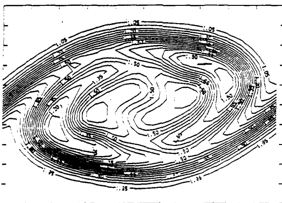
Figure 14. Temperature contours for the uniform density, non-reacting flow, T_1/T_2 = 0.5 , at t = 5 , 10, 15 and 20.
