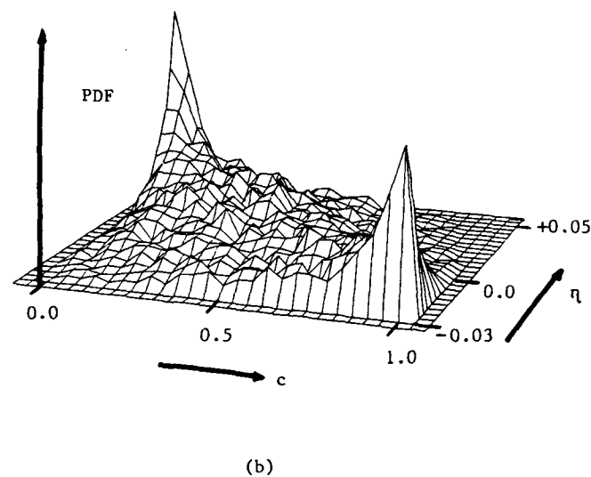
Figure 10. Probability-density function of concentration at x = 5.0 for: (a) P_e = \infty ; and (b) P_e = 2500 . \eta = (y - y_0)/(x - x_0) .
