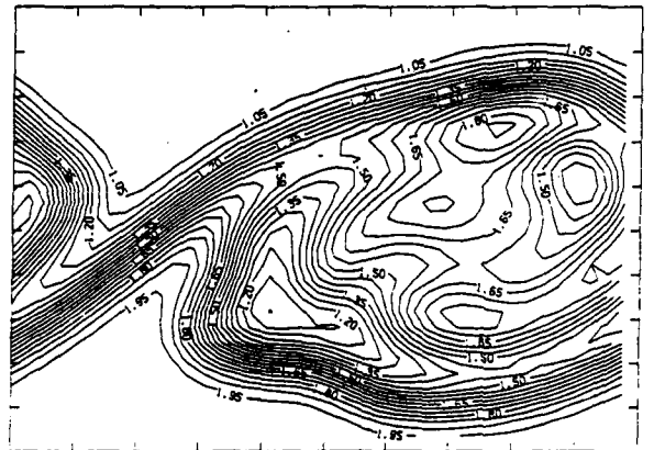
Figure 18. Temperature contours for the density-stratified, non-reacting flow, \rho_1/\rho_2 = 2.0 , at t = 10, 15 and 20 .
