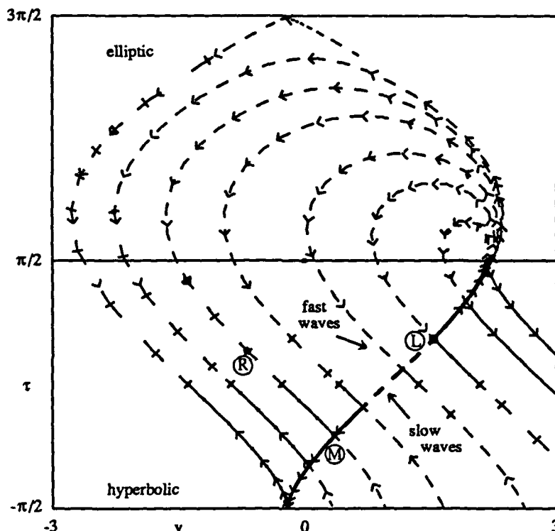
Fig. 6: The wave curve diagram for a typical U_L . Solid curves correspond to rarefaction waves, dashed curves to shock waves, and dashed curves with crossbars to composite waves. Darker curves represent the -c family, while lighter curves represent the +c family.
