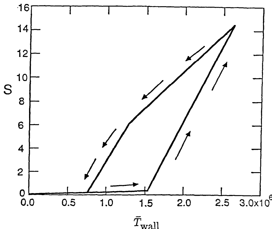
Fig. 11: Hysteresis under cyclic loading.
