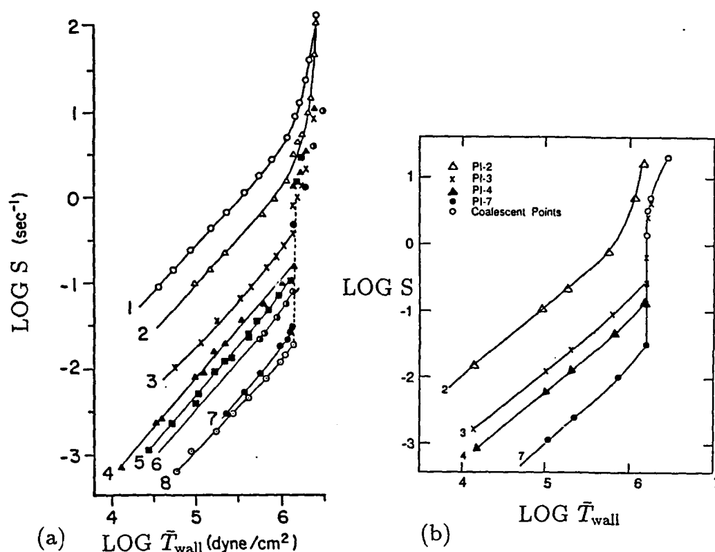
Fig. 10: Volumetric flow rate vs. effective shear stress: (a) experiment [18]; (b) numerical calculation [8]. Notice that the horizontal scale of this panel matches that of panel (a), but the vertical scale does not.
